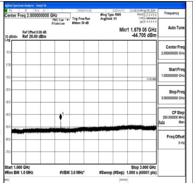
Band26_10MHz_QPSK_26990_1RB#0_1000~3000_1000~3000
