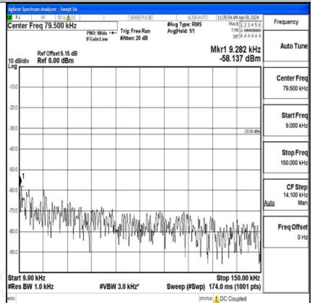
Band26_15MHz_16QAM_26915_1RB#0_0.009~0.15_0.009~0.15
