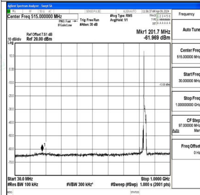
Band26_15MHz_QPSK_26965_1RB#0_30~1000_30~100 0
