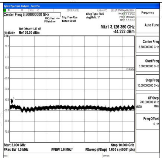
Band26_10MHz_16QAM_26915_1RB#0_3000~10000_300 0~10000
