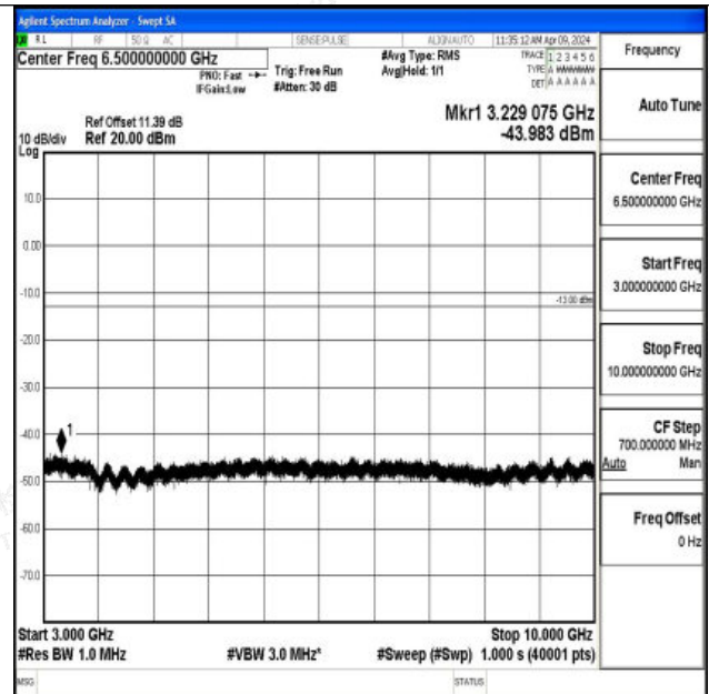
Band26_15MHz_16QAM_26865_1RB#0_3000~10000_300 0~10000
