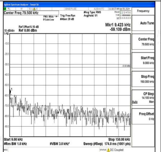
Band26_10MHz_16QAM_26990_1RB#0_0.009~0.15_0.009~0.15
