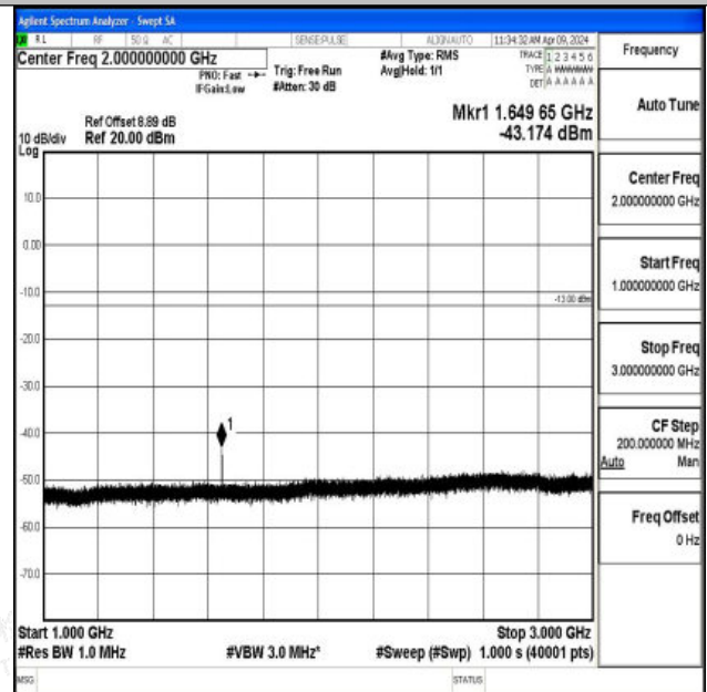
Band26_15MHz_QPSK_26865_1RB#0_1000~3000_1000~3000
