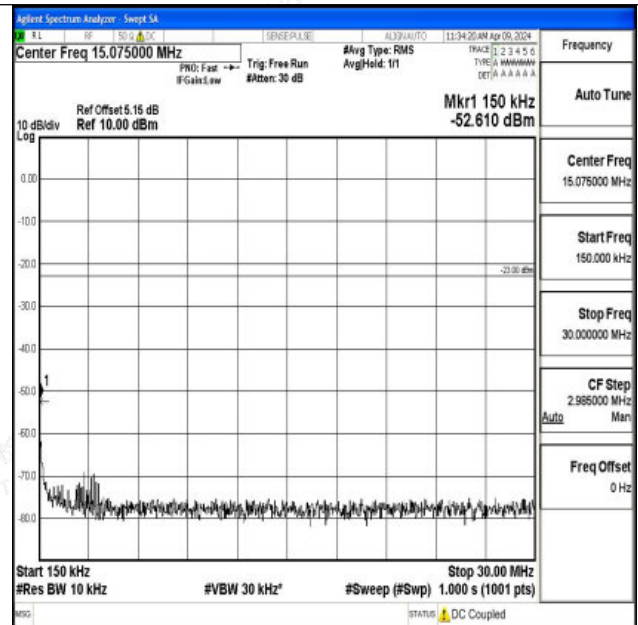
Band26_15MHz_QPSK_26865_1RB#0_0.15~30_0.15~30
