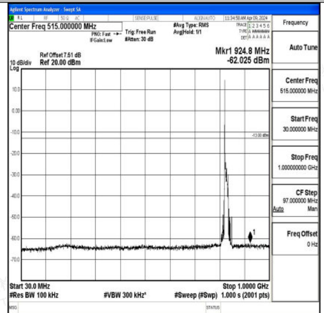
Band26_15MHz_16QAM_26865_1RB#0_30~1000_30~100 0
