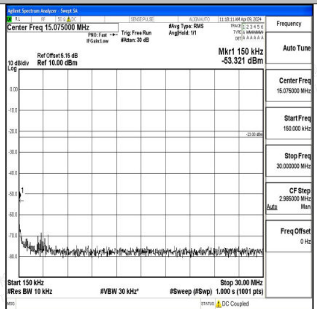
Band26_10MHz_QPSK_26990_1RB#0_0.15~30_0.15~30
