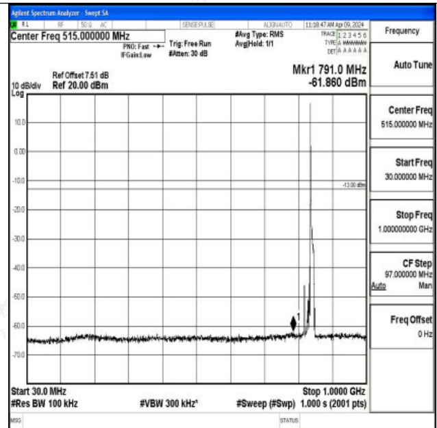
Band26_10MHz_16QAM_26990_1RB#0_30~1000_30~100
