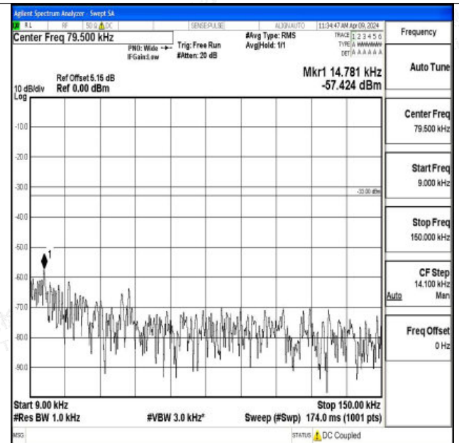
Band26_15MHz_16QAM_26865_1RB#0_0.009~0.15_0.009 ~0.15
