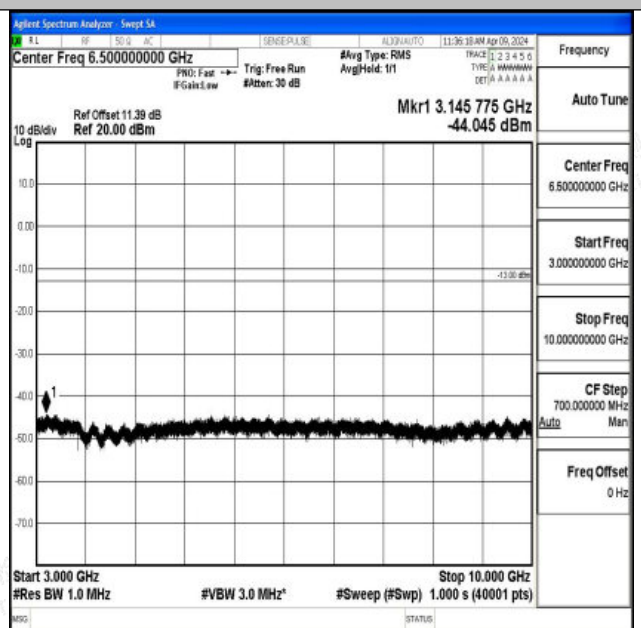
Band26_15MHz_16QAM_26915_1RB#0_3000~10000_300
