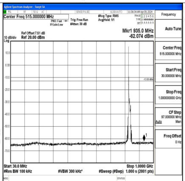
Band26_15MHz_16QAM_26915_1RB#0_30~1000_30~100
