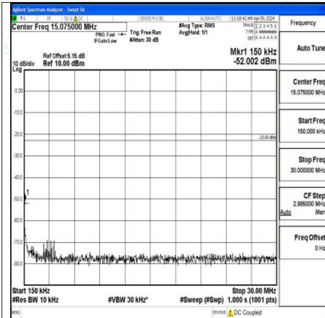
Band26_10MHz_16QAM_26990_1RB#0_0.15~30_0.15~3
