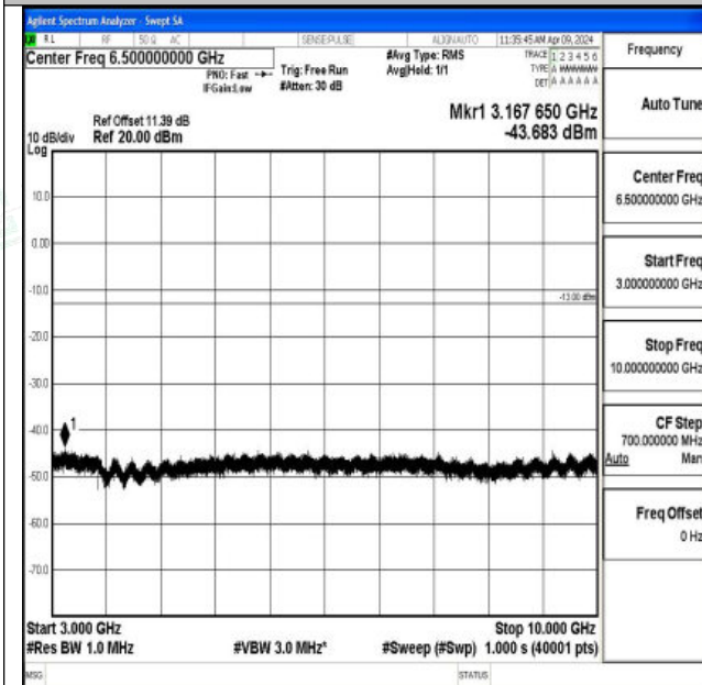
Band26_15MHz_QPSK_26915_1RB#0_3000~10000_3000~10000
