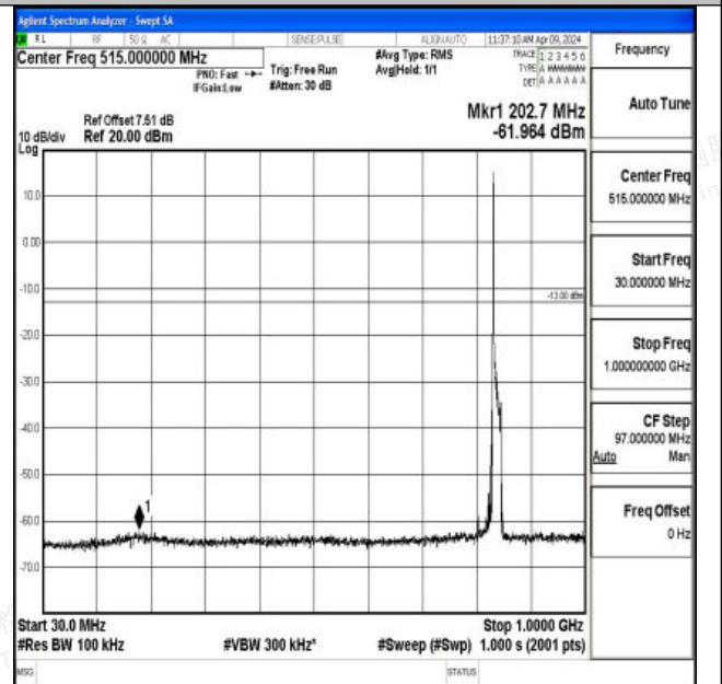
Band26_15MHz_16QAM_26965_1RB#0_30~1000_30~100 0
