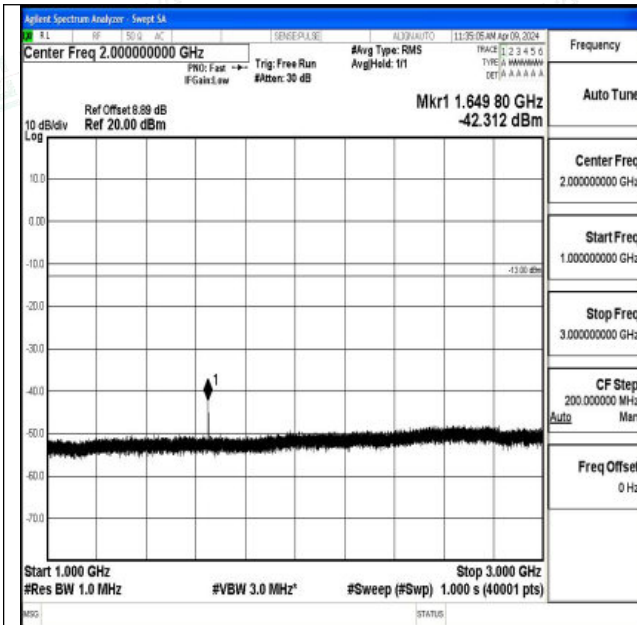
Band26_15MHz_16QAM_26865_1RB#0_1000~3000_100 0~3000
