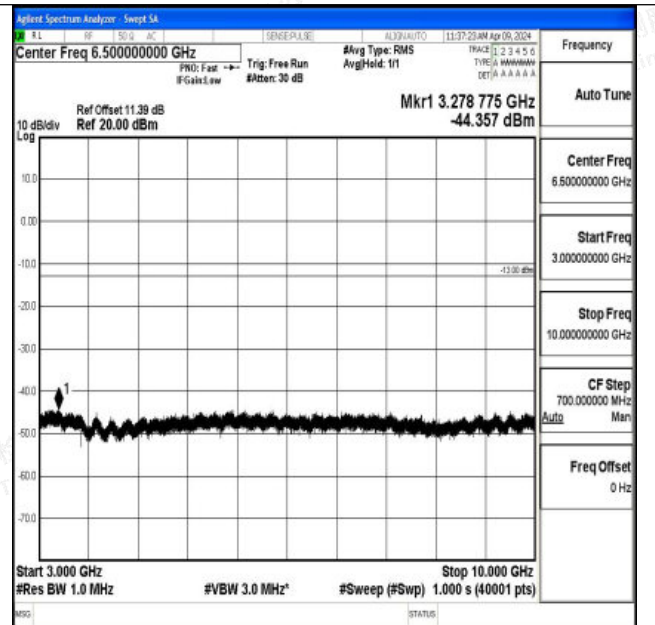
Band26_15MHz_16QAM_26965_1RB#0_3000~10000_300 0~10000
