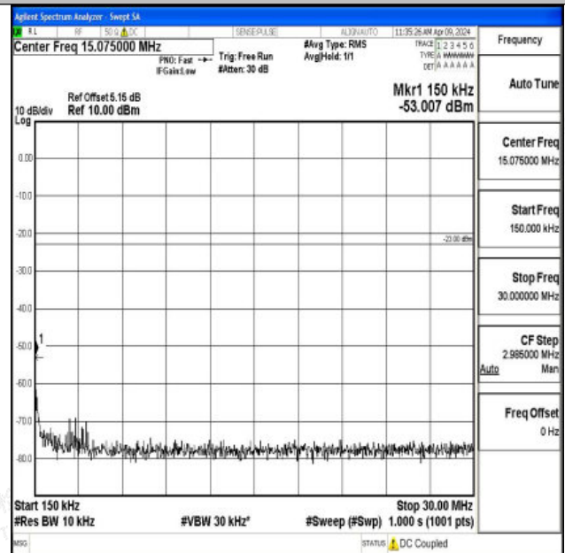
Band26_15MHz_QPSK_26915_1RB#0_0.15~30_0.15~30
