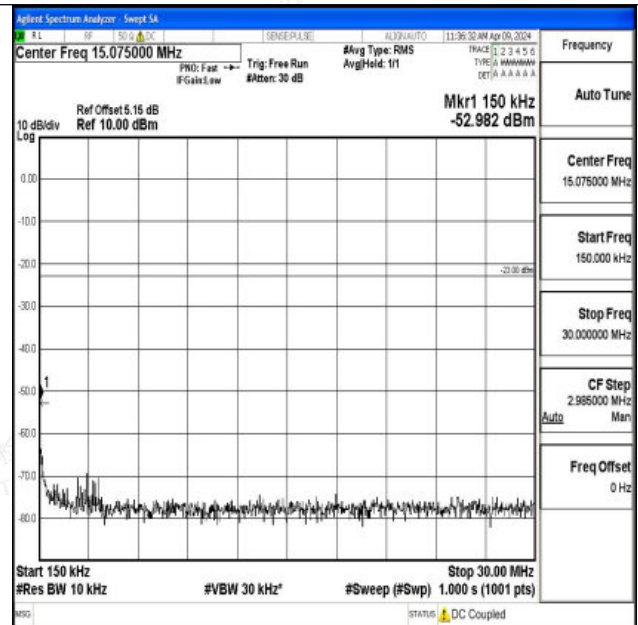
Band26_15MHz_QPSK_26965_1RB#0_0.15~30_0.15~30
