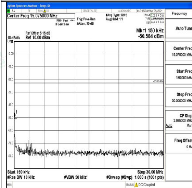
Band26_15MHz_16QAM_26865_1RB#0_0.15~30_0.15~3 0
