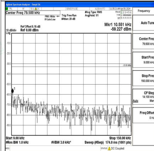
Band26_15MHz_QPSK_26915_1RB#0_0.009~0.15_0.009 ~0.15
