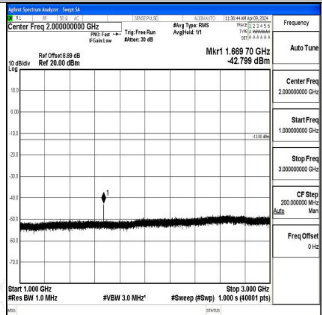
Band26_15MHz_QPSK_26965_1RB#0_1000~3000_1000~ 3000
