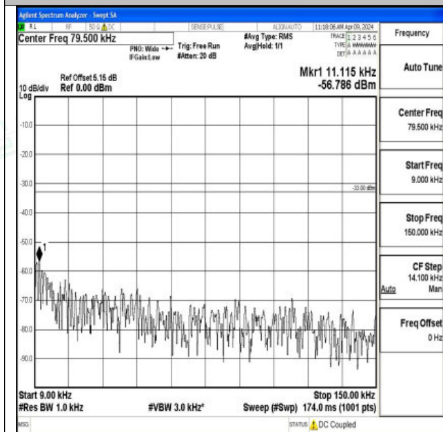
Band26_10MHz_QPSK_26990_1RB#0_0.009~0.15_0.009 ~0.15
