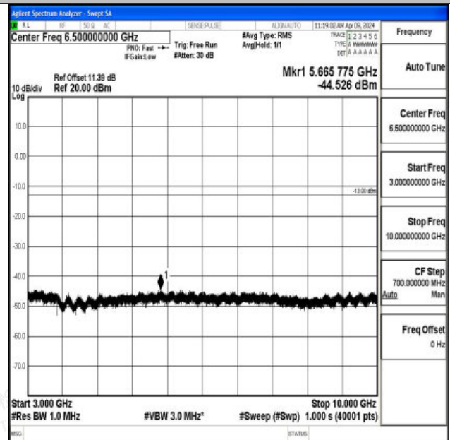
Band26_10MHz_16QAM_26990_1RB#0_3000~10000_300
