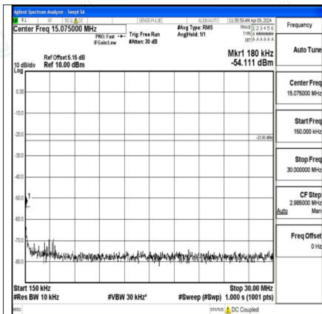
Band26_15MHz_16QAM_26915_1RB#0_0.15~30_0.15~3
