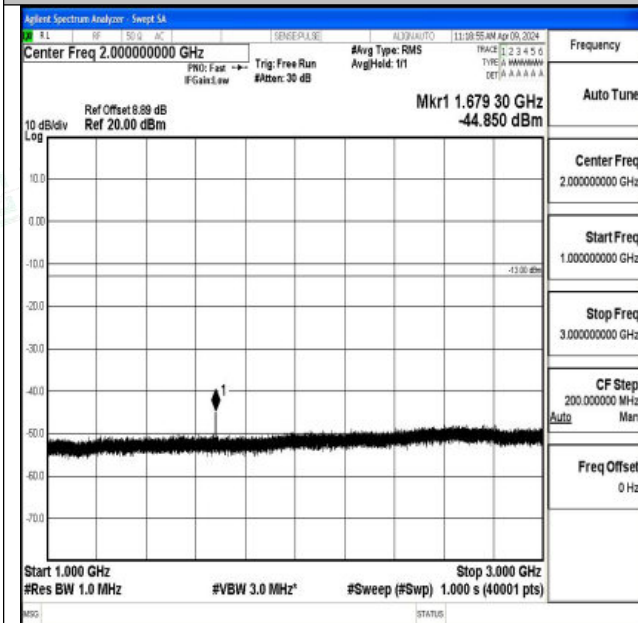
Band26_10MHz_16QAM_26990_1RB#0_1000~3000_100
