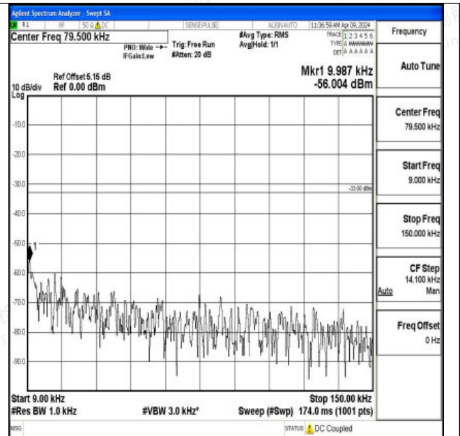
Band26_15MHz_16QAM_26965_1RB#0_0.009~0.15_0.009 ~0.15
