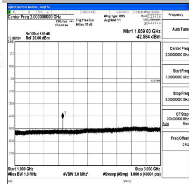
Band26_15MHz_16QAM_26915_1RB#0_1000~3000_100
