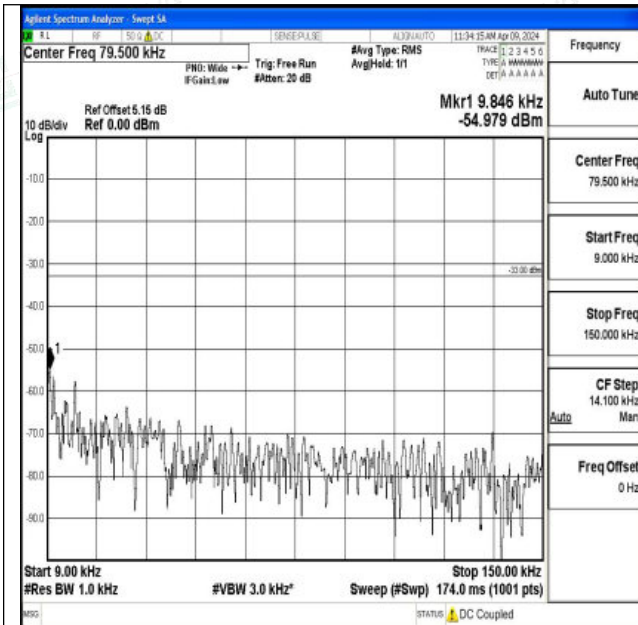
Band26_15MHz_QPSK_26865_1RB#0_0.009~0.15_0.009~0.15
