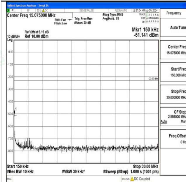
Band26_15MHz_16QAM_26965_1RB#0_0.15~30_0.15~3 0
