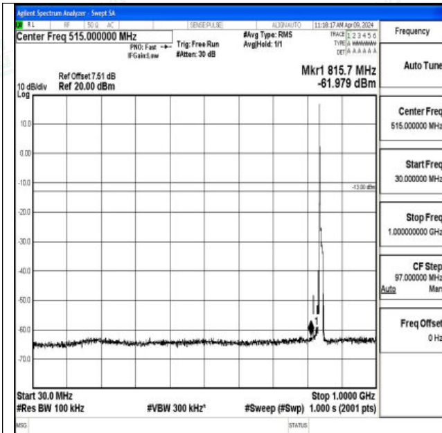
Band26_10MHz_QPSK_26990_1RB#0_30~1000_30~100
