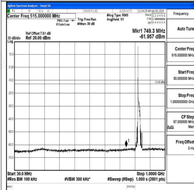
Band26_15MHz_QPSK_26865_1RB#0_30~1000_30~1000
