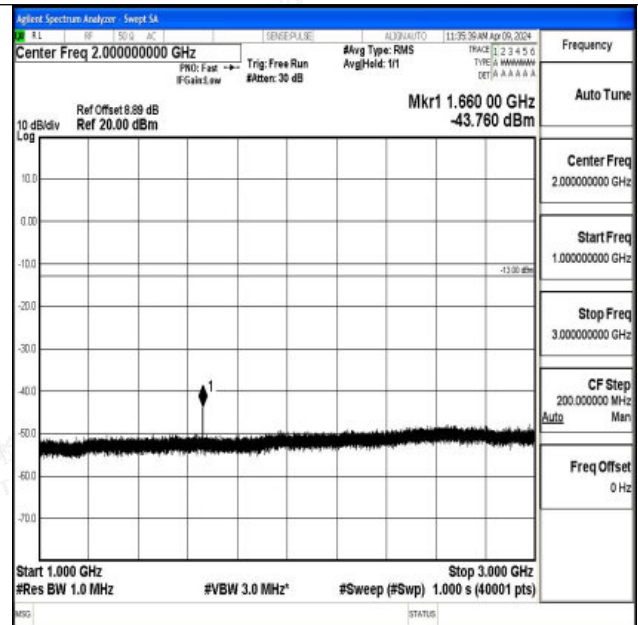
Band26_15MHz_QPSK_26915_1RB#0_1000~3000_1000~3000
