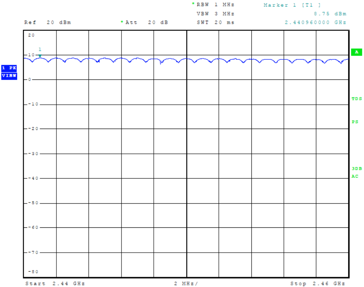
Figure 6 Plot of Number of Hopping Channels Mode 2, BT BR GFSK
