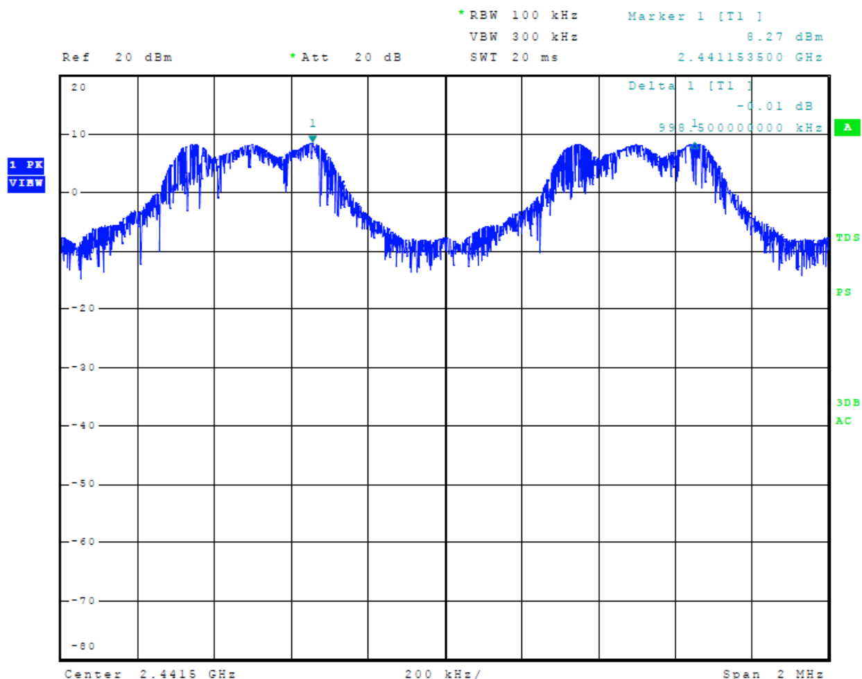
Figure 8 Plot of Channel Separation Mode 2, BT BR GFSK
