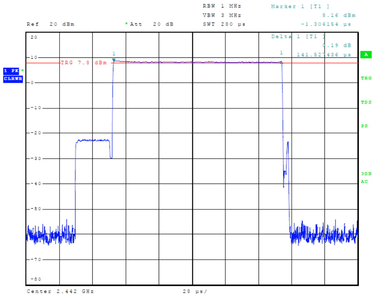
Figure 9 Plot of Dwell time On Channel Mode 2, BT BR GFSK
