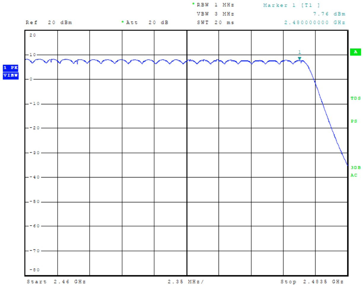
Figure 7 Plot of Number of Hopping Channels Mode 2, BT BR GFSK
