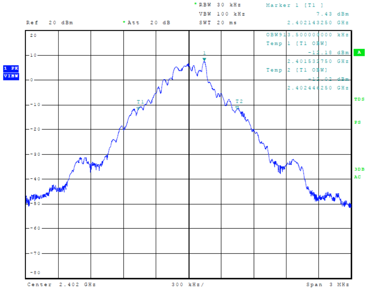
Figure 3 Plot of Transmitter Emissions 99% Occupied Bandwidth Mode 2, BT BR GFSK
