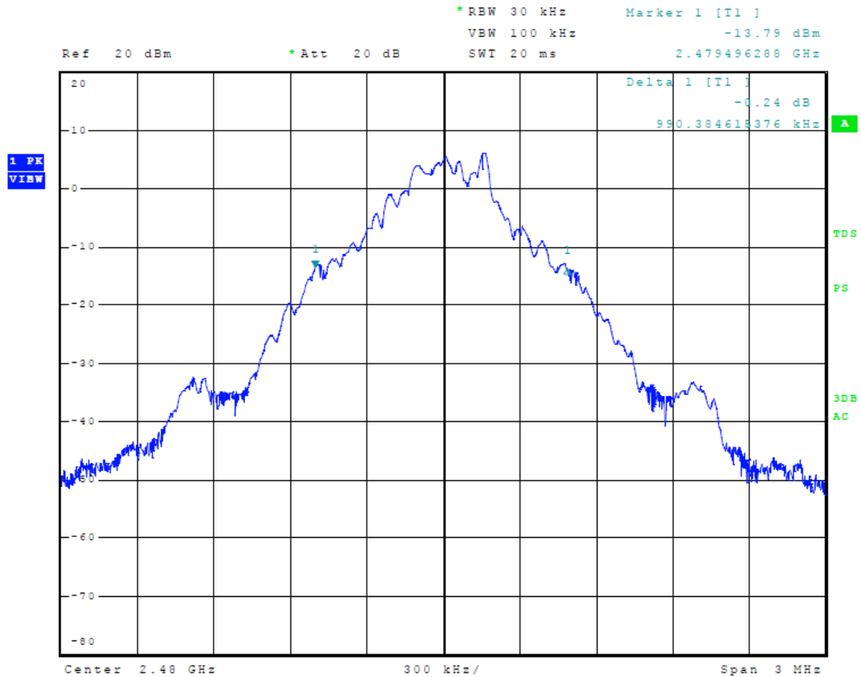
Figure 2 Plot of Transmitter Emissions 20-dB Occupied Bandwidth Mode 2, BT BR GFSK
