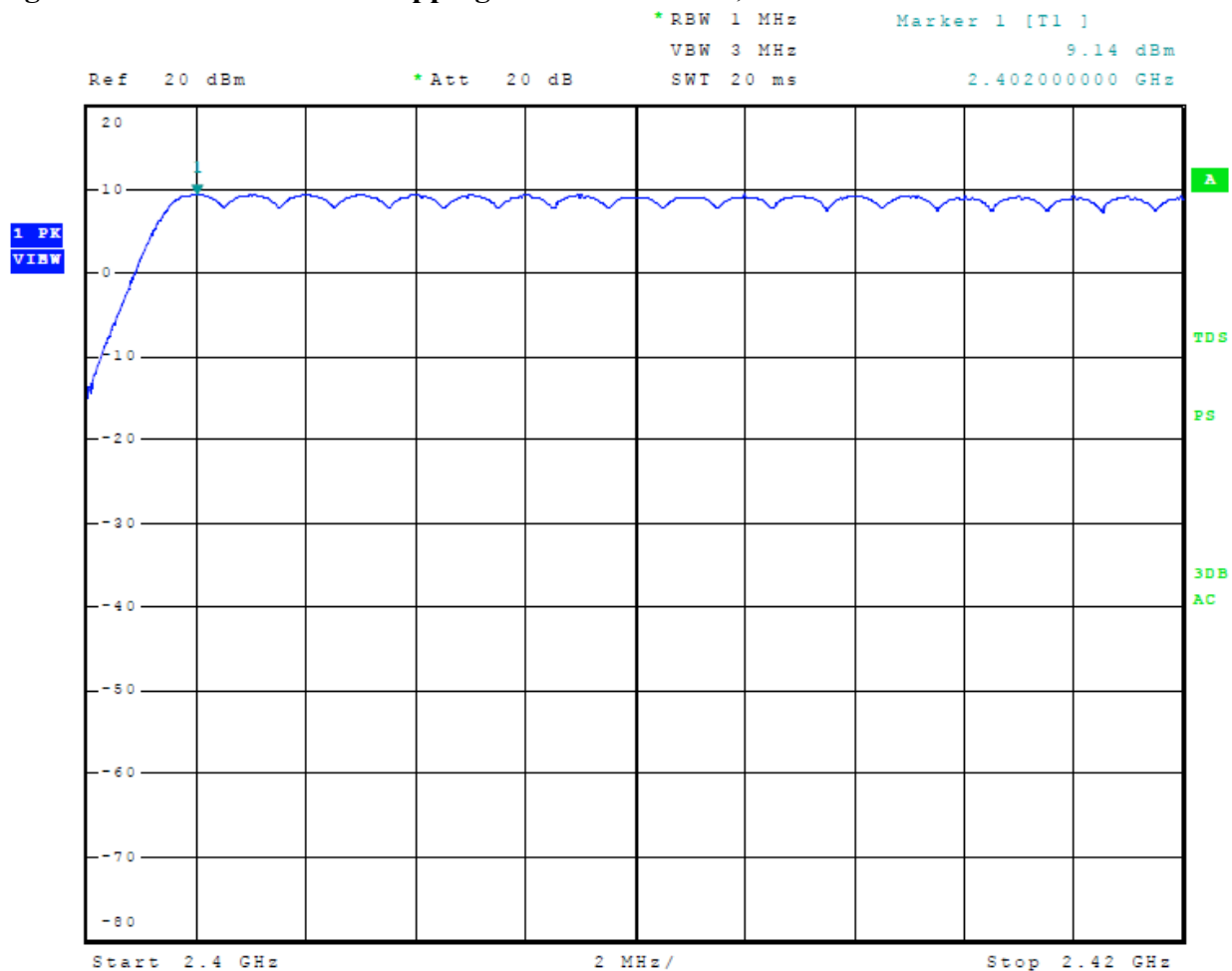
Figure 4 Plot of Number of Hopping Channels Mode 2, BT BR GFSK
