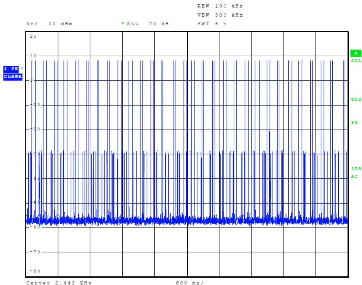
Figure 10 Plot of Number of Times on Channel over 6 Second Period Mode 2, BT BR GFSK
