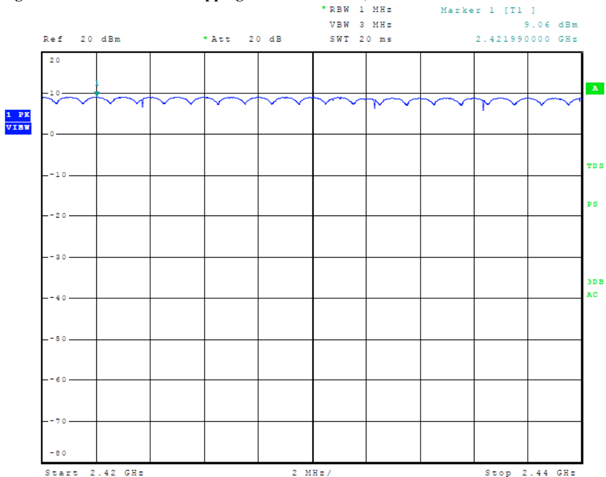
Figure 5 Plot of Number of Hopping Channels Mode 2, BT BR GFSK
