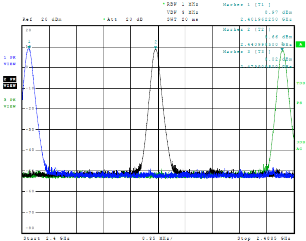
Figure 1 Plot of Transmitter Emissions Operation in 2402-2480 MHz Mode 2, BT BR GFSK
