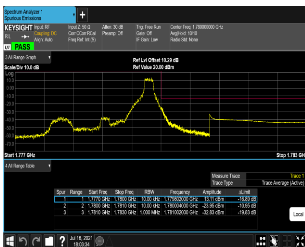
Band66-1.4MHz-QPSK-132665-1RB#5
