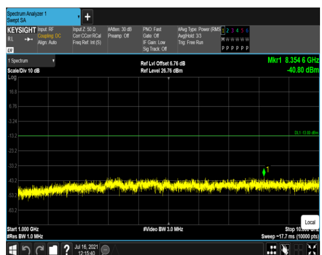
Band5-1.4MHz-QPSK-20643:1000~10000MHz
