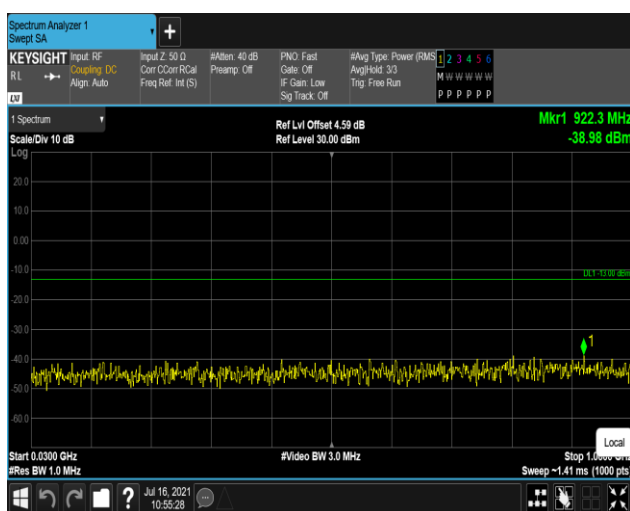
Band2-20MHz-16QAM-19100:30~1000MHz
