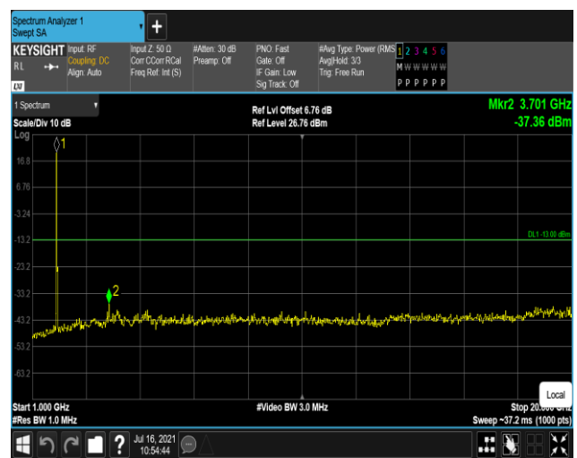
Band2-20MHz-16QAM-18900:1000~20000MHz
