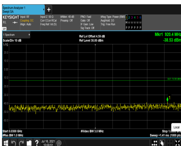
Band2-1.4MHz-16QAM-19193:30~1000MHz
