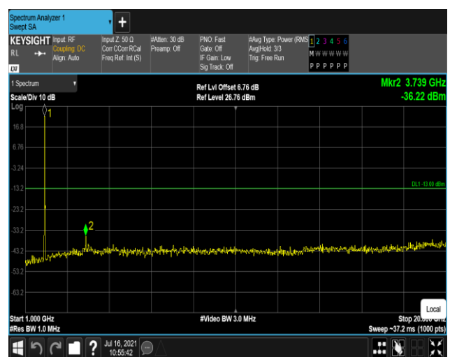
Band2-20MHz-16QAM-19100:1000~20000MHz
