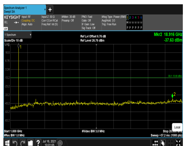
Band2-1.4MHz-16QAM-19193:1000~20000MHz
