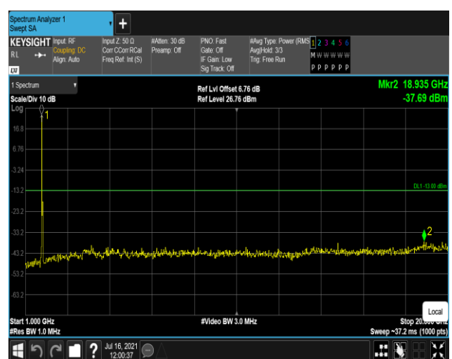
Band4-20MHz-QPSK-20300:1000~20000MHz
