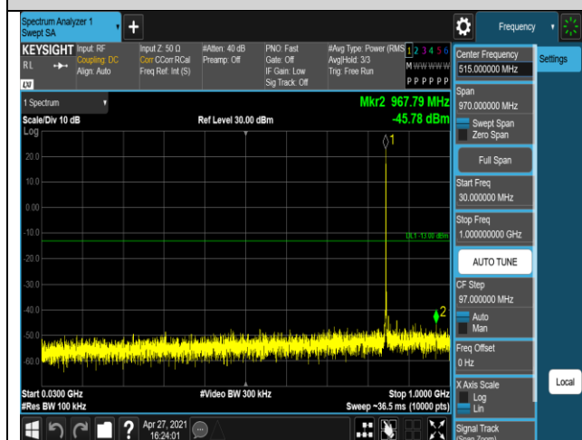
Band5-1.4MHz-16QAM-20407-1RB#0-Range1:30~1
