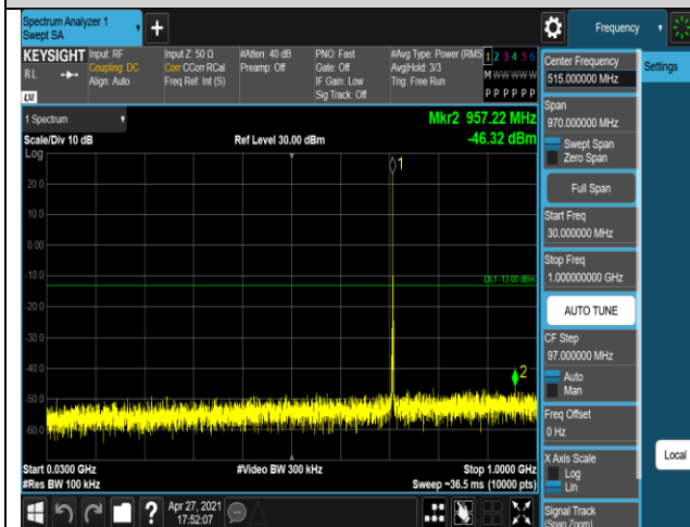
Band12-10MHz-QPSK-23060-1RB#0-Range1:30~1000MHz
