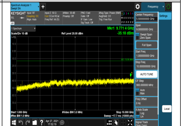
Band12-10MHz-QPSK-23060-1RB#0-Range2:1000~10000MHz
