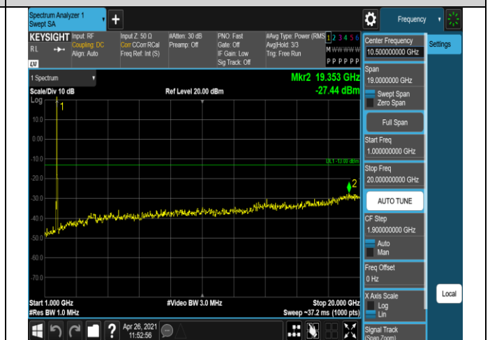
Band5-1.4MHz-QPSK-20407-1RB#0-Range2:1000~10
