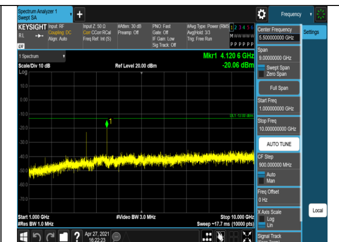
Band5-1.4MHz-QPSK-20525-1RB#0-Range2:1000~10
