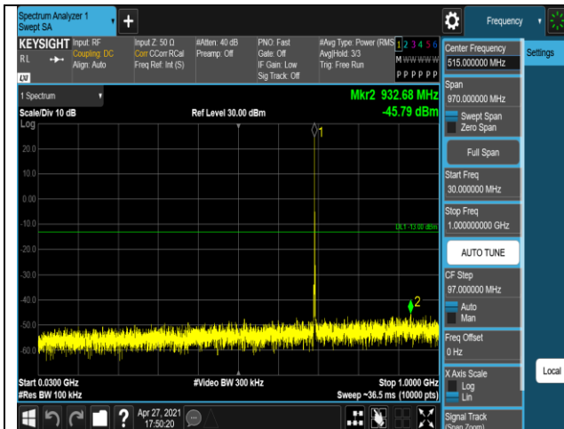
Band12-1.4MHz-16QAM-23095-1RB#0-Range1:30~1000MHz
