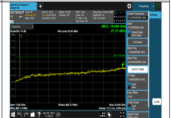
Band4-20MHz-16QAM-20300-1RB#0-Range2:1000~20
