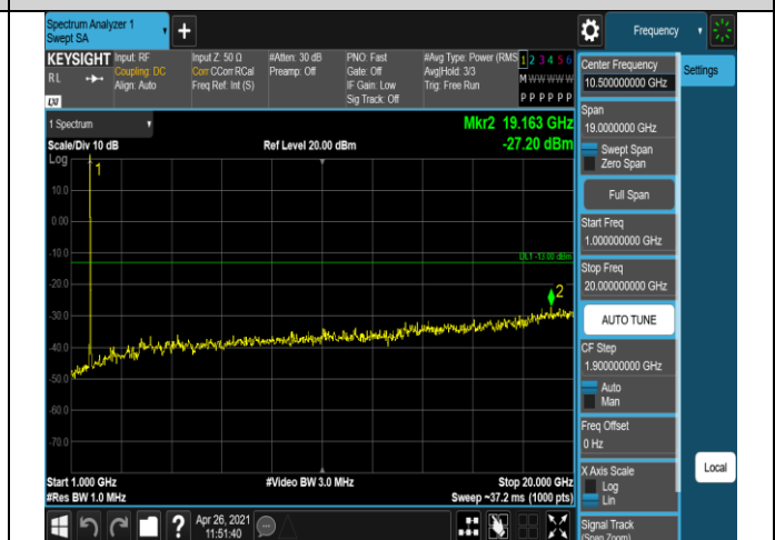
Band4-20MHz-QPSK-20300-1RB#0-Range2:1000~200
