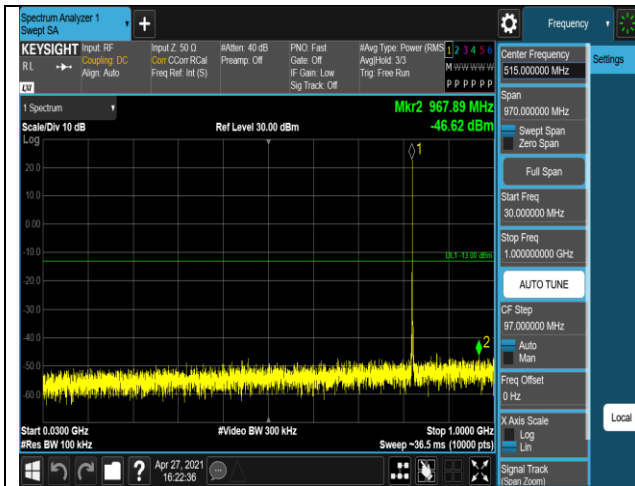
Band5-1.4MHz-16QAM-20525-1RB#0-Range1:30~1 000MHz
