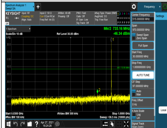
Band5-10MHz-QPSK-20450-1RB#0-Range1:30~10 00MHz
