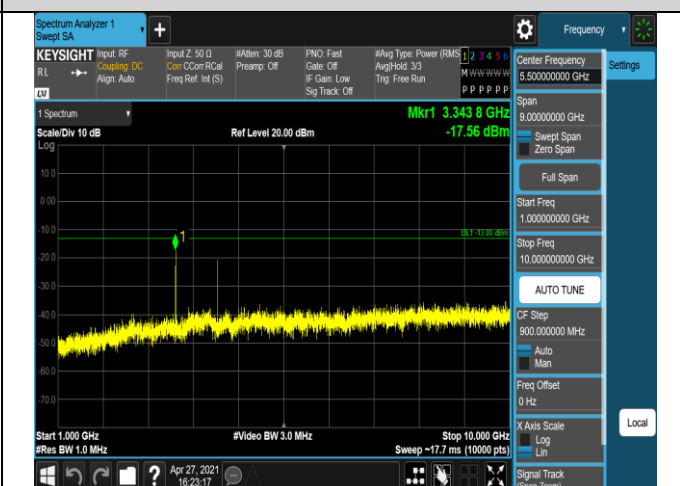
Band5-1.4MHz-QPSK-20643-1RB#0-Range2:1000~10
