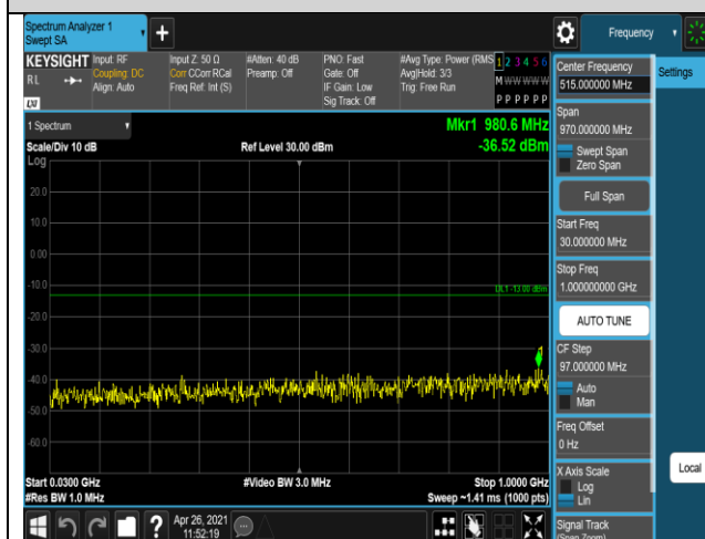
Band4-20MHz-16QAM-20050-1RB#0-Range1:30~1
