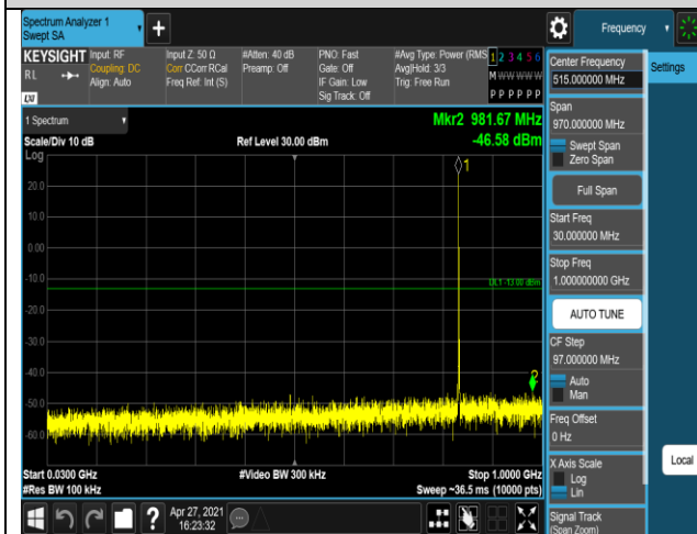
Band5-1.4MHz-16QAM-20643-1RB#0-Range1:30~1 000MHz
