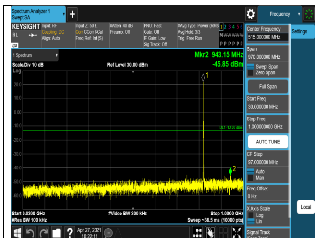
Band5-1.4MHz-QPSK-20525-1RB#0-Range1:30~10
