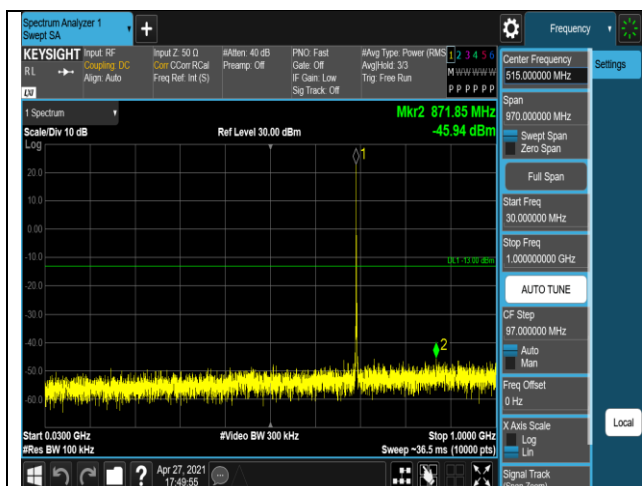
Band12-1.4MHz-QPSK-23095-1RB#0-Range1:30~1 000MHz
