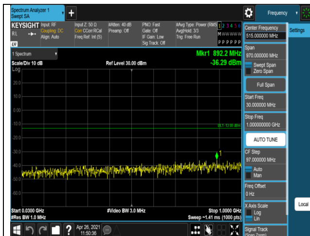
Band4-20MHz-QPSK-20175-1RB#0-Range1:30~10
