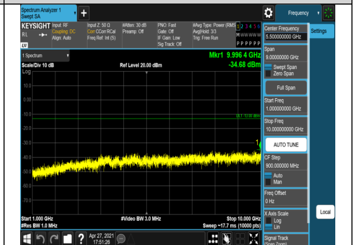
Band12-1.4MHz-16QAM-23173-1RB#0-Range2:1000~10000MHz
