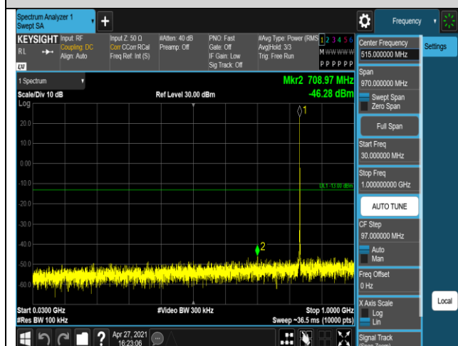
Band5-1.4MHz-QPSK-20643-1RB#0-Range1:30~10
