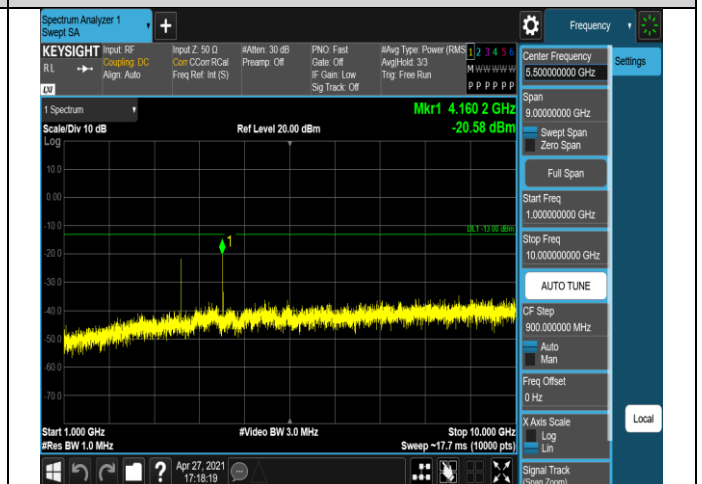
Band5-10MHz-16QAM-20600-1RB#0-Range2:1000~10
