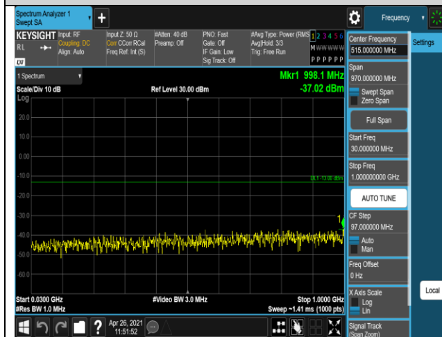
Band4-20MHz-16QAM-20300-1RB#0-Range1:30~1
