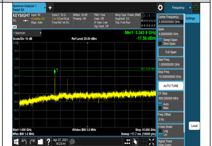
Band5-1.4MHz-16QAM-20643-1RB#0-Range2:1000~1 0000MHz
