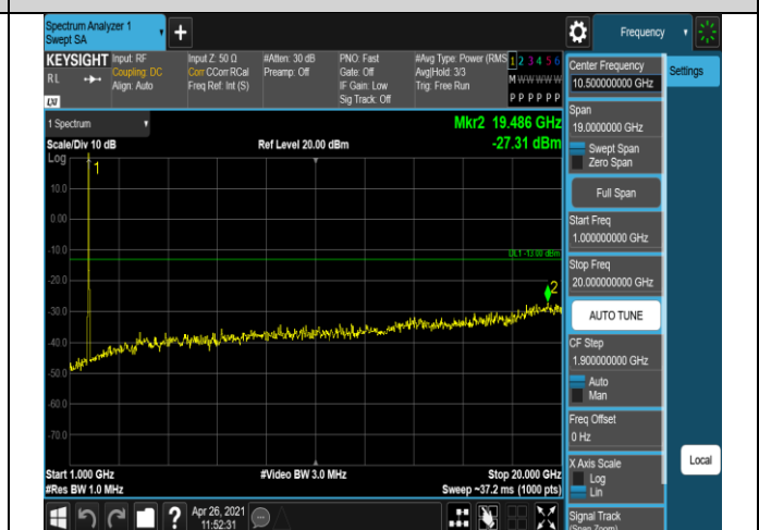
Band4-20MHz-16QAM-20050-1RB#0-Range2:1000~20
