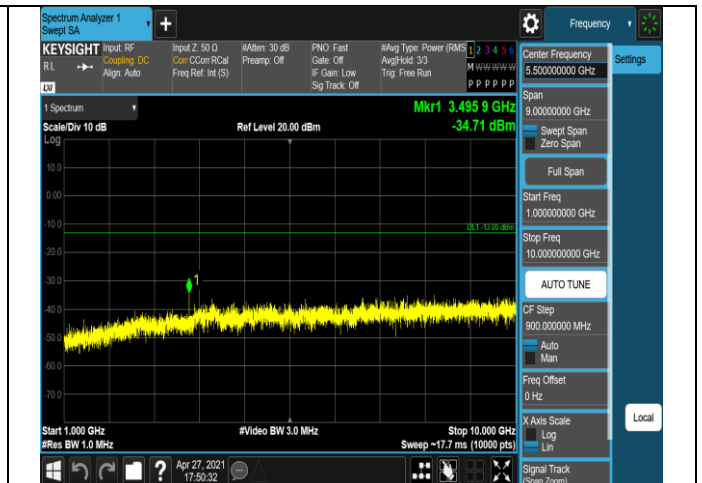
Band12-1.4MHz-16QAM-23095-1RB#0-Range2:1000~10000MHz
