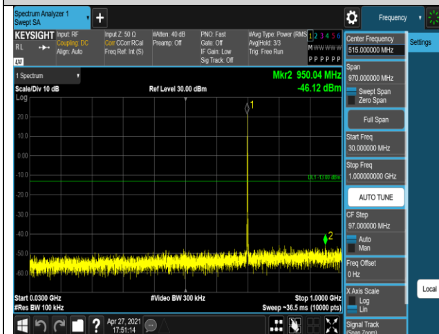
Band12-1.4MHz-16QAM-23173-1RB#0-Range1:30~1000MHz
