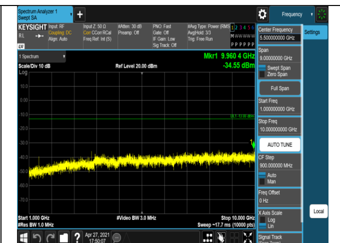
Band12-1.4MHz-QPSK-23095-1RB#0-Range2:1000~1 0000MHz
