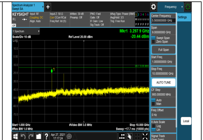
Band5-10MHz-16QAM-20525-1RB#0-Range2:1000~10
