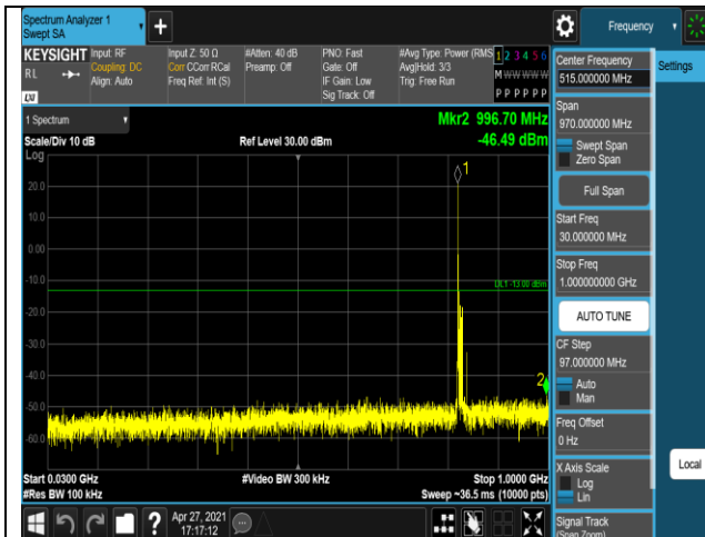
Band5-10MHz-16QAM-20525-1RB#0-Range1:30~1
