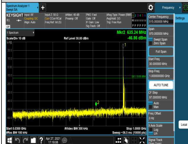
Band5-10MHz-16QAM-20600-1RB#0-Range1:30~1
