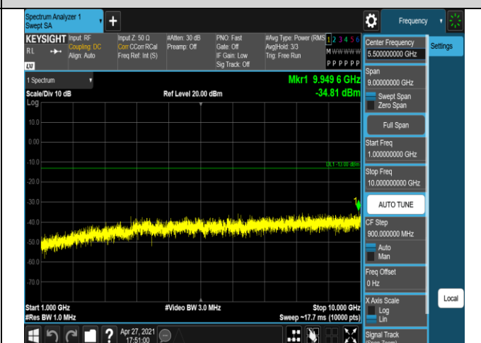
Band12-1.4MHz-QPSK-23173-1RB#0-Range2:1000~1 0000MHz
