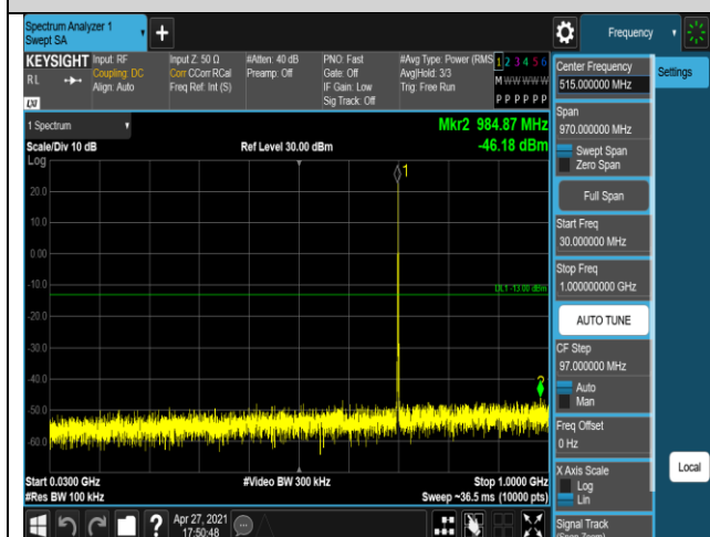
Band12-1.4MHz-QPSK-23173-1RB#0-Range1:30~1 000MHz
