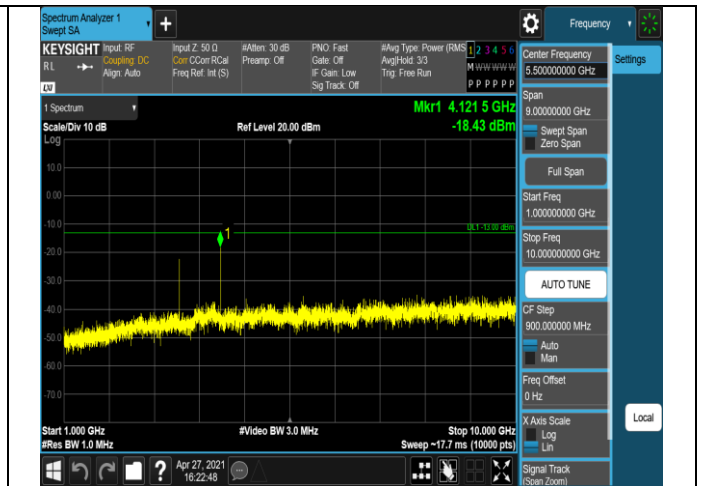
Band5-1.4MHz-16QAM-20525-1RB#0-Range2:1000~1 0000MHz
