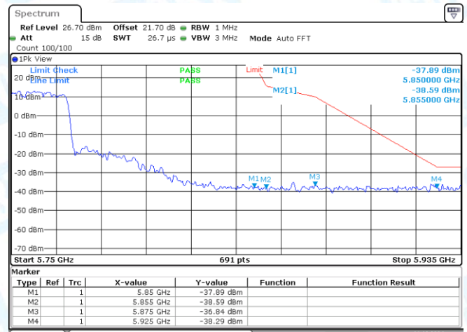
11AX80MIMO-Ant1-5775-PASS
