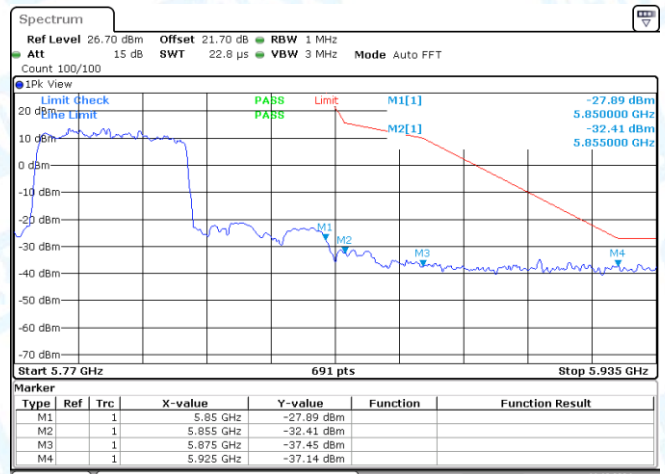
11AX40MIMO-Ant2-5755-PASS
