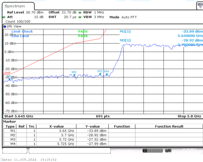
11AC80MIMO-Ant2-5775-PASS
