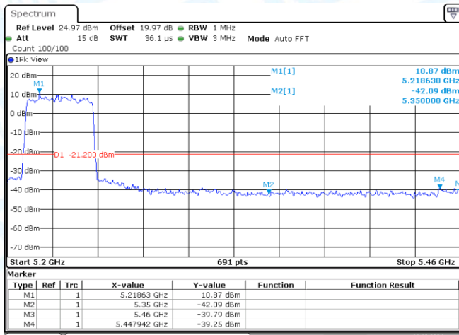
11AX40MIMO-Ant1-5190-PASS
