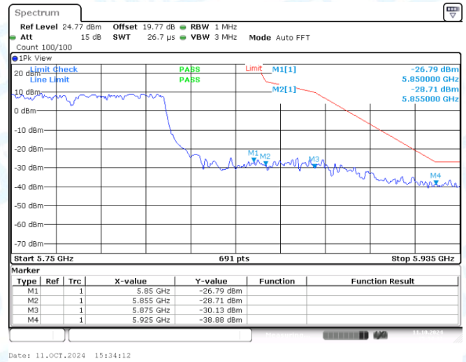
11AC80MIMO-Ant1-5775-PASS
