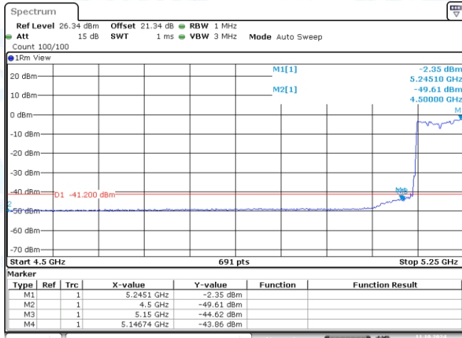
11AX80MIMO-Ant2-5210-PASS
