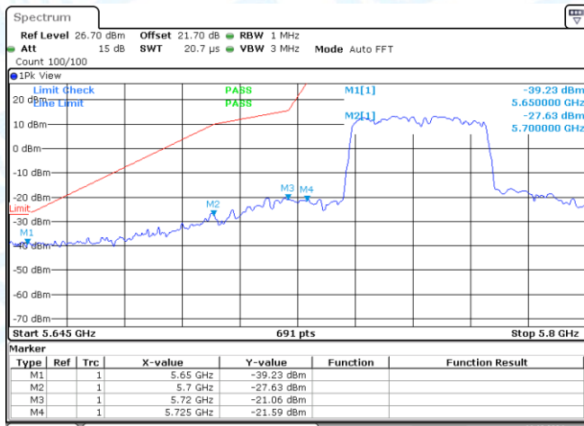
11AX80MIMO-Ant1-5775-PASS
