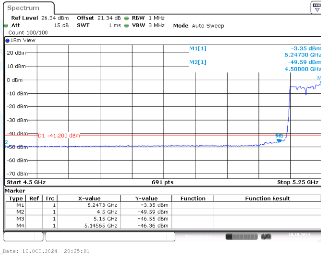
11AC80MIMO-Ant2-5210-PASS
