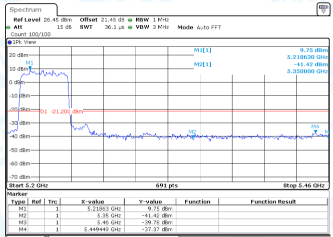
11AX40MIMO-Ant2-5190-PASS
