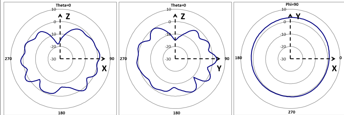
6G Radiation Pattern
