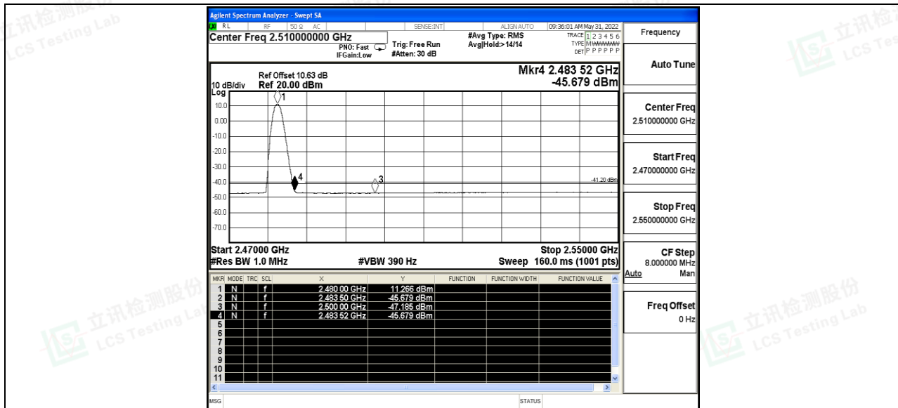
DH5_Ant_High_2480_Peak
