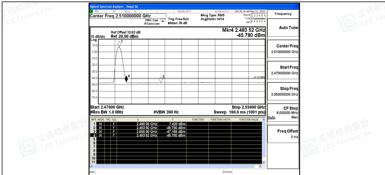
2DH5_Ant_High_2480_Peak
