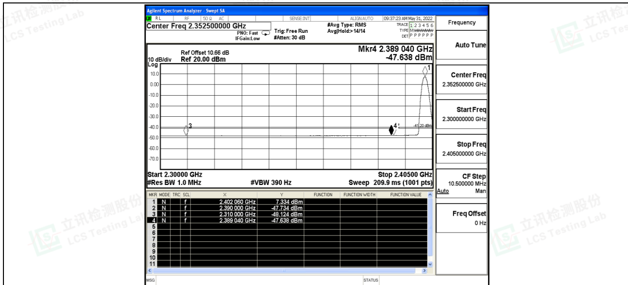
2DH5_Ant_Low_2402_Peak
