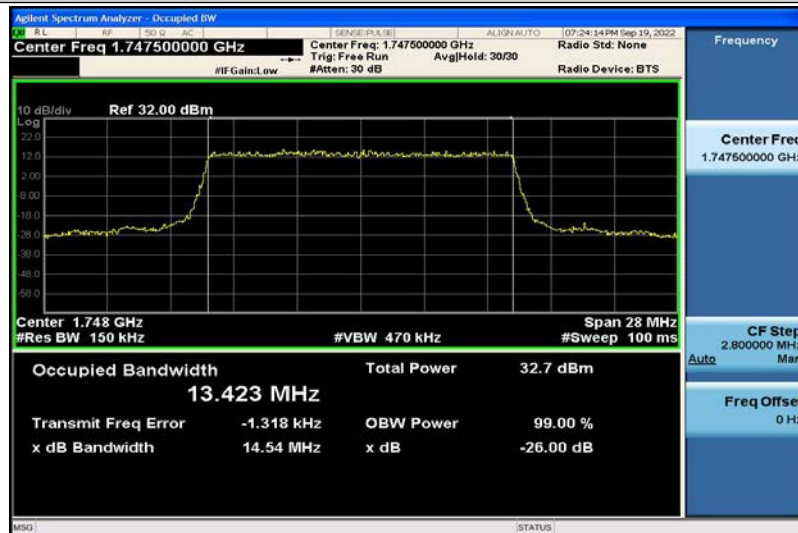
Band4-15MHz-QPSK-20325-75RB#0-13.423
