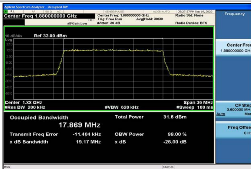
Band2-20MHz-16QAM-18900-100RB#0-17.869
