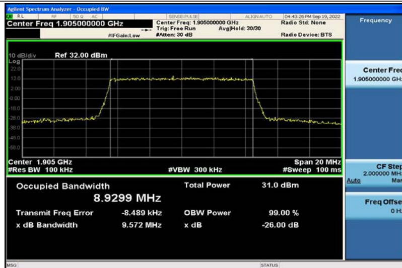
Band2-10MHz-16QAM-19150-50RB#0-8.9299
