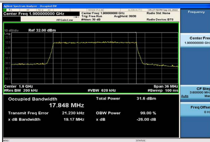
Band2-20MHz-16QAM-19100-100RB#0-17.848
