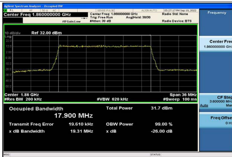
Band2-20MHz-16QAM-18700-100RB#0-17.900
