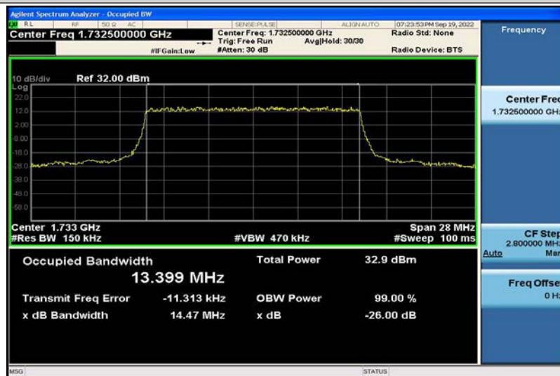
Band4-15MHz-QPSK-20175-75RB#0-13.399
