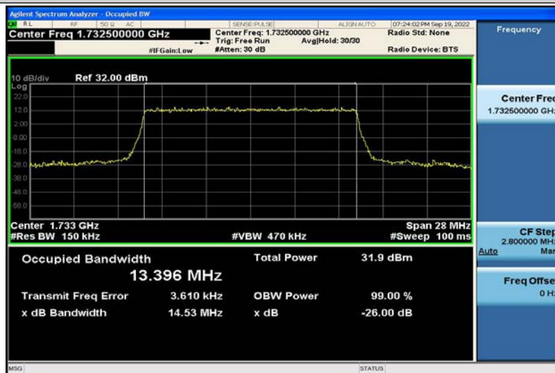
Band4-15MHz-16QAM-20175-75RB#0-13.396
