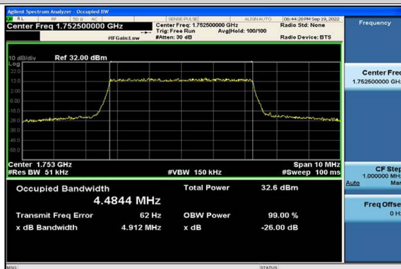
Band4-5MHz-QPSK-20375-25RB#0-4.4844
