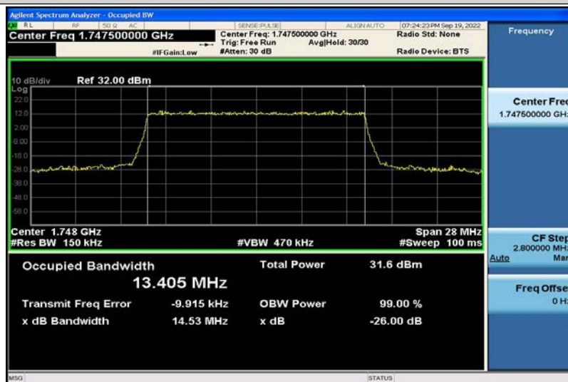
Band4-15MHz-16QAM-20325-75RB#0-13.405
