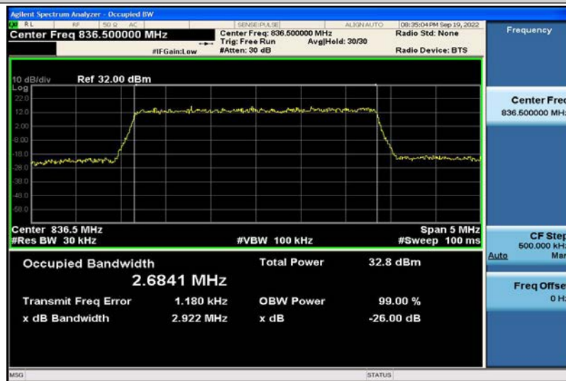
Band5-3MHz-16QAM-20525-15RB#0-2.6841
