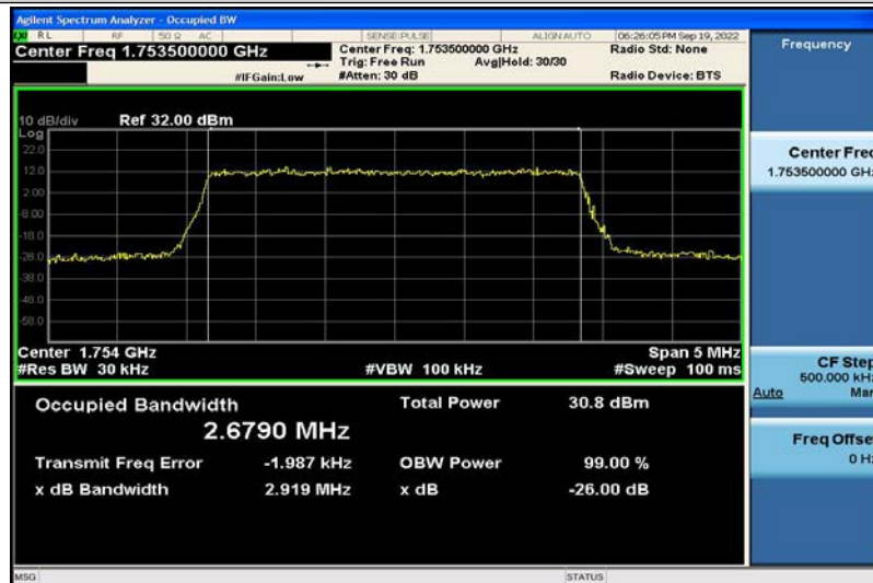
Band4-3MHz-16QAM-20385-15RB#0-2.6790
