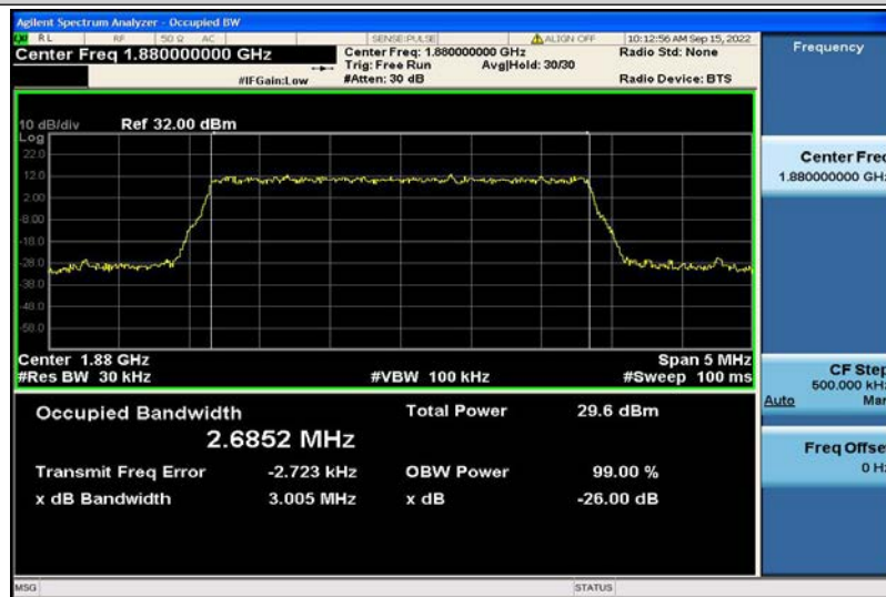
Band2-3MHz-16QAM-18900-15RB#0-2.6852
