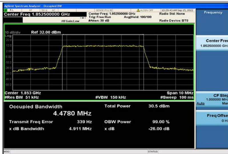
Band2-5MHz-16QAM-18625-25RB#0-4.4780
