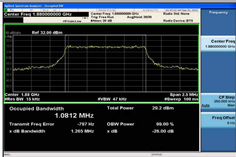
Band2-1.4MHz-16QAM-18900-6RB#0-1.0812
