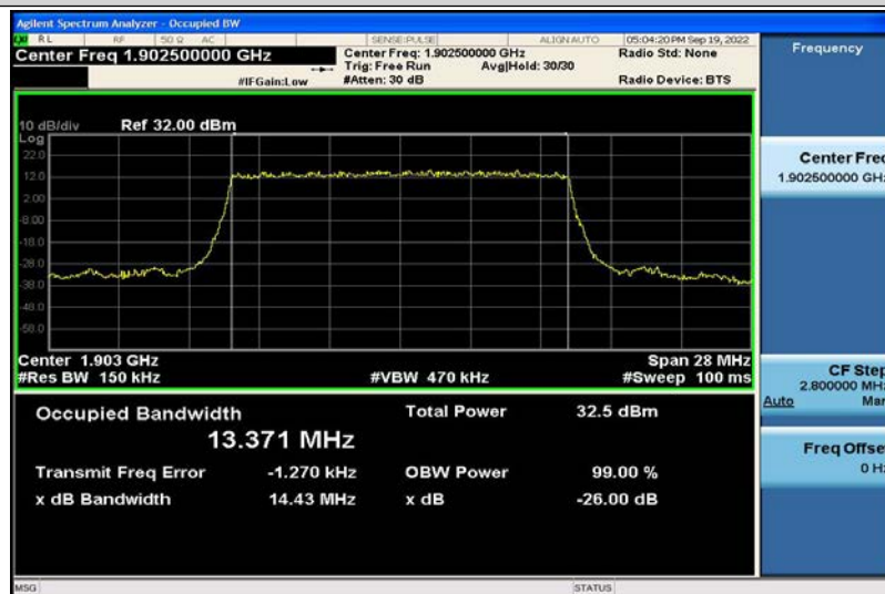
Band2-15MHz-QPSK-19125-75RB#0-13.371
