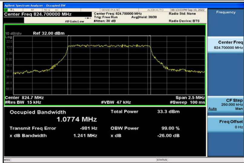
Band5-1.4MHz-QPSK-20407-6RB#0-1.0774
