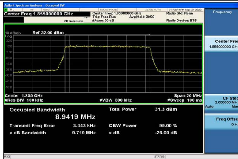
Band2-10MHz-16QAM-18650-50RB#0-8.9419
