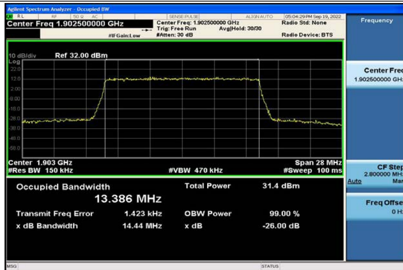
Band2-15MHz-16QAM-19125-75RB#0-13.386
