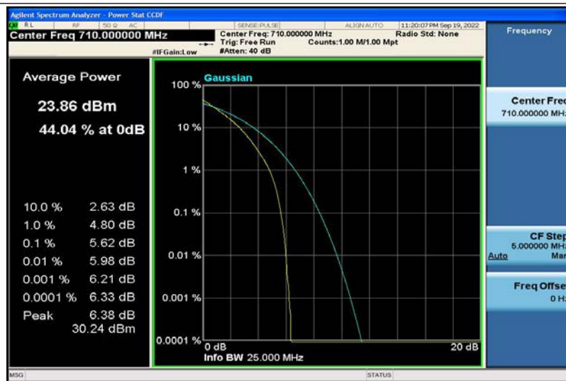
Band17-5MHz-QPSK-23790-25RB#0
