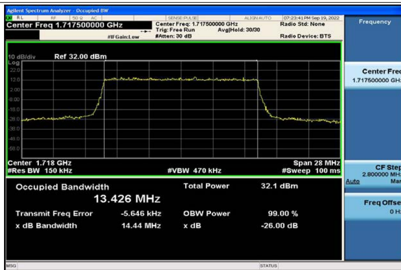
Band4-15MHz-16QAM-20025-75RB#0-13.426
