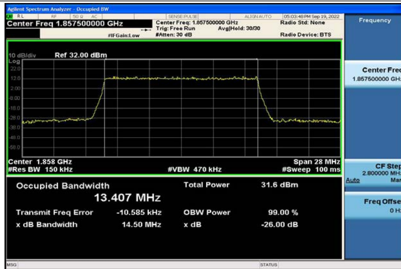
Band2-15MHz-16QAM-18675-75RB#0-13.407
