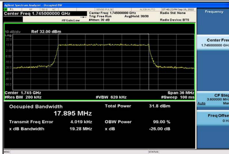
Band4-20MHz-16QAM-20300-100RB#0-17.895
