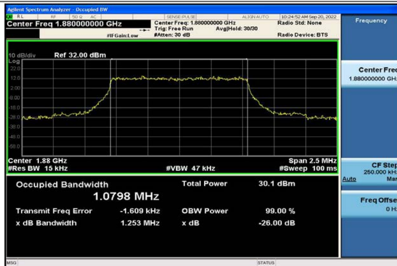
Band2-1.4MHz-QPSK-18900-6RB#0-1.0798
