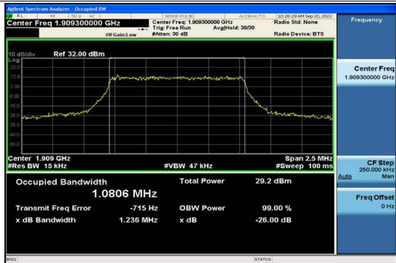
Band2-1.4MHz-16QAM-19193-6RB#0-1.0806
