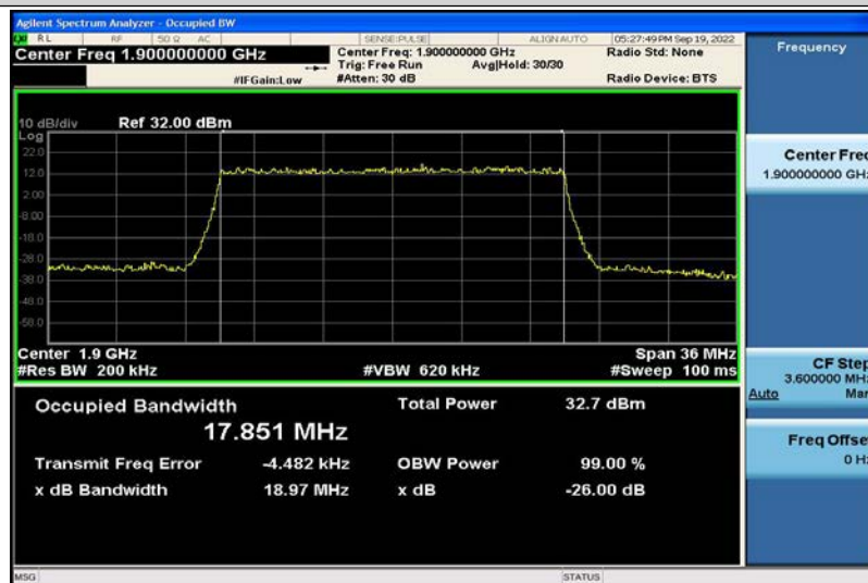
Band2-20MHz-QPSK-19100-100RB#0-17.851
