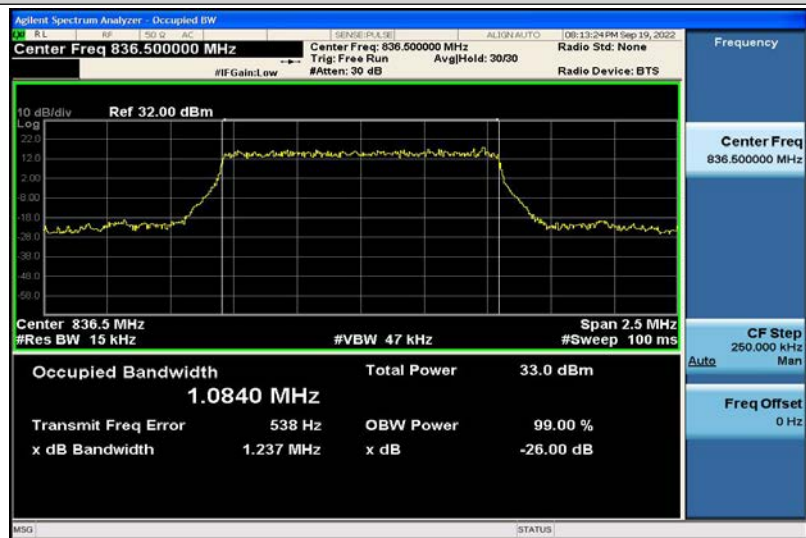
Band5-1.4MHz-QPSK-20525-6RB#0-1.0840
