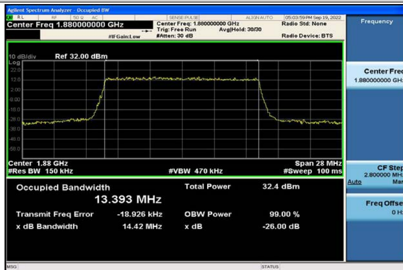
Band2-15MHz-QPSK-18900-75RB#0-13.393
