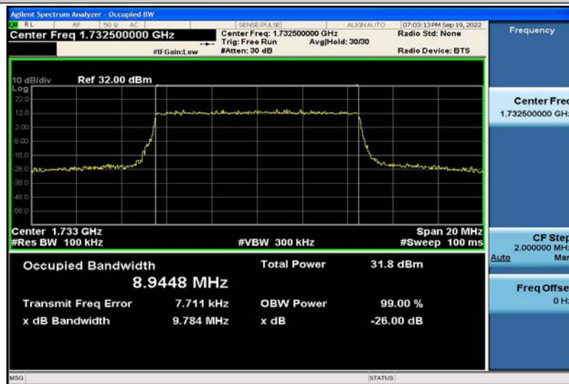
Band4-10MHz-16QAM-20175-50RB#0-8.9448
