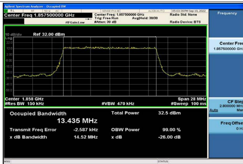
Band2-15MHz-QPSK-18675-75RB#0-13.435
