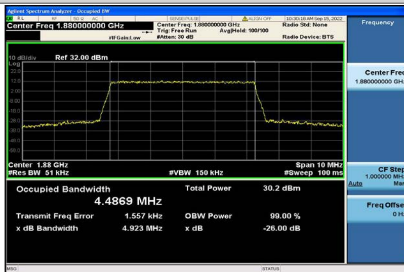
Band2-5MHz-16QAM-18900-25RB#0-4.4869
