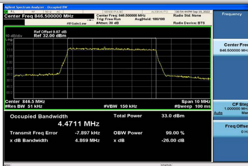
Band5-5MHz-16QAM-20625-25RB#0-4.4711
