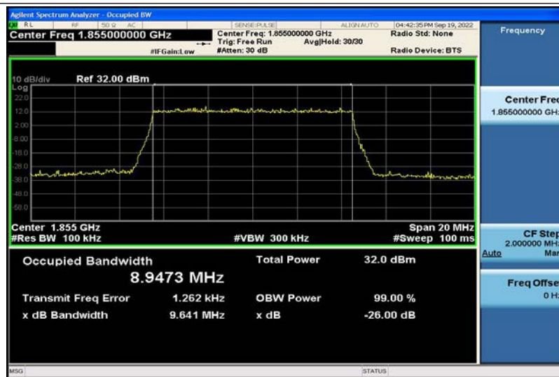
Band2-10MHz-QPSK-18650-50RB#0-8.9473
