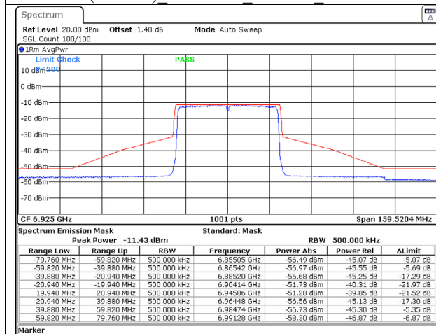
802.11ax (40MHz) 6925MHz Chain A NSS-1
