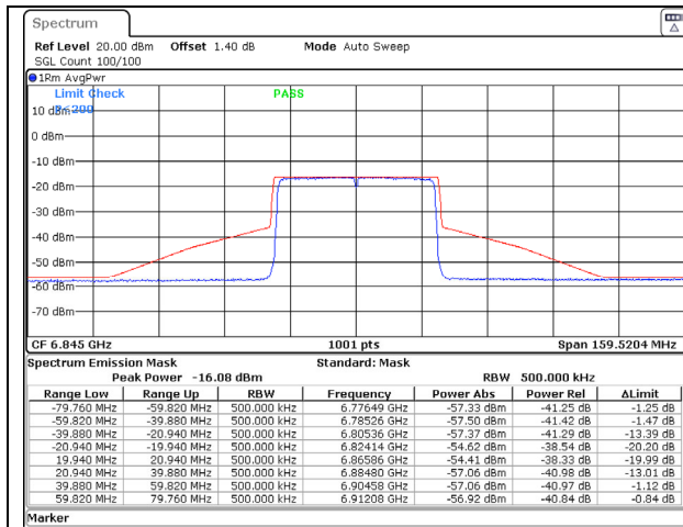
802.11ax (40MHz) 6845MHz Chain A NSS-1
