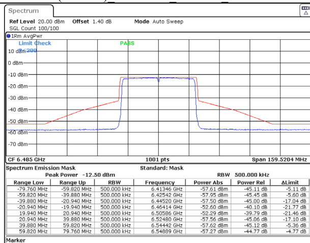
802.11ax (40MHz) 6485MHz Chain A NSS-1
