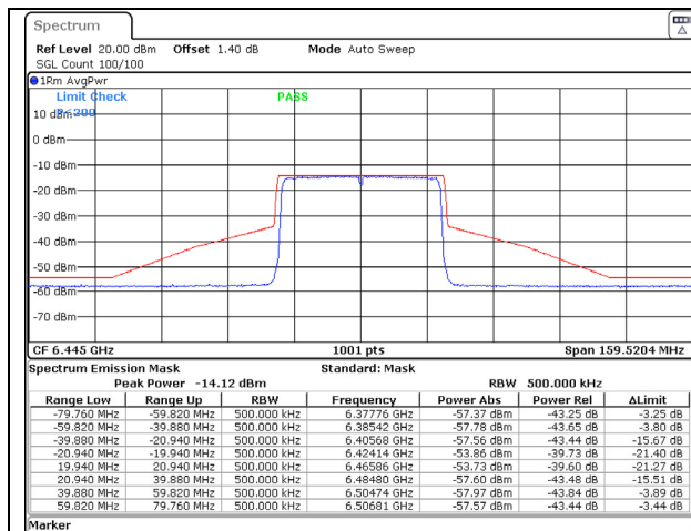
802.11ax (40MHz) 6445MHz Chain C NSS-1
