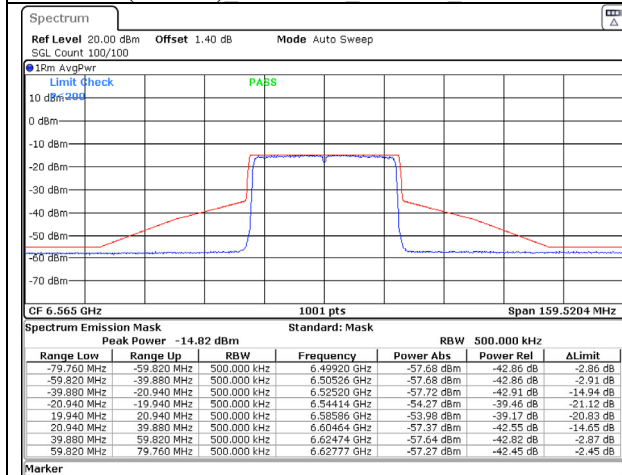
802.11ax (40MHz) 6565MHz Chain A NSS-1
