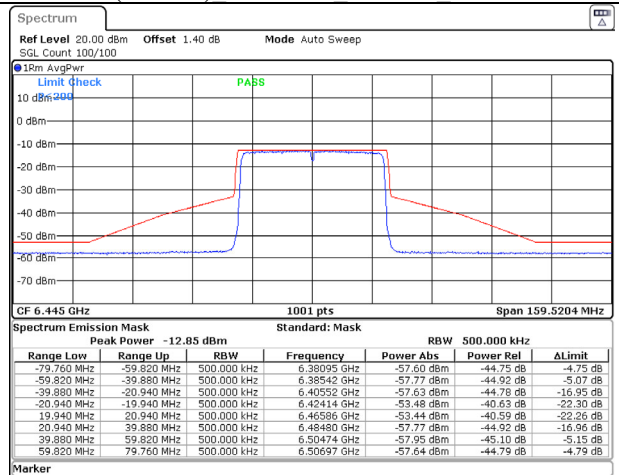
802.11ax (40MHz) 6445MHz Chain B NSS-1
