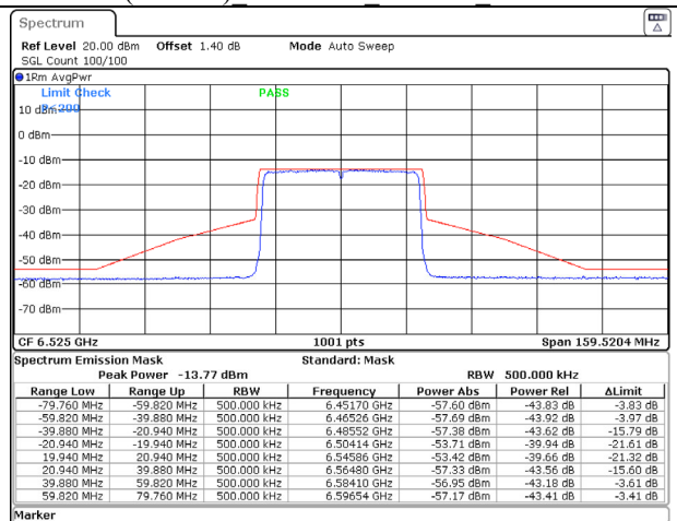
802.11ax (40MHz) 6525MHz Chain D NSS-1
