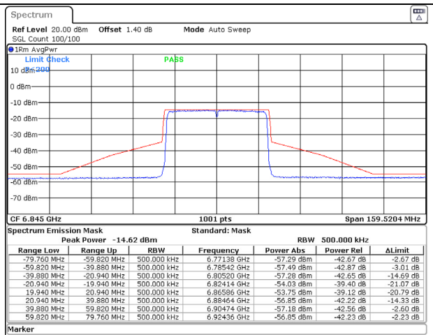
802.11ax (40MHz) 6845MHz Chain B NSS-1
