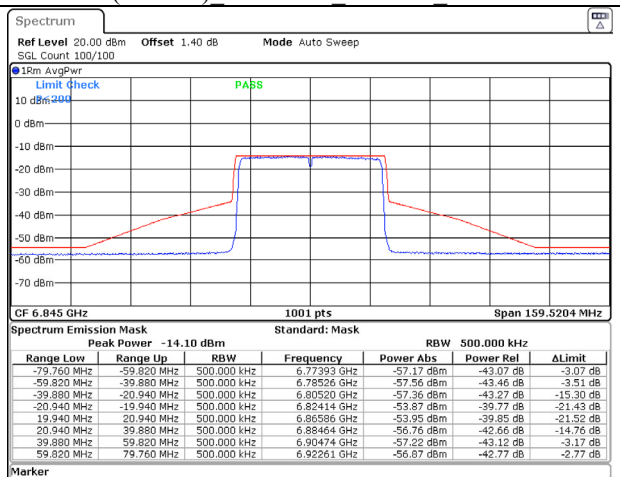
802.11ax (40MHz) 6845MHz Chain D NSS-1
