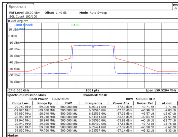
802.11ax (40MHz) 6565MHz Chain C NSS-1
