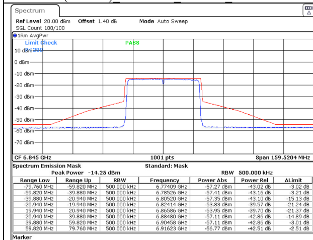
802.11ax (40MHz) 6845MHz Chain C NSS-1
