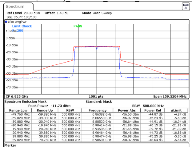
802.11ax (40MHz) 6925MHz Chain B NSS-1
