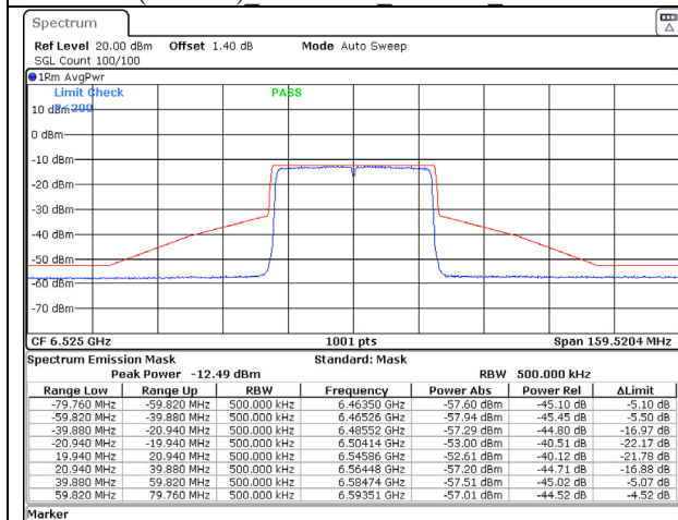
802.11ax (40MHz) 6525MHz Chain C NSS-1
