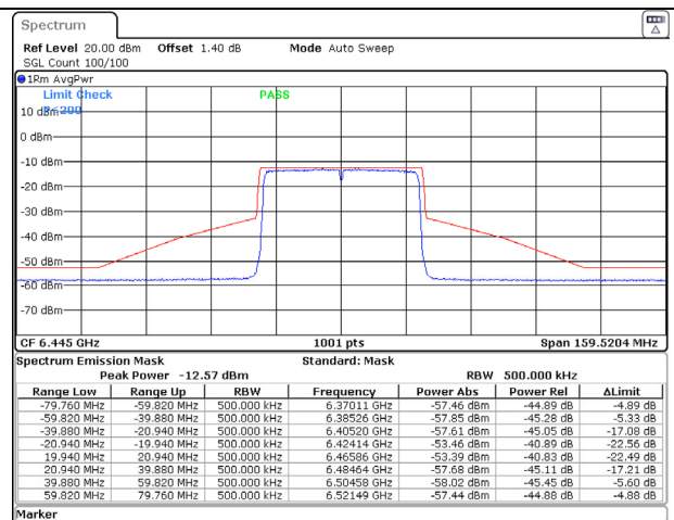
802.11ax (40MHz) 6445MHz Chain D NSS-1
