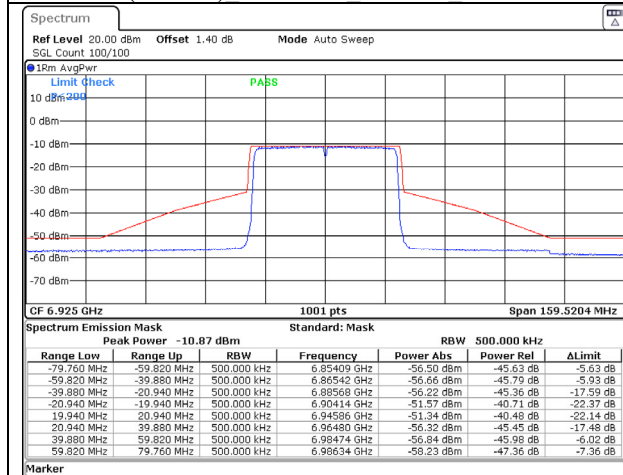
802.11ax (40MHz) 6925MHz Chain C NSS-1
