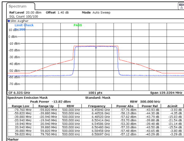
802.11ax (40MHz) 6525MHz Chain A NSS-1
