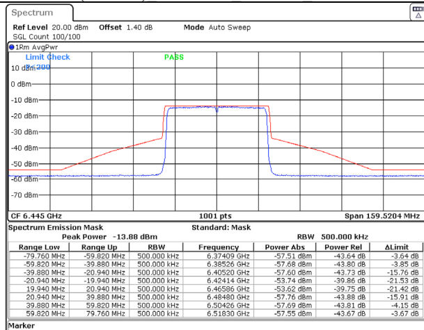
802.11ax (40MHz) 6445MHz Chain A NSS-1
