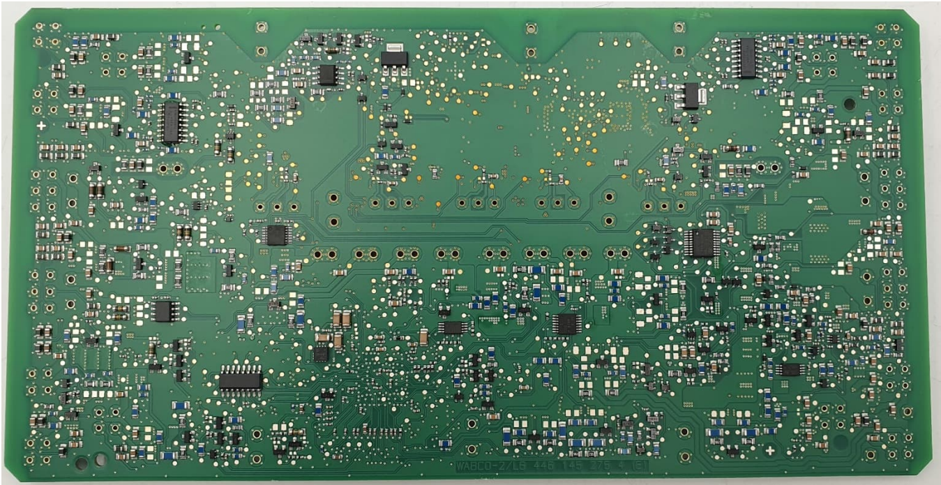
PCB bottom view, (provided by ZF CV Systems Hannover GmbH)
