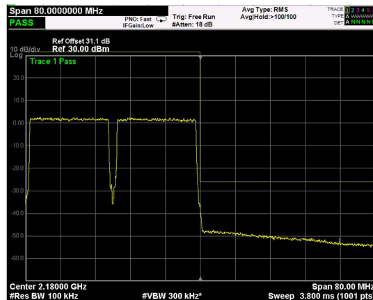
High Band Edge, 2 Carrier, Modulation: 16QAM, BW=20MHz
