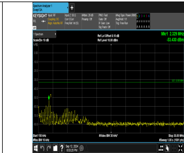
Band4_5MHz_QPSK_20375_1RB#0_0.15~30_0.15~30
