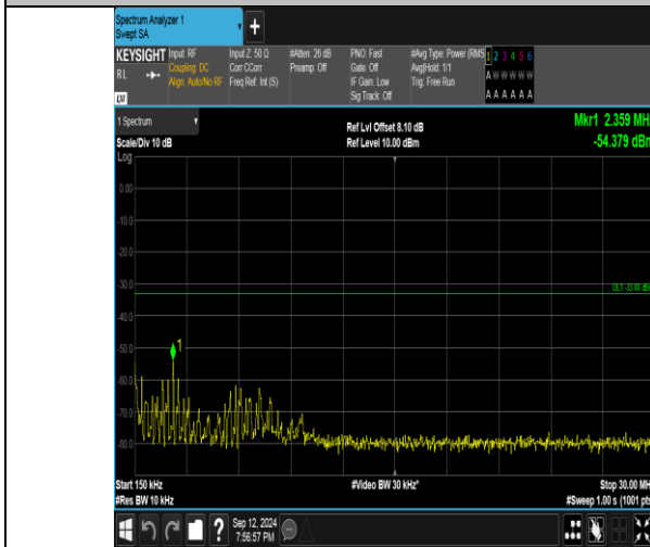
Band4_5MHz_16QAM_19975_25RB#0_0.15~30_0.15~30
