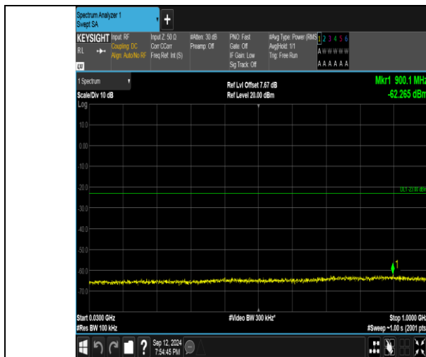
Band4_5MHz_QPSK_19975_1RB#24_30~1000_30~1000
