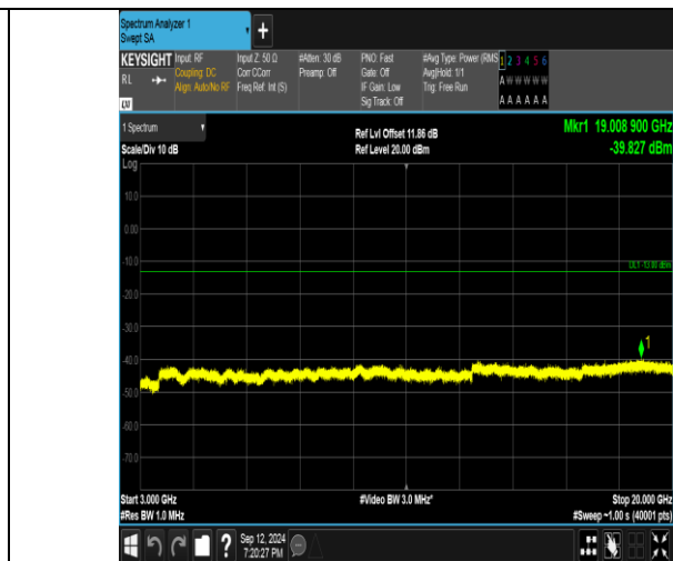
Band4_3MHz_16QAM_20385_1RB#14_3000~20000_3000~20000
