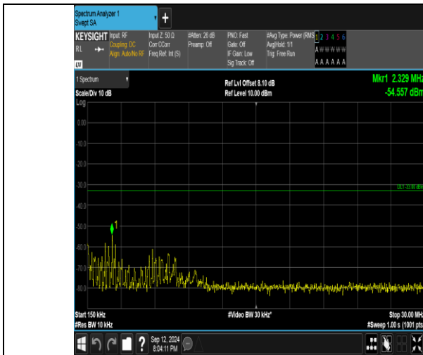
Band4_5MHz_16QAM_20375_1RB#0_0.15~30_0.15~30
