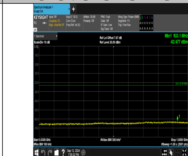
Band4_5MHz_16QAM_19975_1RB#24_30~1000_30~1000
