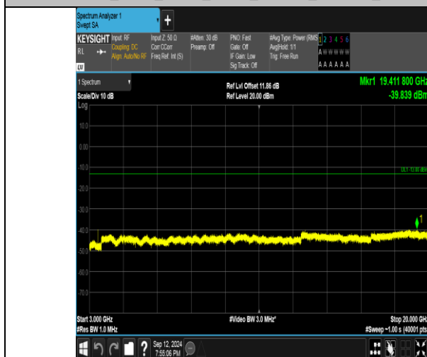
Band4_5MHz_QPSK_19975_1RB#24_3000~20000_3000~20000
