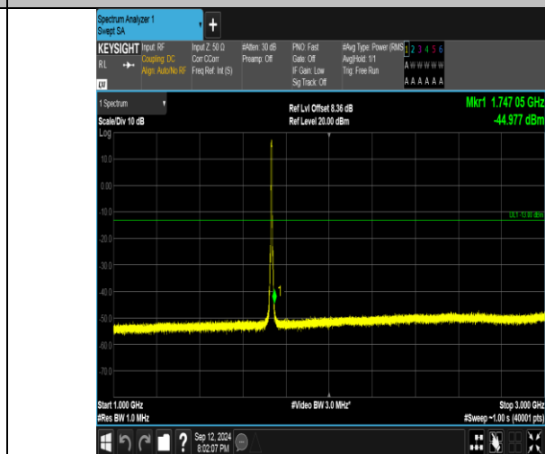
Band4_5MHz_QPSK_20175_25RB#0_1000~3000_1000~3000
