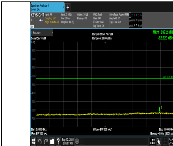
Band4_5MHz_QPSK_20375_1RB#24_30~1000_30~1000
