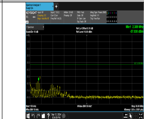
Band4_5MHz_QPSK_20375_1RB#24_0.15~30_0.15~30
