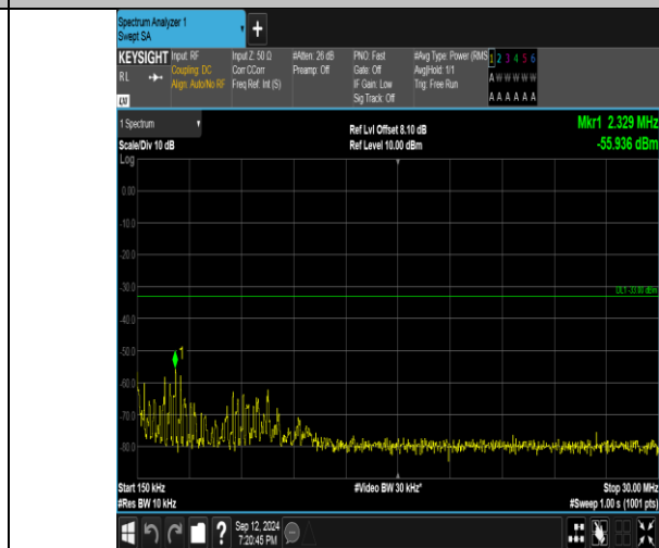
Band4_3MHz_QPSK_20385_15RB#0_0.15~30_0.15~30
