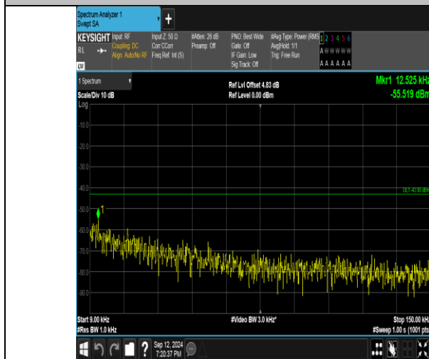
Band4_3MHz_QPSK_20385_15RB#0_0.009~0.15_0.009~0.15
