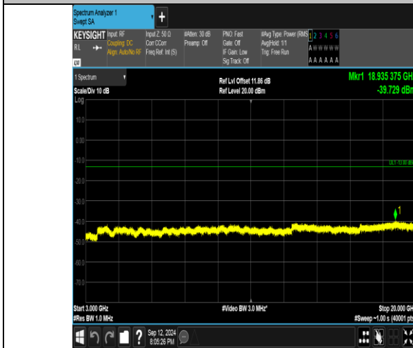
Band4_5MHz_QPSK_20375_1RB#24_3000~20000_3000~20000
