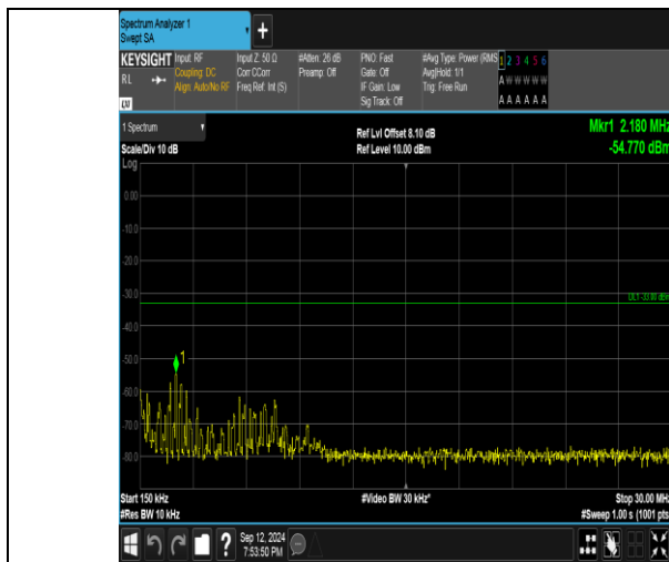
Band4_5MHz_16QAM_19975_1RB#0_0.15-30_0.15-30
