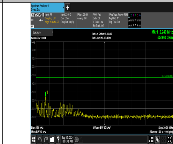
Band4_5MHz_QPSK_20175_25RB#0_0.15~30_0.15~30
