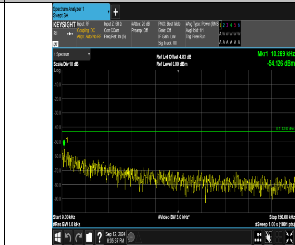
Band4_5MHz_16QAM_20375_1RB#24_0.009~0.15_0.009~0.15
