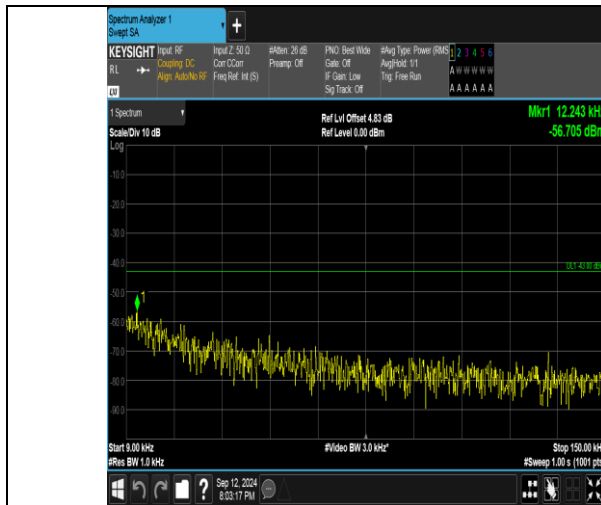
Band4_5MHz_QPSK_20375_1RB#0_0.009~0.15_0.009~0.15
