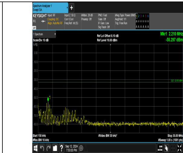
Band4_5MHz_QPSK_19975_1RB#0_0.15~30_0.15~30
