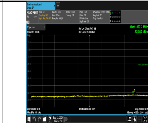
Band4_5MHz_16QAM_20175_25RB#0_30~1000_30~1000
