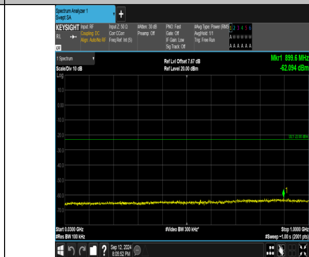
Band4_5MHz_16QAM_20375_1RB#24_30~1000_30~1000
