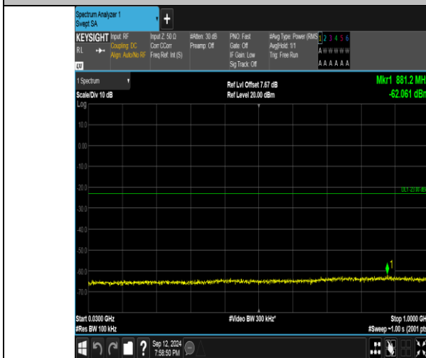
Band4_5MHz_QPSK_20175_1RB#0_30~1000_30~1000
