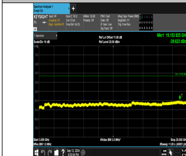
Band4_5MHz_QPSK_20375_1RB#0_3000~20000_3000~20000
