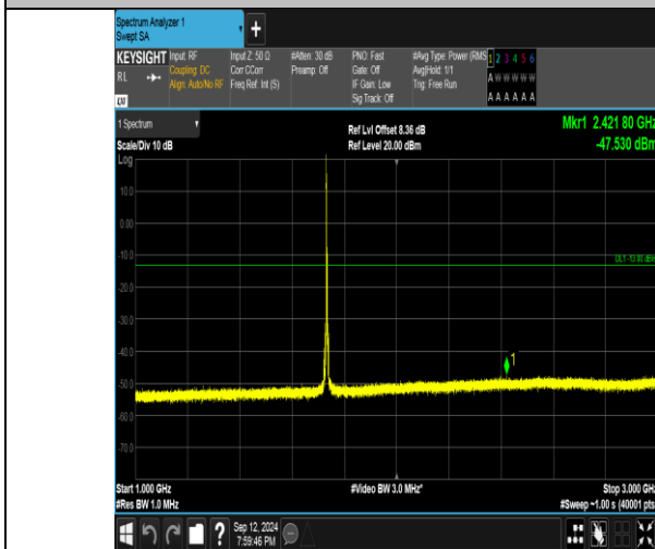
Band4_5MHz_16QAM_20175_1RB#0_1000-3000_1000-3000
