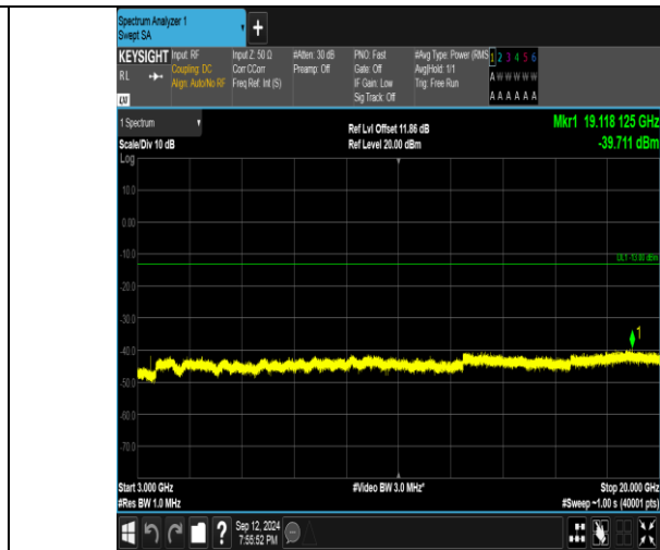
Band4_5MHz_16QAM_19975_1RB#24_3000~20000_3000~20000
