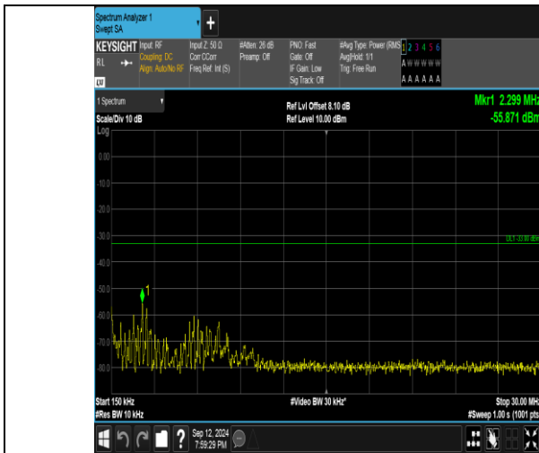
Band4_5MHz_16QAM_20175_1RB#0_0.15-30_0.15-30
