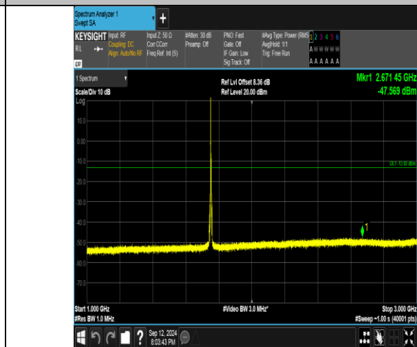
Band4_5MHz_QPSK_20375_1RB#0_1000~3000_1000~3000
