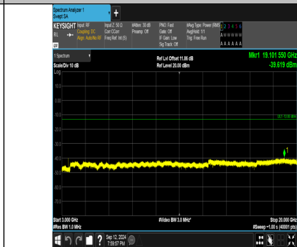
Band4_5MHz_16QAM_20175_1RB#0_3000-20000_3000-20000
