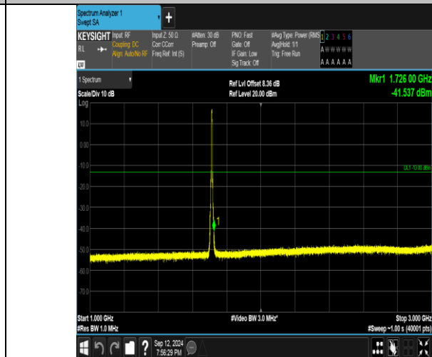
Band4_5MHz_QPSK_19975_25RB#0_1000~3000_1000~3000
