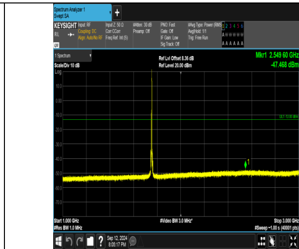
Band4_5MHz_QPSK_20375_1RB#24_1000~3000_1000~3000
