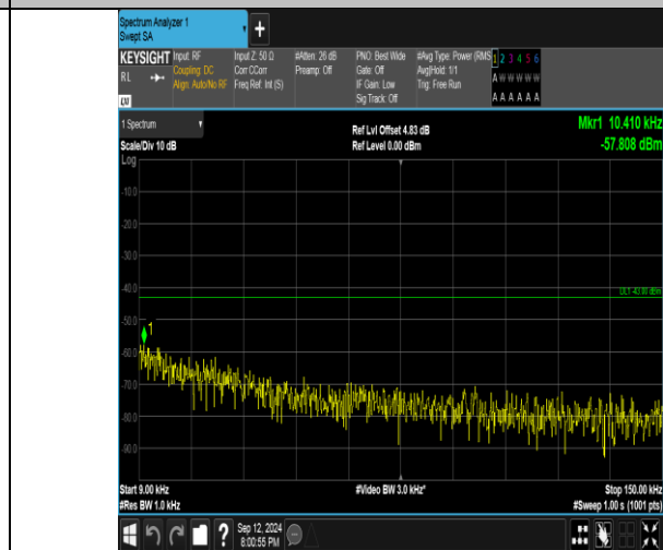
Band4_5MHz_16QAM_20175_1RB#24_0.009~0.15_0.009~0.15
