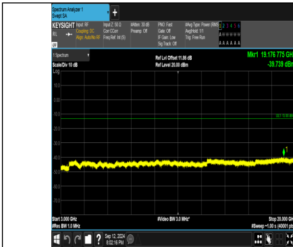
Band4_5MHz_QPSK_20175_25RB#0_3000~20000_3000~20000
