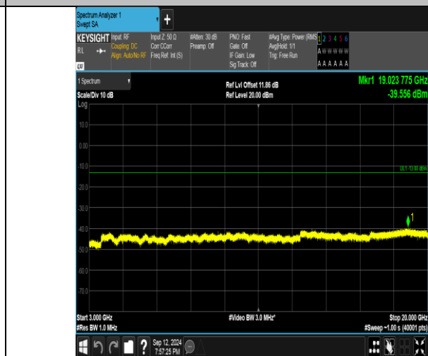
Band4_5MHz_16QAM_19975_25RB#0_3000~20000_3000~20000
