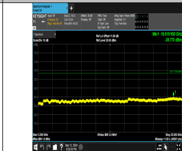
Band4_5MHz_16QAM_20175_25RB#0_3000~20000_3000~20000
