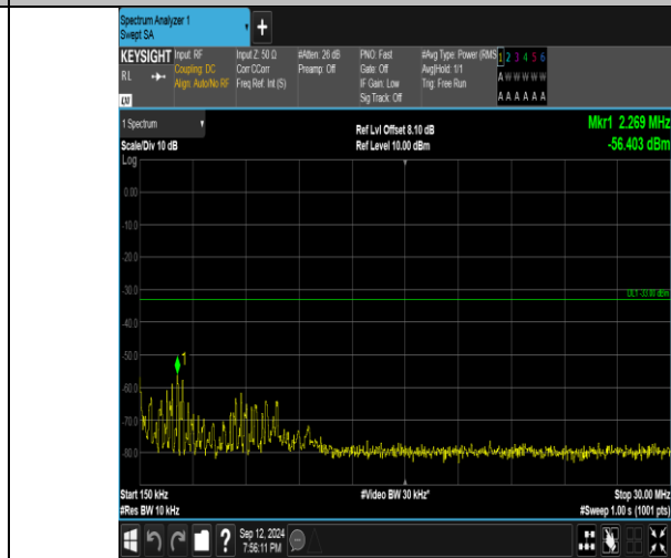
Band4_5MHz_QPSK_19975_25RB#0_0.15~30_0.15~30
