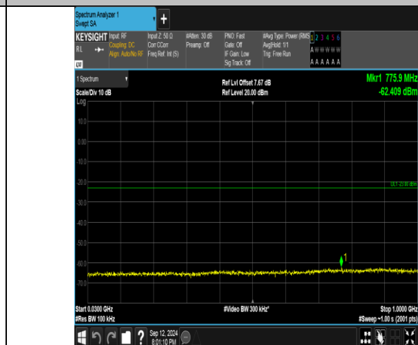
Band4_5MHz_16QAM_20175_1RB#24_30~1000_30~1000
