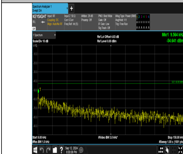
Band4_5MHz_QPSK_20175_1RB#24_0.009-0.15_0.009-0.15
