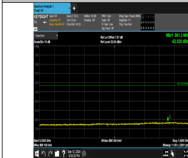
Band4_5MHz_QPSK_20375_1RB#0_30~1000_30~1000
