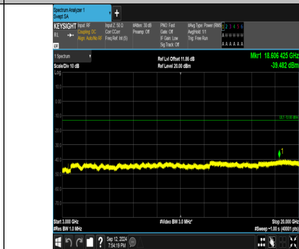
Band4_5MHz_16QAM_19975_1RB#0_3000-20000_3000-20000
