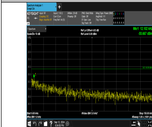
Band4_5MHz_QPSK_20375_1RB#24_0.009~0.15_0.009~0.15
