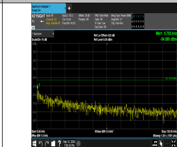
Band4_5MHz_16QAM_19975_1RB#24_0.009~0.15_0.009~0.15
