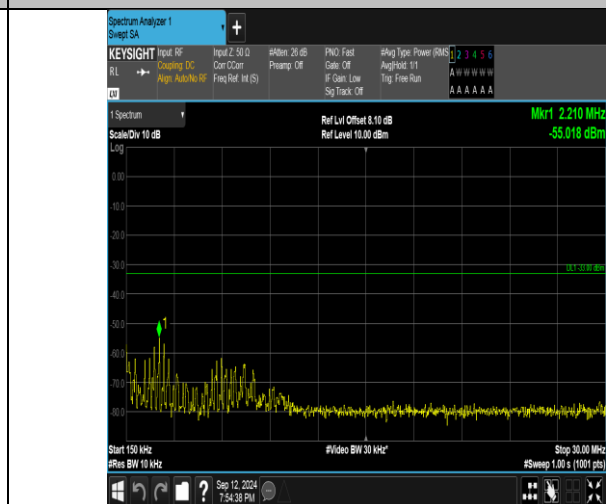
Band4_5MHz_QPSK_19975_1RB#24_0.15-30_0.15-30
