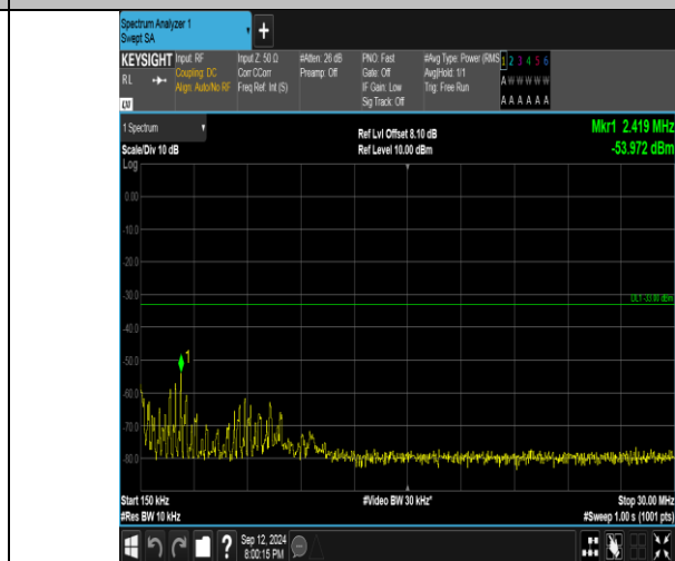
Band4_5MHz_QPSK_20175_1RB#24_0.15-30_0.15-30
