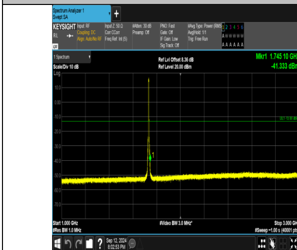
Band4_5MHz_16QAM_20175_25RB#0_1000~3000_1000~3000
