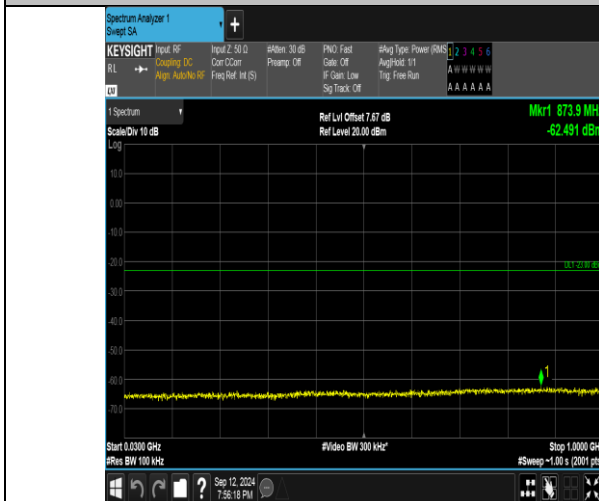
Band4_5MHz_QPSK_19975_25RB#0_30~1000_30~1000
