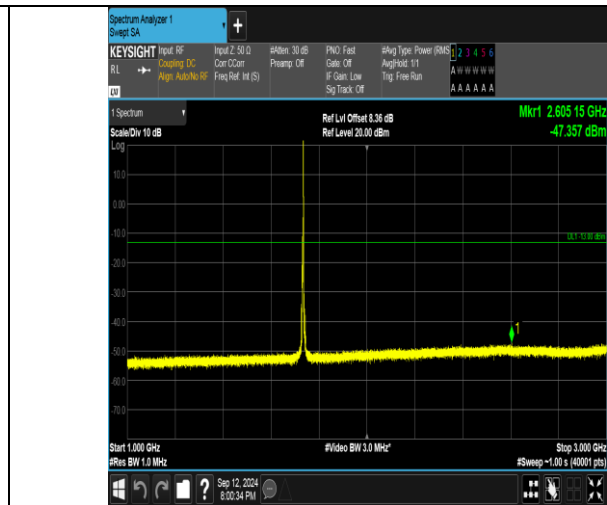
Band4_5MHz_QPSK_20175_1RB#24_1000~3000_1000~3000
