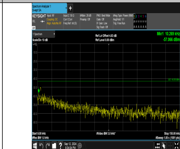
Band4_5MHz_16QAM_20375_1RB#0_0.009~0.15_0.009~0.15
