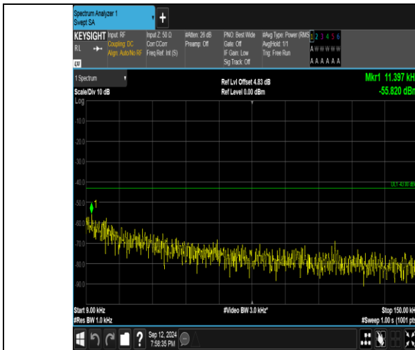
Band4_5MHz_QPSK_20175_1RB#0_0.009~0.15_0.009~0.15
