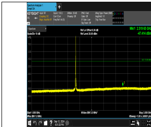
Band4_5MHz_16QAM_20175_1RB#24_1000~3000_1000~3000
