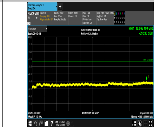
Band4_5MHz_16QAM_20375_1RB#0_3000~20000_3000~20000
