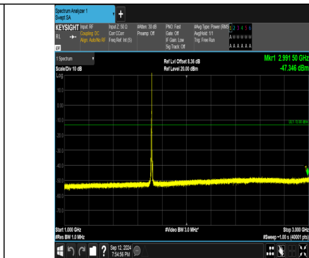
Band4_5MHz_QPSK_19975_1RB#24_1000~3000_1000~3000
