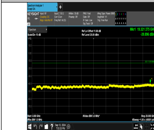
Band4_5MHz_QPSK_19975_1RB#0_3000~20000_3000~20000
