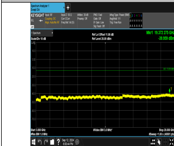
Band4_5MHz_QPSK_20175_1RB#24_3000~20000_3000~20000
