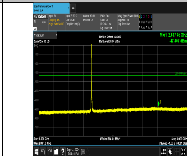
Band4_5MHz_QPSK_19975_1RB#0_1000~3000_1000~3000
