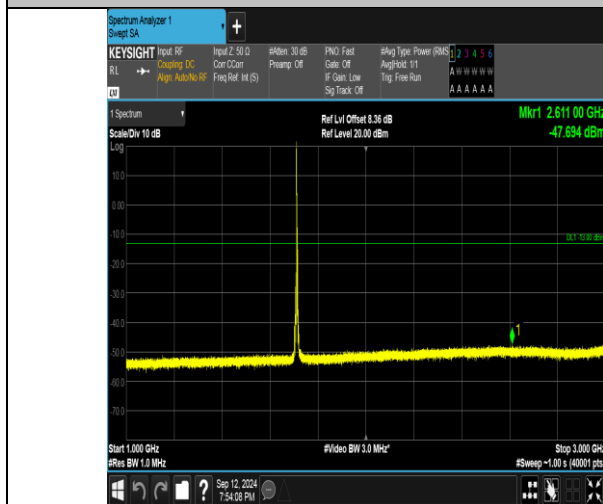
Band4_5MHz_16QAM_19975_1RB#0_1000-3000_1000-3000
