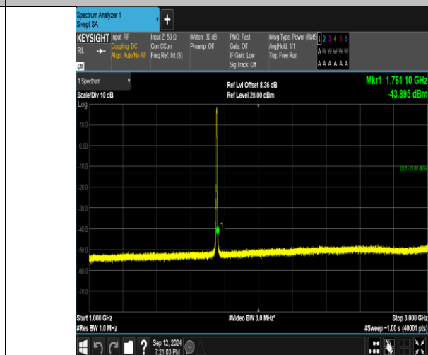
Band4_3MHz_QPSK_20385_15RB#0_1000~3000_1000~3000
