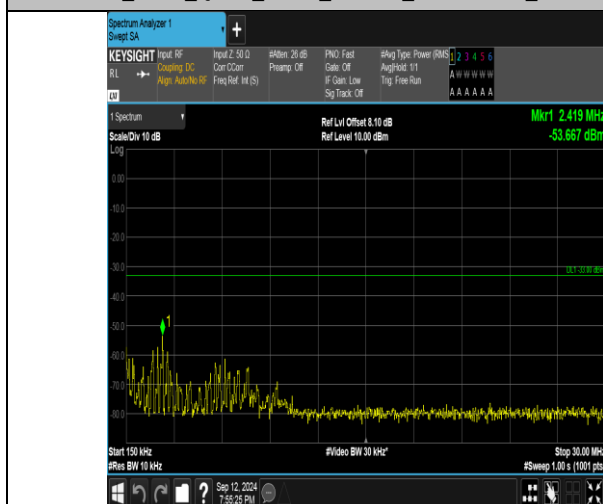
Band4_5MHz_16QAM_19975_1RB#24_0.15~30_0.15~30
