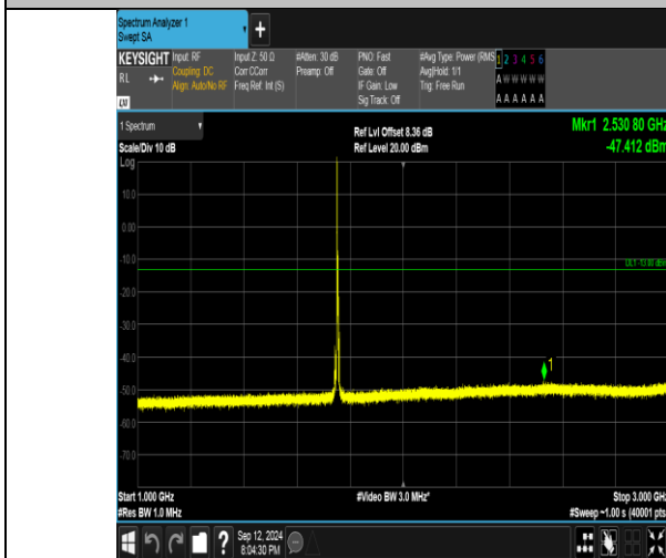
Band4_5MHz_16QAM_20375_1RB#0_1000~3000_1000~3000
