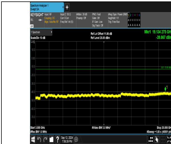
Band4_5MHz_QPSK_19975_25RB#0_3000~20000_3000~20000
