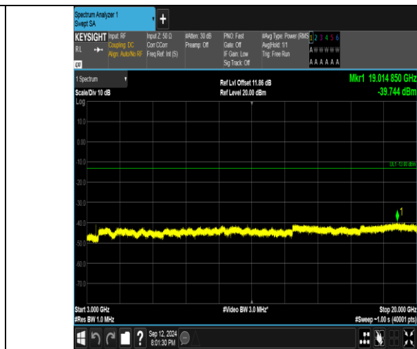
Band4_5MHz_16QAM_20175_1RB#24_3000~20000_3000~20000
