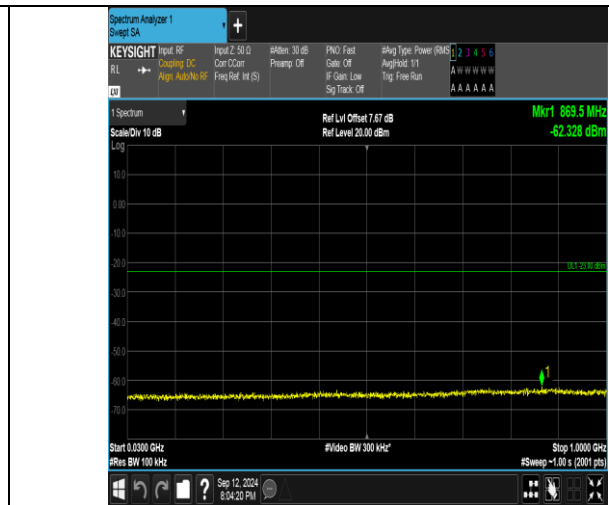
Band4_5MHz_16QAM_20375_1RB#0_30~1000_30~1000
