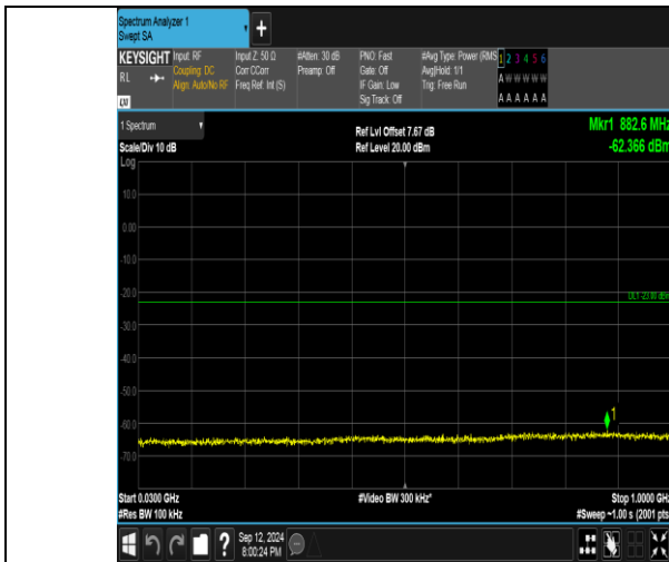
Band4_5MHz_QPSK_20175_1RB#24_30~1000_30~1000
