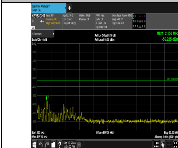
Band4_5MHz_16QAM_20175_1RB#24_0.15~30_0.15~30
