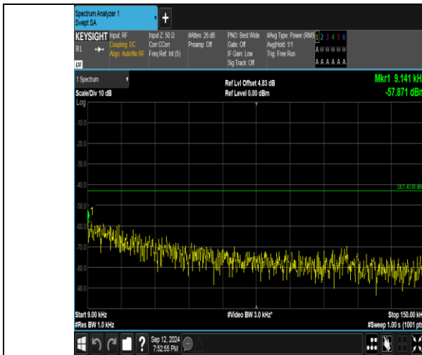
Band4_5MHz_QPSK_19975_1RB#0_0.009~0.15_0.009~0.15
