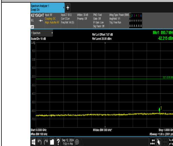
Band4_5MHz_QPSK_19975_1RB#0_30~1000_30~1000
