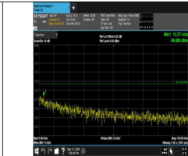
Band4_5MHz_16QAM_19975_25RB#0_0.009~0.15_0.009~0.15
