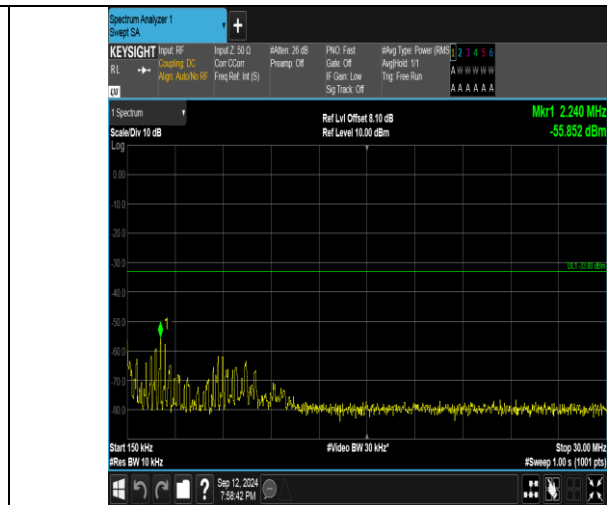
Band4_5MHz_QPSK_20175_1RB#0_0.15~30_0.15~30
