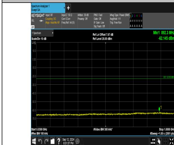
Band4_5MHz_QPSK_20175_25RB#0_30~1000_30~1000
