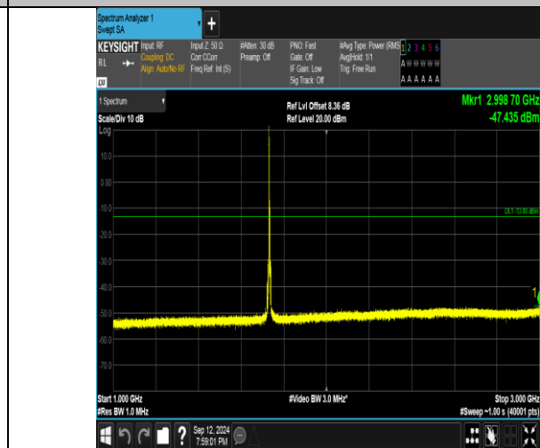
Band4_5MHz_QPSK_20175_1RB#0_1000~3000_1000~3000
