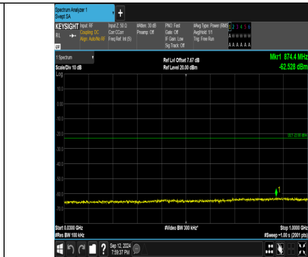
Band4_5MHz_16QAM_20175_1RB#0_30-1000_30-1000
