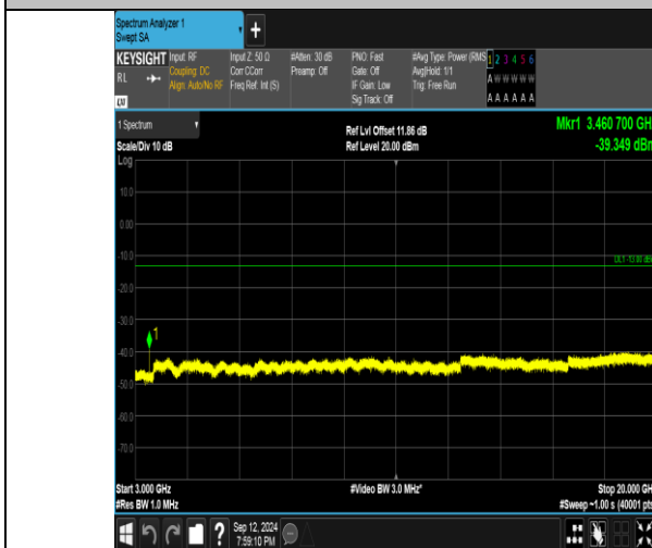
Band4_5MHz_QPSK_20175_1RB#0_3000~20000_3000~20000
