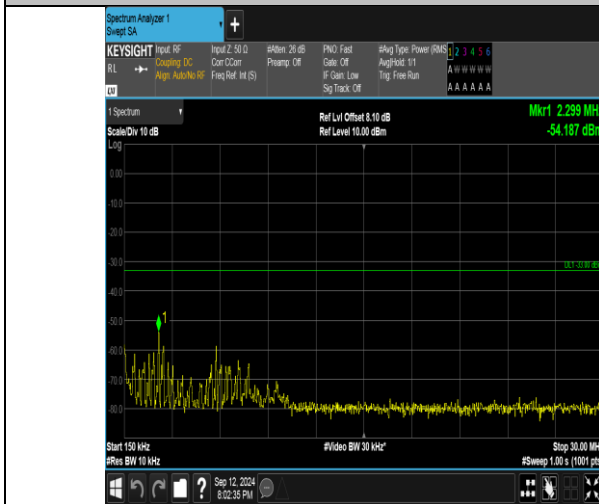
Band4_5MHz_16QAM_20175_25RB#0_0.15~30_0.15~30
