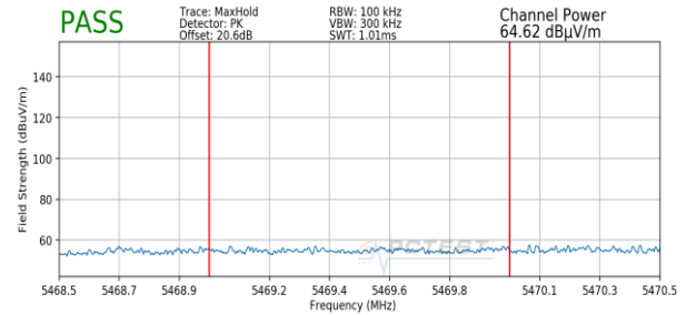
Plot 7-336. Radiated Lower Band Edge Plot MIMO (Peak – UNII Band 2C)
