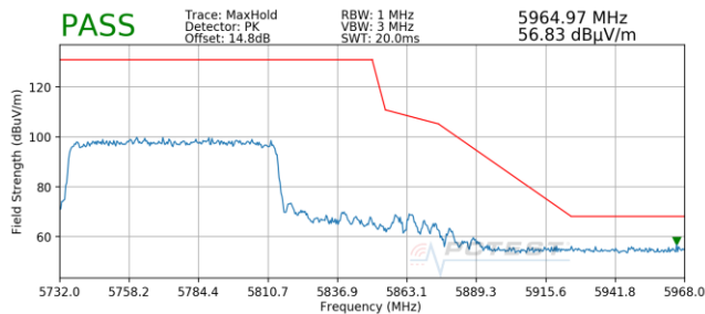
Plot 7-351. Radiated Upper Band Edge Plot MIMO (Peak – UNII Band 3)
