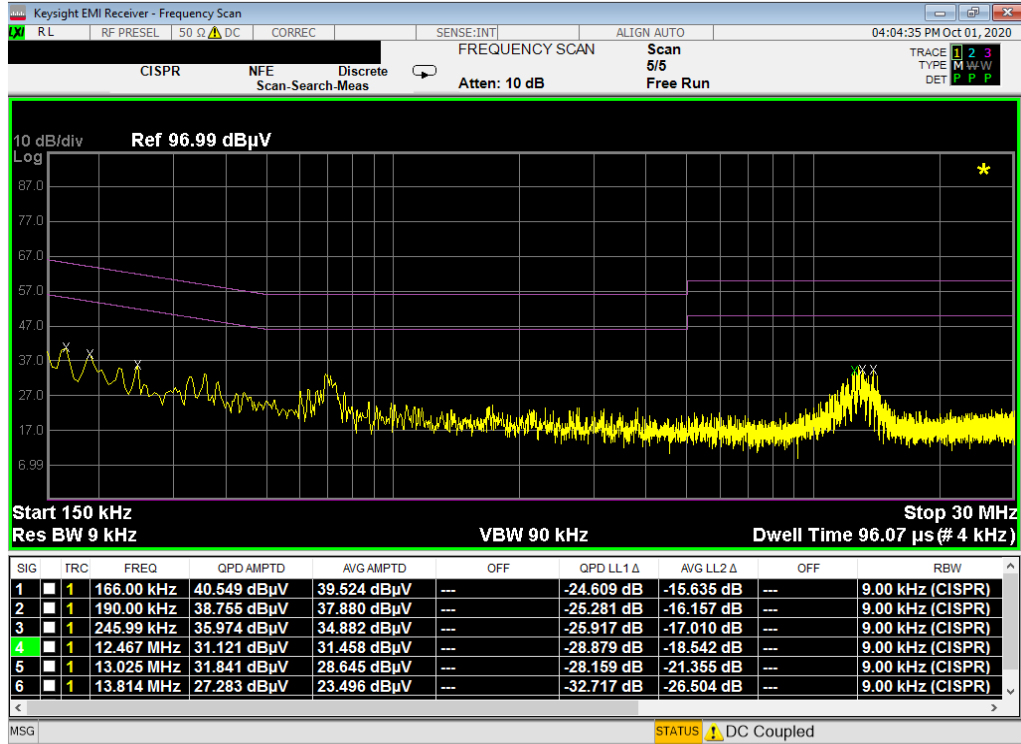
Plot 7-357. Line Conducted Plot with 802.11a UNII Band 2C (L1)
