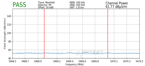
Plot 7-329. Radiated Lower Band Edge Plot SISO ANT2 (Peak - UNII Band 2C)
