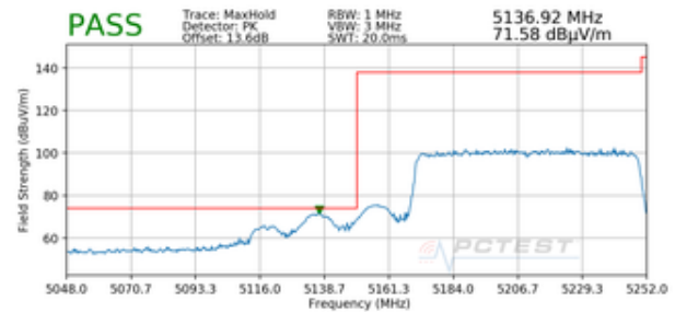
Plot 7-325. Radiated Lower Band Edge Plot SISO ANT2 (Peak – UNII Band 1)
