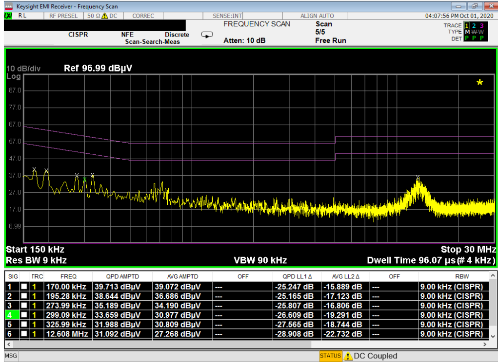
Plot 7-359. Line Conducted Plot with 802.11a UNII Band 3 (L1)
