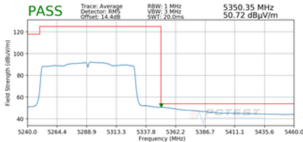
Plot 7-326. Radiated Upper Band Edge Plot SISO ANT2 (Average – UNII Band 2A)
