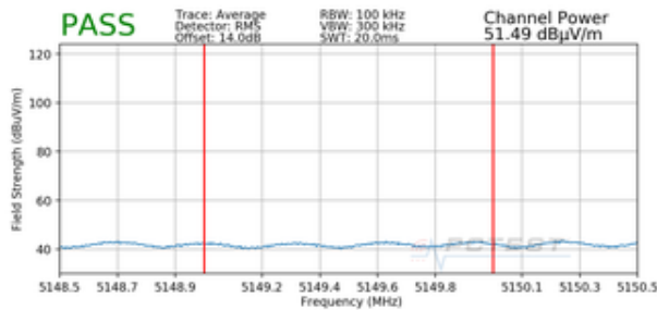
Plot 7-345. Radiated Lower Band Edge Plot MIMO (Average – UNII Band 1)
