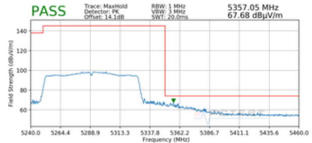
Plot 7-306. Radiated Upper Band Edge Plot SISO ANT1 (Peak – UNII Band 2A)
