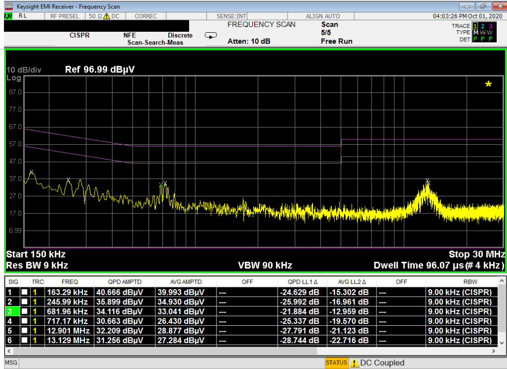
Plot 7-355. Line Conducted Plot with 802.11a UNII Band 2A (L1)
