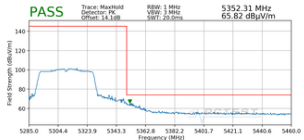
Plot 7-299. Radiated Upper Band Edge Plot SISO ANT1 (Peak – UNII Band 2A)
