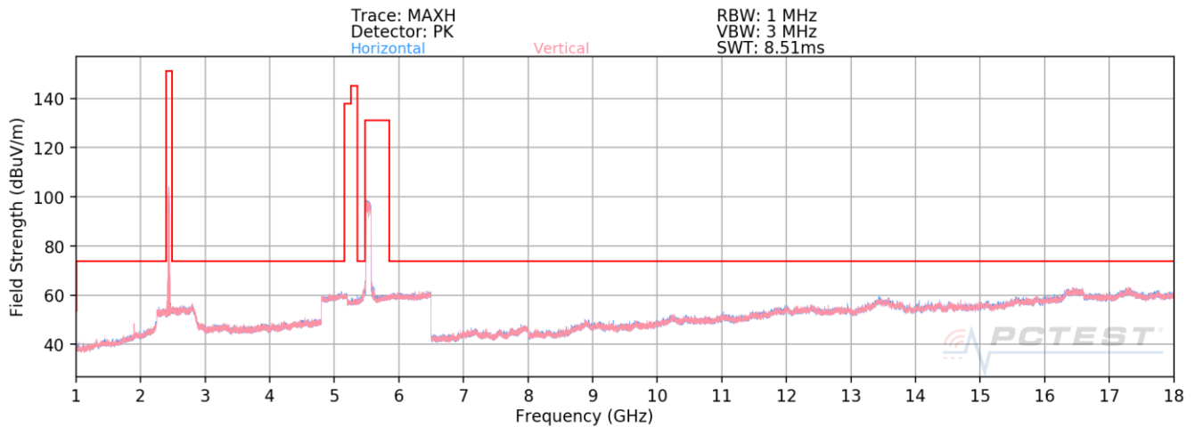
Plot 7-283. Radiated Spurious Plot above 1GHz (5GHz – 2.4 GHz)
