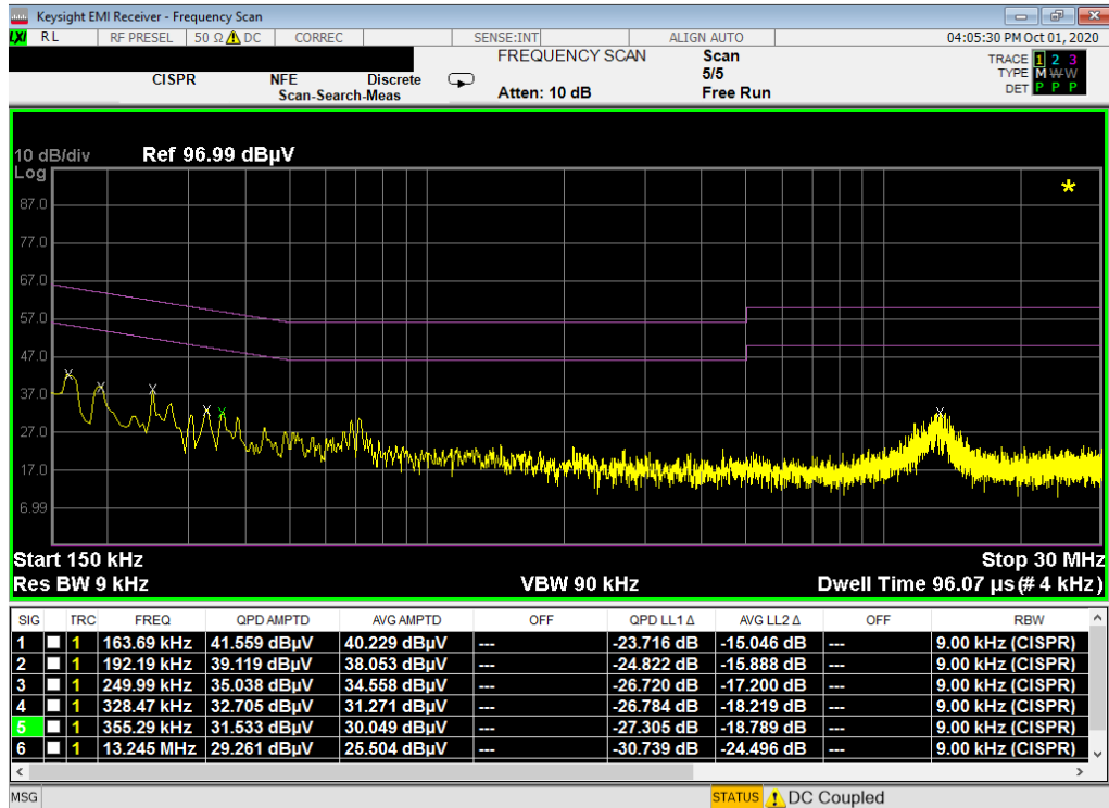
Plot 7-358. Line Conducted Plot with 802.11a UNII Band 2C (N)
