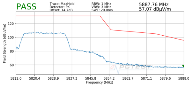
Plot 7-337. Radiated Upper Band Edge Plot MIMO (Peak – UNII Band 3)
