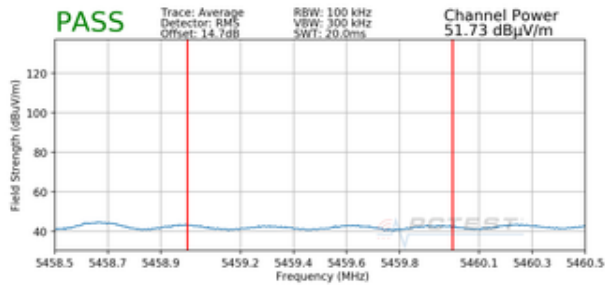
Plot 7-349. Radiated Lower Band Edge Plot MIMO (Average – UNII Band 2C)
