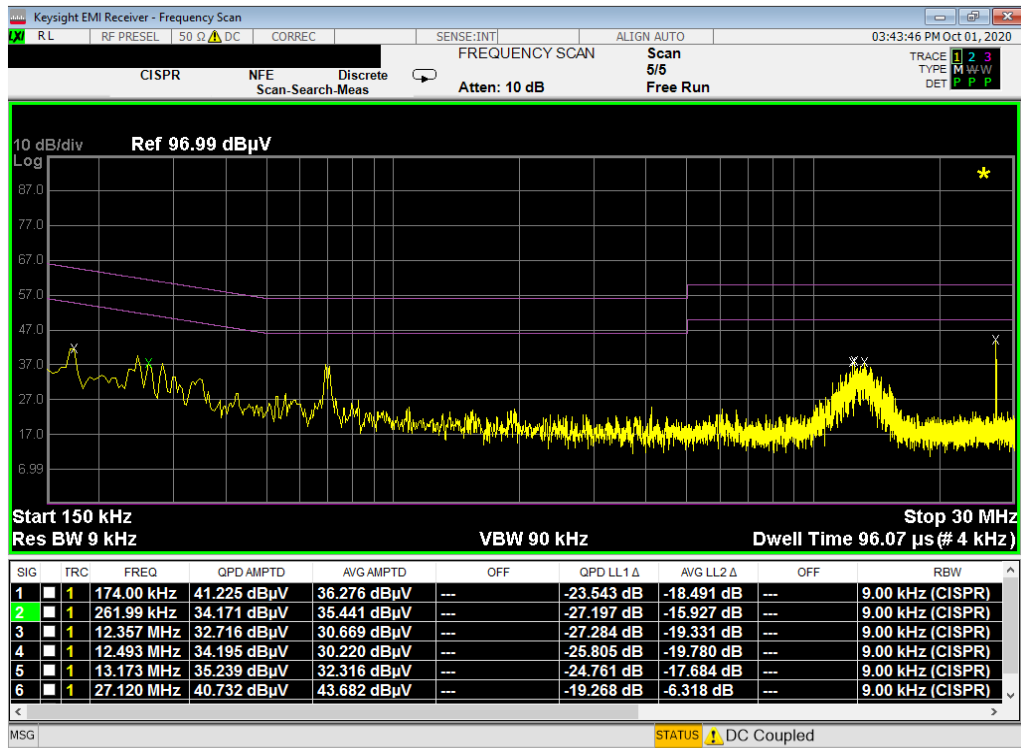
Plot 7-353. Line Conducted Plot with 802.11a UNII Band 1 (L1)
