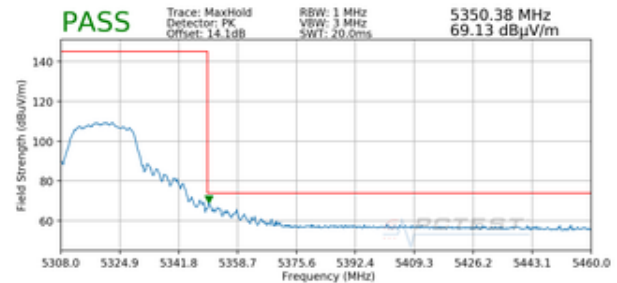
Plot 7-334. Radiated Upper Band Edge Plot MIMO (Peak – UNII Band 2A)
