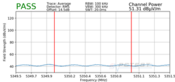
Plot 7-347. Radiated Upper Band Edge Plot MIMO (Average – UNII Band 2A)
