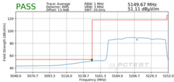
Plot 7-303. Radiated Lower Band Edge Plot SISO ANT1 (Average – UNII Band 1)
