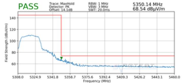
Plot 7-313. Radiated Upper Band Edge Plot SISO ANT2 (Peak – UNII Band 2A)
