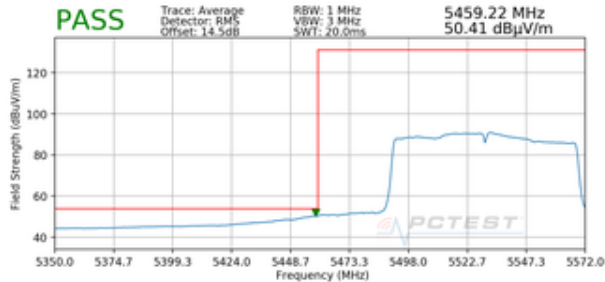
Plot 7-328. Radiated Lower Band Edge Plot SISO ANT2 (Average - UNII Band 2C)
