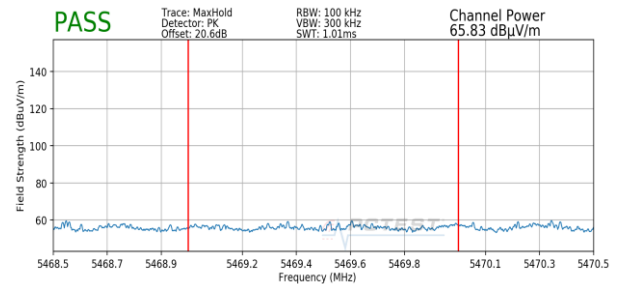
Plot 7-322. Radiated Lower Band Edge Plot SISO ANT2 (Peak – UNII Band 2C)
