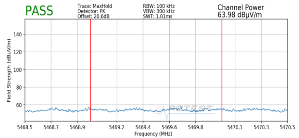
Plot 7-350. Radiated Lower Band Edge Plot MIMO (Peak – UNII Band 2C)
