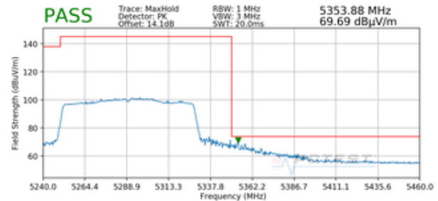
Plot 7-327. Radiated Upper Band Edge Plot SISO ANT2 (Peak – UNII Band 2A)
