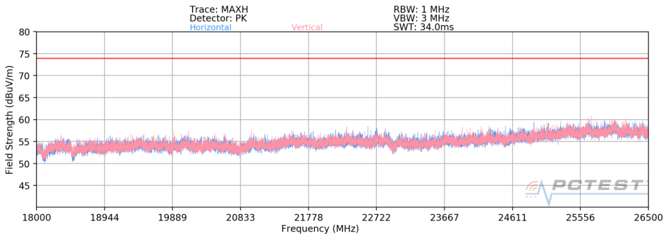
Plot 7-287. Radiated Spurious Plot 18GHz – 26.5GHz (Dual Band Simult. Tx)
