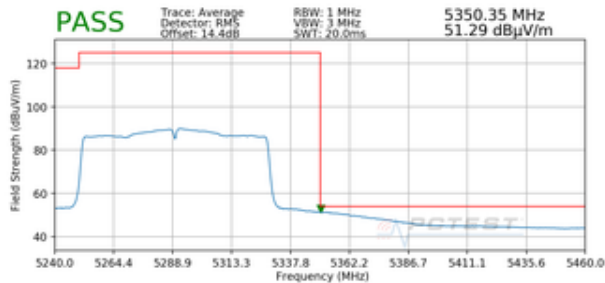
Plot 7-305. Radiated Upper Band Edge Plot SISO ANT1 (Average – UNII Band 2A)
