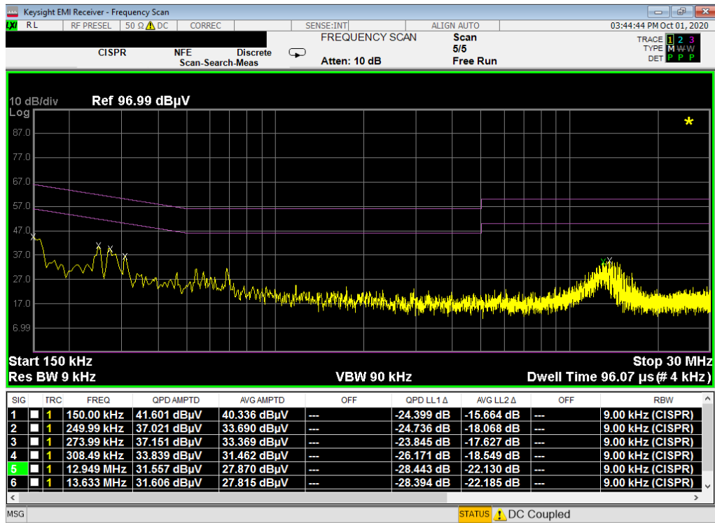
Plot 7-354. Line Conducted Plot with 802.11a UNII Band 1 (N)
