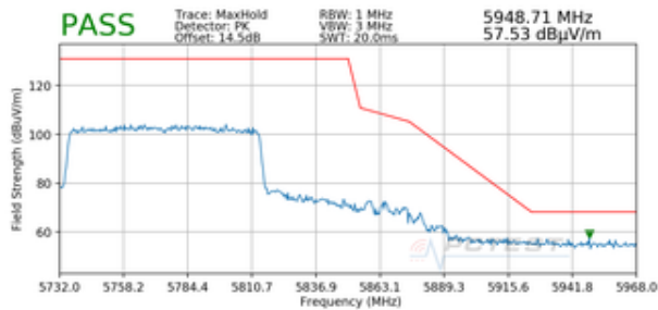
Plot 7-330. Radiated Upper Band Edge Plot SISO ANT2 (Peak - UNII Band 3)
