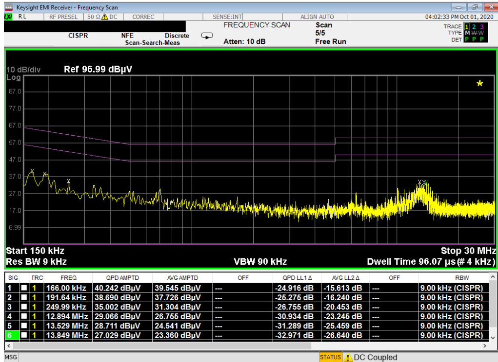
Plot 7-356. Line Conducted Plot with 802.11a UNII Band 2A (N)
