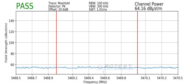
Plot 7-308. Radiated Lower Band Edge Plot SISO ANT1 (Peak – UNII Band 2C)
