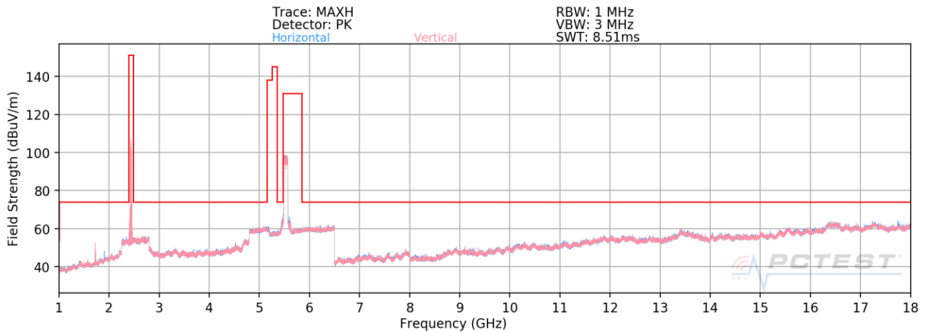
Plot 7-286. Radiated Spurious Plot above 1GHz (Dual Band Simult. Tx)
