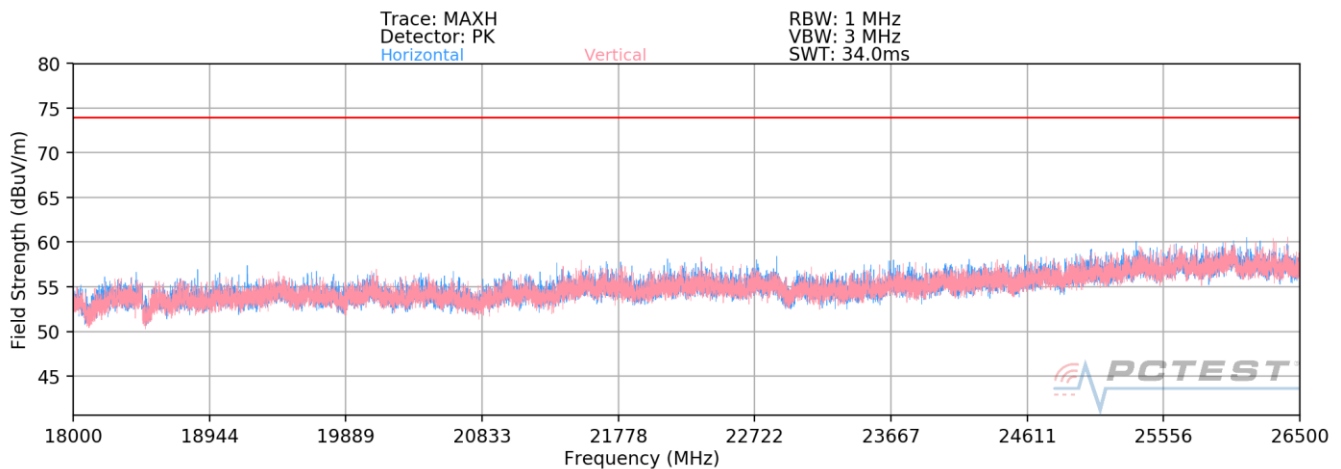
Plot 7-284. Radiated Spurious Plot 18GHz – 26.5GHz (5GHz – 2.4 GHz)
