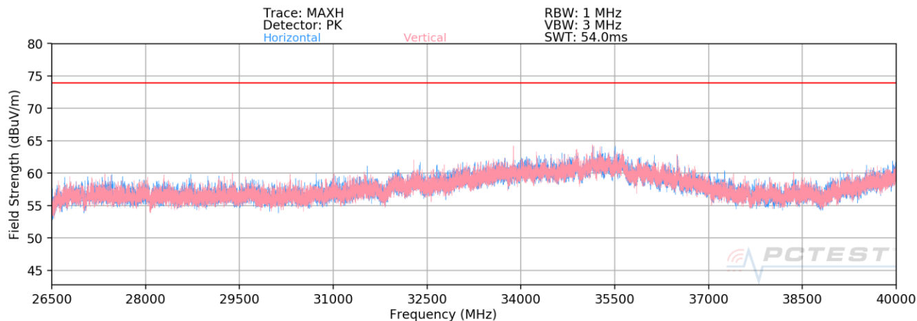
Plot 7-285. Radiated Spurious Plot above 26.5GHz (5GHz – 2.4 GHz)
