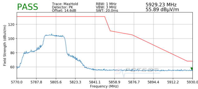
Plot 7-344. Radiated Upper Band Edge Plot MIMO (Peak – UNII Band 3)
