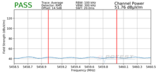
Plot 7-307. Radiated Lower Band Edge Plot SISO ANT1 (Average – UNII Band 2C)
