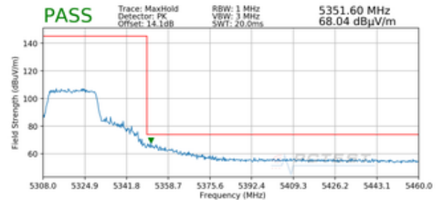
Plot 7-292. Radiated Upper Band Edge Plot SISO ANT1 (Peak – UNII Band 2A)
