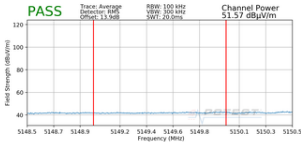
Plot 7-324. Radiated Lower Band Edge Plot SISO ANT2 (Average – UNII Band 1)
