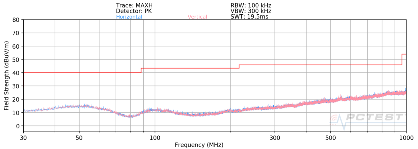
Plot 7-352. Radiated Spurious Plot below 1GHz
