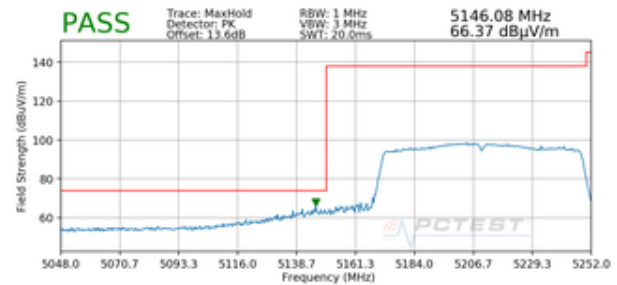
Plot 7-304. Radiated Lower Band Edge Plot SISO ANT1 (Peak – UNII Band 1)
