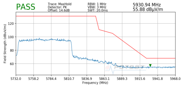
Plot 7-309. Radiated Upper Band Edge Plot SISO ANT1 (Peak – UNII Band 3)
