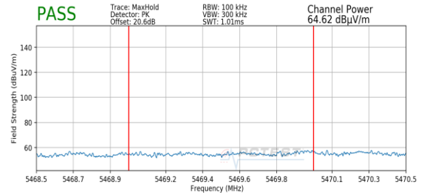
Plot 7-343. Radiated Lower Band Edge Plot MIMO (Peak – UNII Band 2C)
