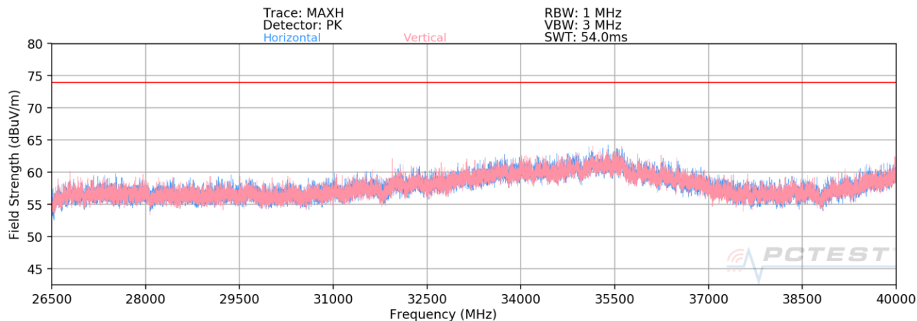
Plot 7-288. Radiated Spurious Plot above 26.5GHz (Dual Band Simult. Tx)
