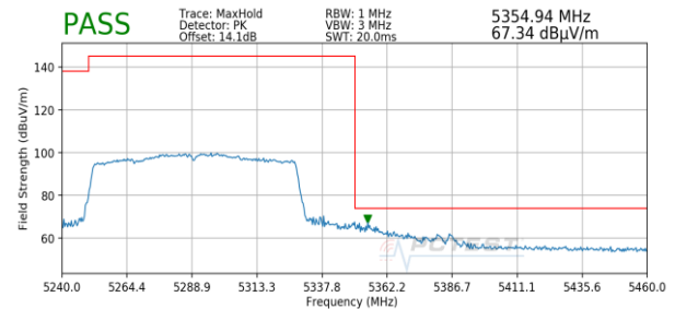
Plot 7-348. Radiated Upper Band Edge Plot MIMO (Peak – UNII Band 2A)
