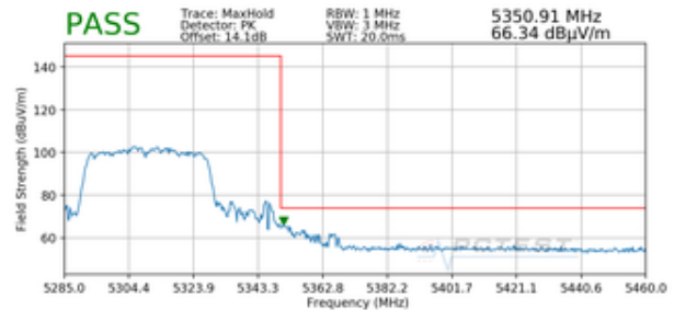
Plot 7-341. Radiated Upper Band Edge Plot MIMO (Peak – UNII Band 2A)
