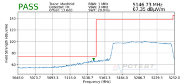
Plot 7-346. Radiated Lower Band Edge Plot MIMO (Peak – UNII Band 1)
