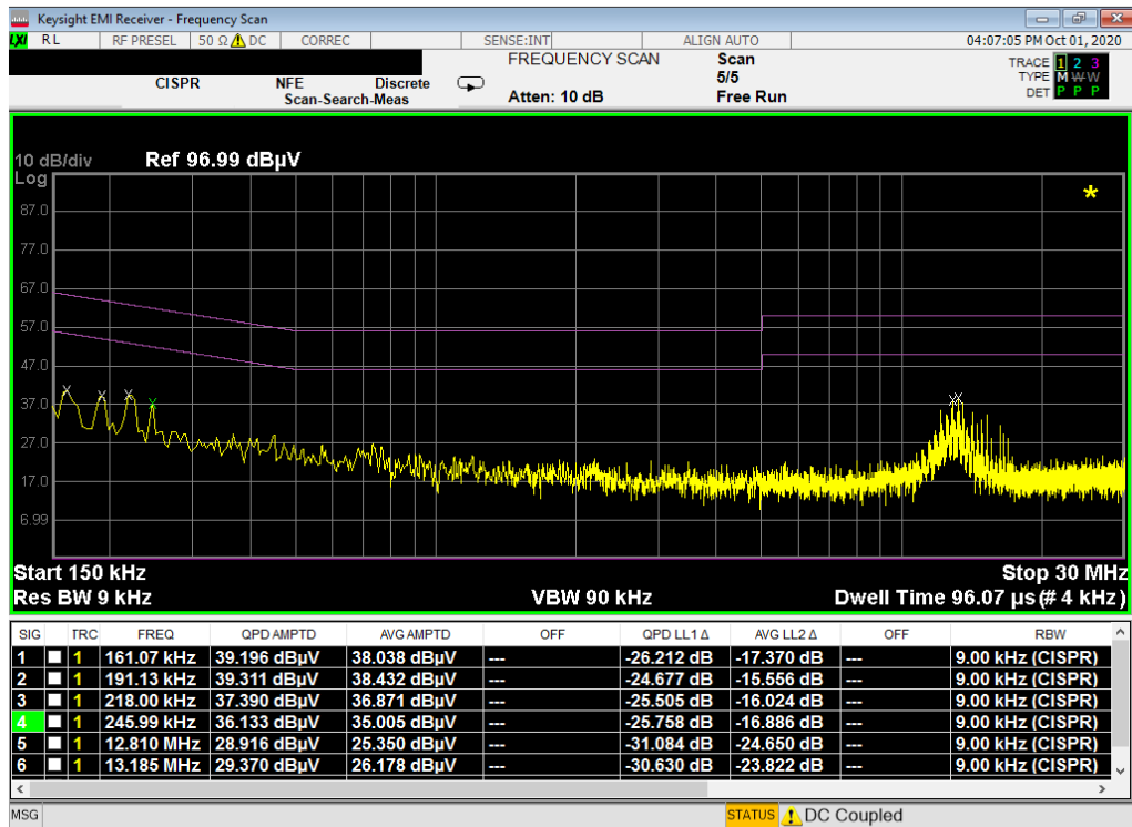
Plot 7-360. Line Conducted Plot with 802.11a UNII Band 3 (N)
