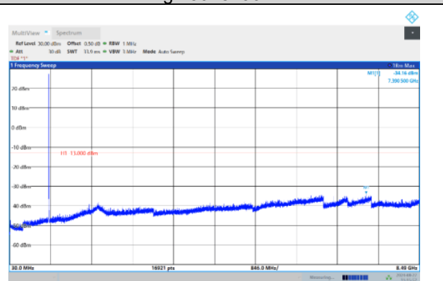
Band26-5MHz-16QAM-26815-1RB#0- Range:30~8490MHz
