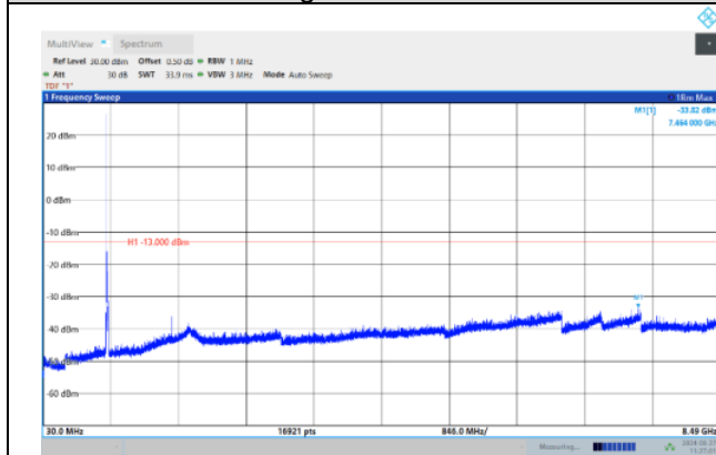
Band26-15MHz-16QAM-26915-1RB#0- Range:30~8490MHz
