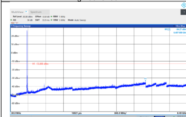
Band26-5MHz-QPSK-27015-1RB#0- Range:30~8490MHz
