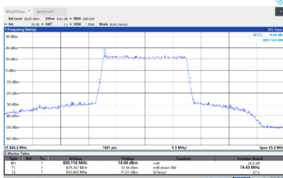
Band26-15MHz-64QAM-26915-75RB#0
