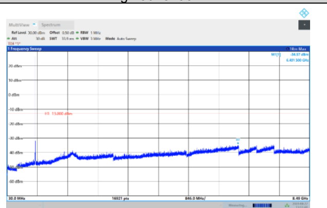
Band26-5MHz-QPSK-26915-1RB#0- Range:30~8490MHz
