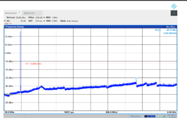
Band26-3MHz-64QAM-27025-1RB#0- Range:30~8490MHz
