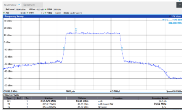
Band26-15MHz-64QAM-26865-75RB#0
