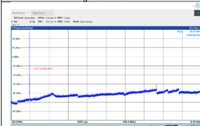
Band26-5MHz-QPSK-26815-1RB#0- Range:30~8490MHz
