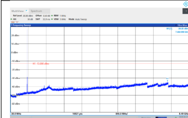
Band26-3MHz-64QAM-26915-1RB#0- Range:30~8490MHz
