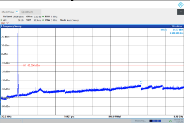
Band26-15MHz-16QAM-26965-1RB#0- Range:30~8490MHz
