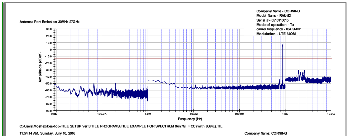
Figure 83. — 864.5 LTE 64QAM
