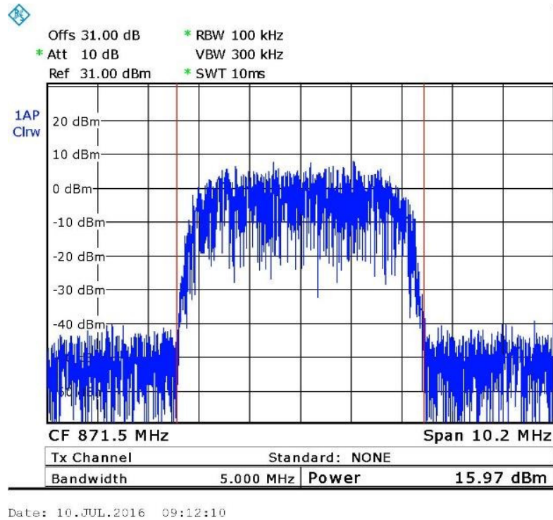
Figure 17. — W-CDMA - 871.5 MHz
