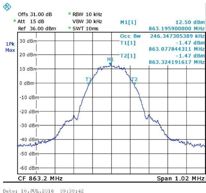
Figure 79. — 863.2MHz GSM Output
