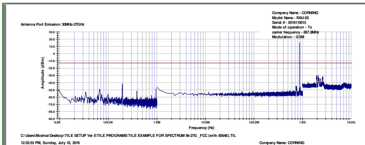
Figure 86. — 867.8 GSM
