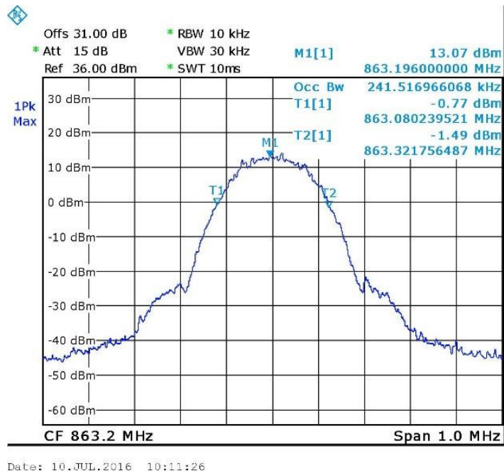
Figure 78. — 863.2MHz GSM Input
