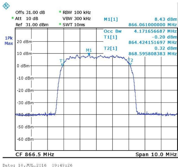
Figure 77. — 866.5MHz WCDMA Output
