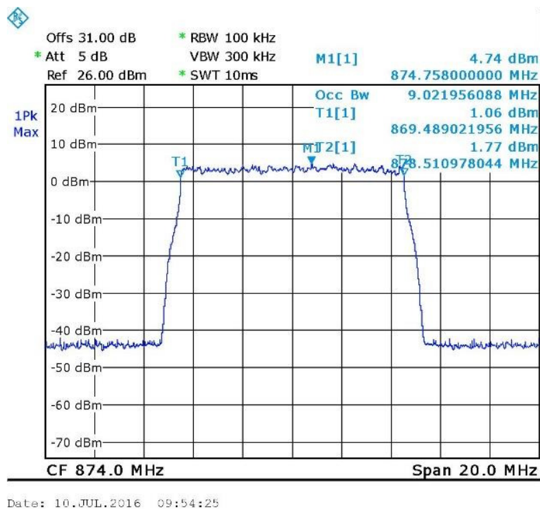
Figure 23. — LTE 64QAM Output 874.0MHz
