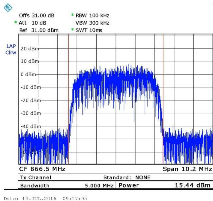
Figure 67. — 866.5 MHz – WCDMA
