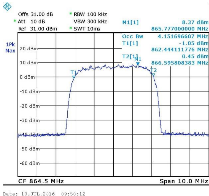
Figure 75. — 864.5MHz WCDMA Output
