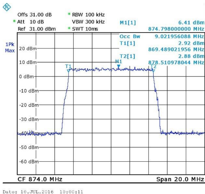
Figure 22. — LTE 64QAM Input 874.0MHz
