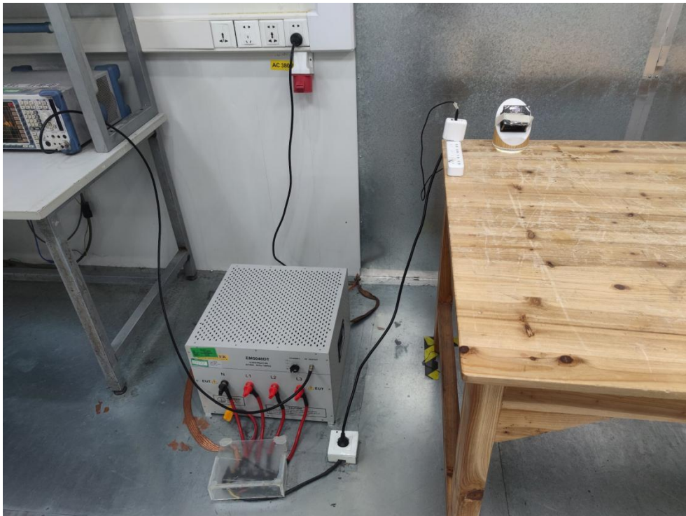
WPT Photo of Conducted Emission Measurement
