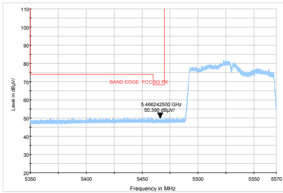
802.11ac VHT80 –Channel 106: Peak
