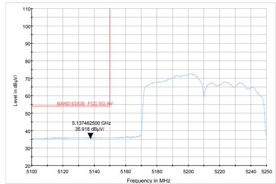
802.11ac VHT80- Channel 42: Average
