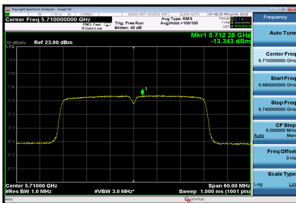
U-NII-2C, 802.11n HT40, Channel No.: 142
