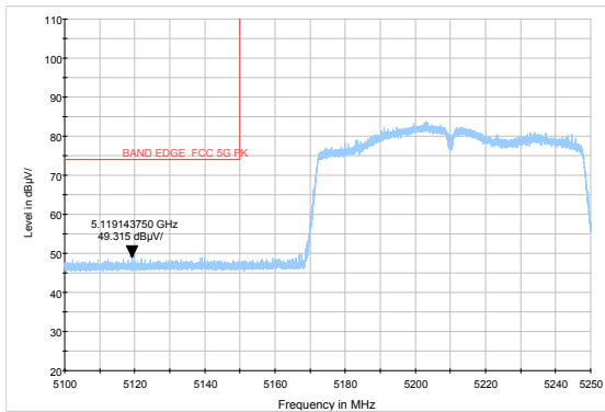
802.11ac VHT80 -Channel 42: Peak
