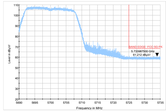
802.11a-Channel 140: Peak
