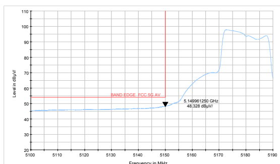
802.11a-Channel 36: Average
