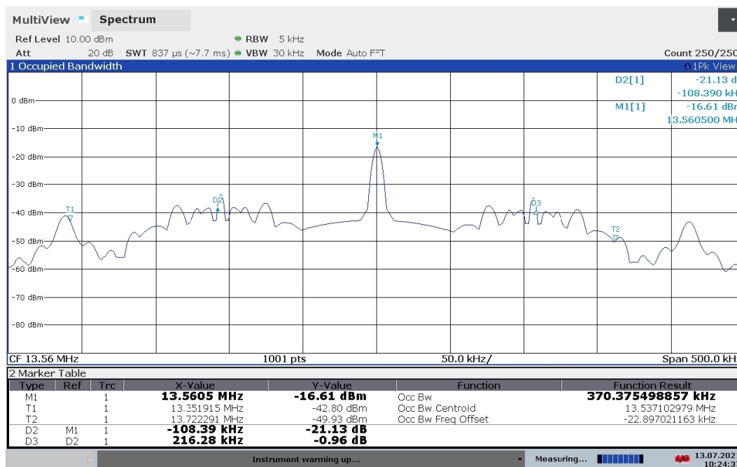
Figure 6: Intentional Emission Bandwidth.
