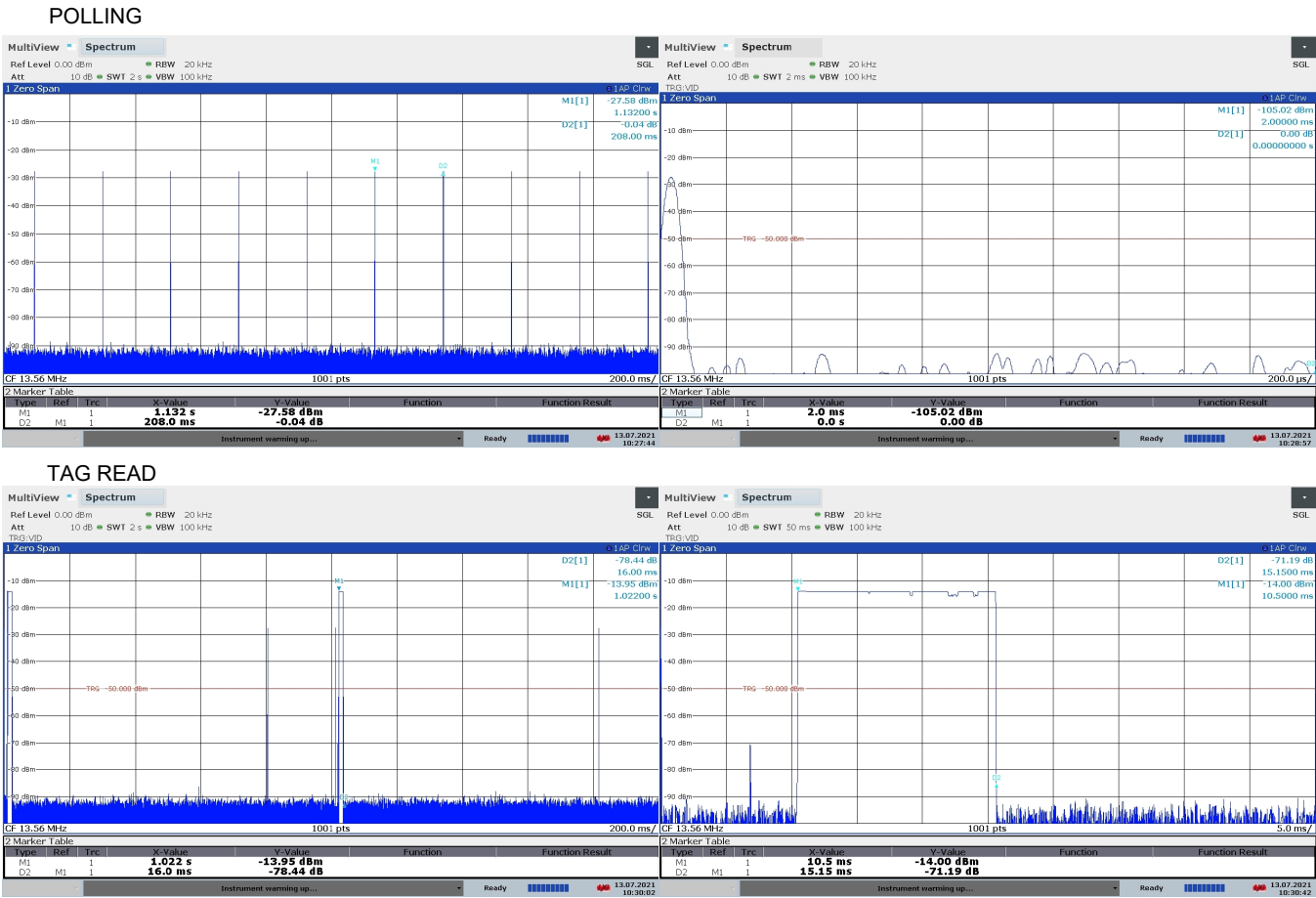
Figure 5: Pulsed Emission Characteristics (Duty Cycle).
