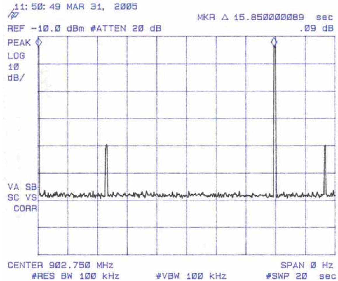
Figure 4-11. Occupancy Time, 50 Tags: 20sec Sweep Time
