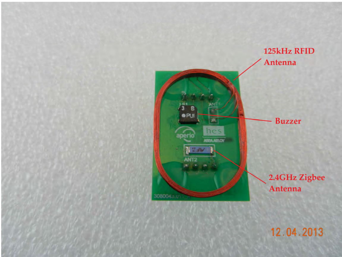
Antenna board
