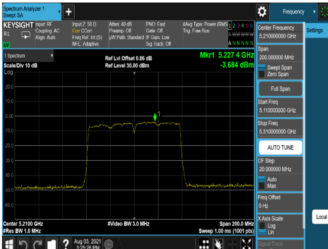
Plot 7-305. ISED PSD Antenna 5T (80MHz BW 11ac - Ch.42, MCS5)
