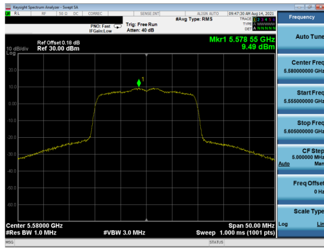
Plot 7-320. PSD Antenna 3b (20MHz BW 802.11ax(SU) – Ch. 116, MCS2)
