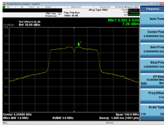
Plot 7-321. PSD Antenna 3b (40MHz BW 802.11n – Ch. 110, MCS2)
