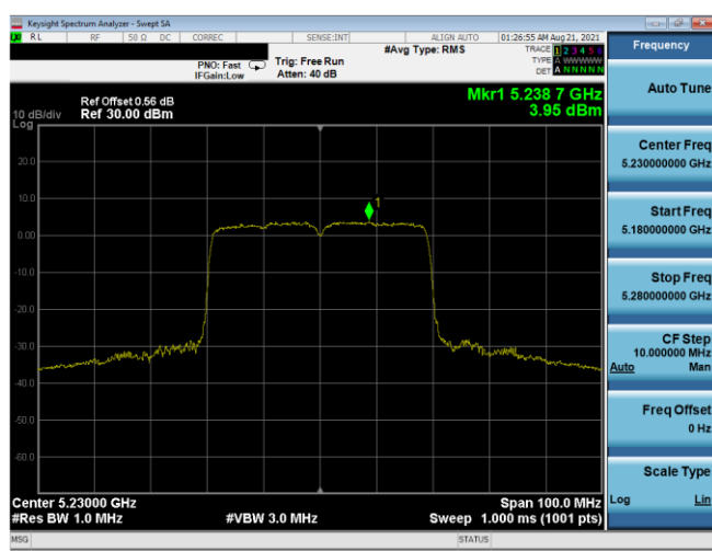
Plot 7-304. ISED PSD Antenna 5T (40MHz BW 11ax(SU) - Ch.46, MCS5)
