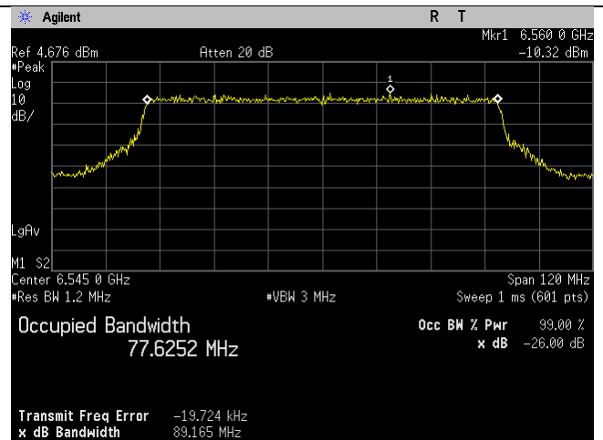
6545MHz_119_80MHz BW_be-mode_Chain 3
