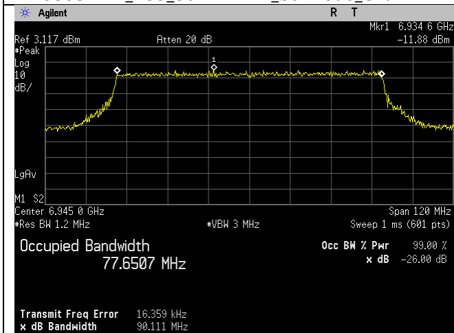
6945MHz_199_80MHz BW_be-mode_Chain 0
