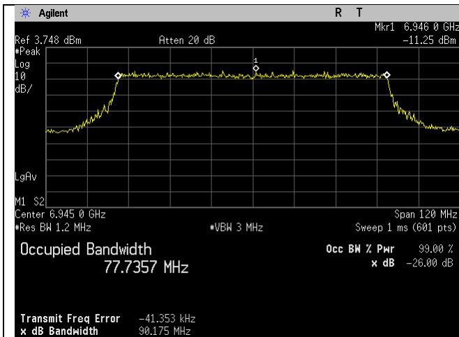
6945MHz_199_80MHz BW_be-mode_Chain 2
