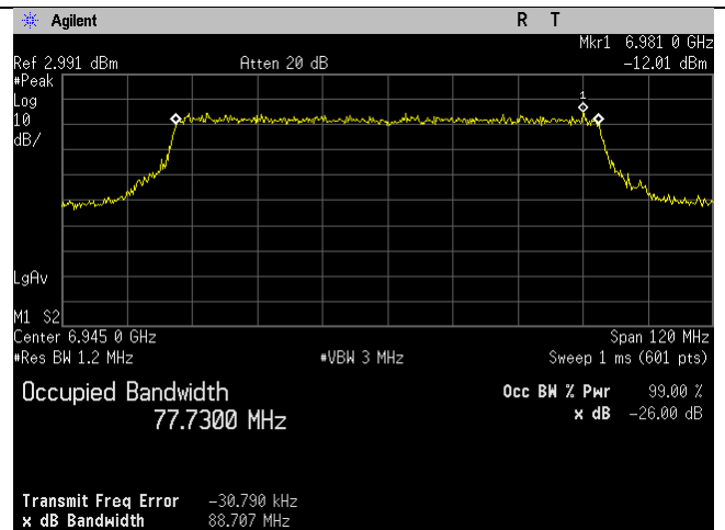
6945MHz_199_80MHz BW_be-mode_Chain 3
