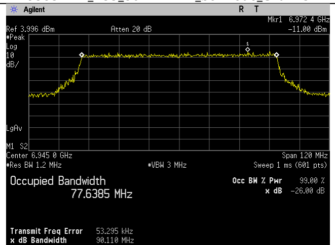
6945MHz_199_80MHz BW_be-mode_Chain 1
