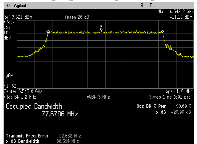
6545MHz_119_80MHz BW_be-mode_Chain 1
