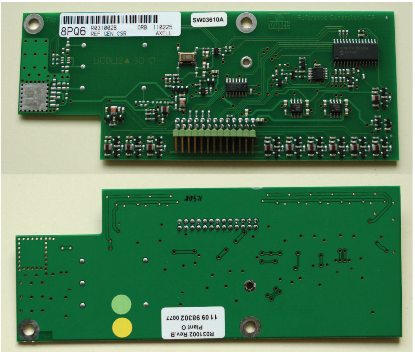
R031002B Reference Generator.
