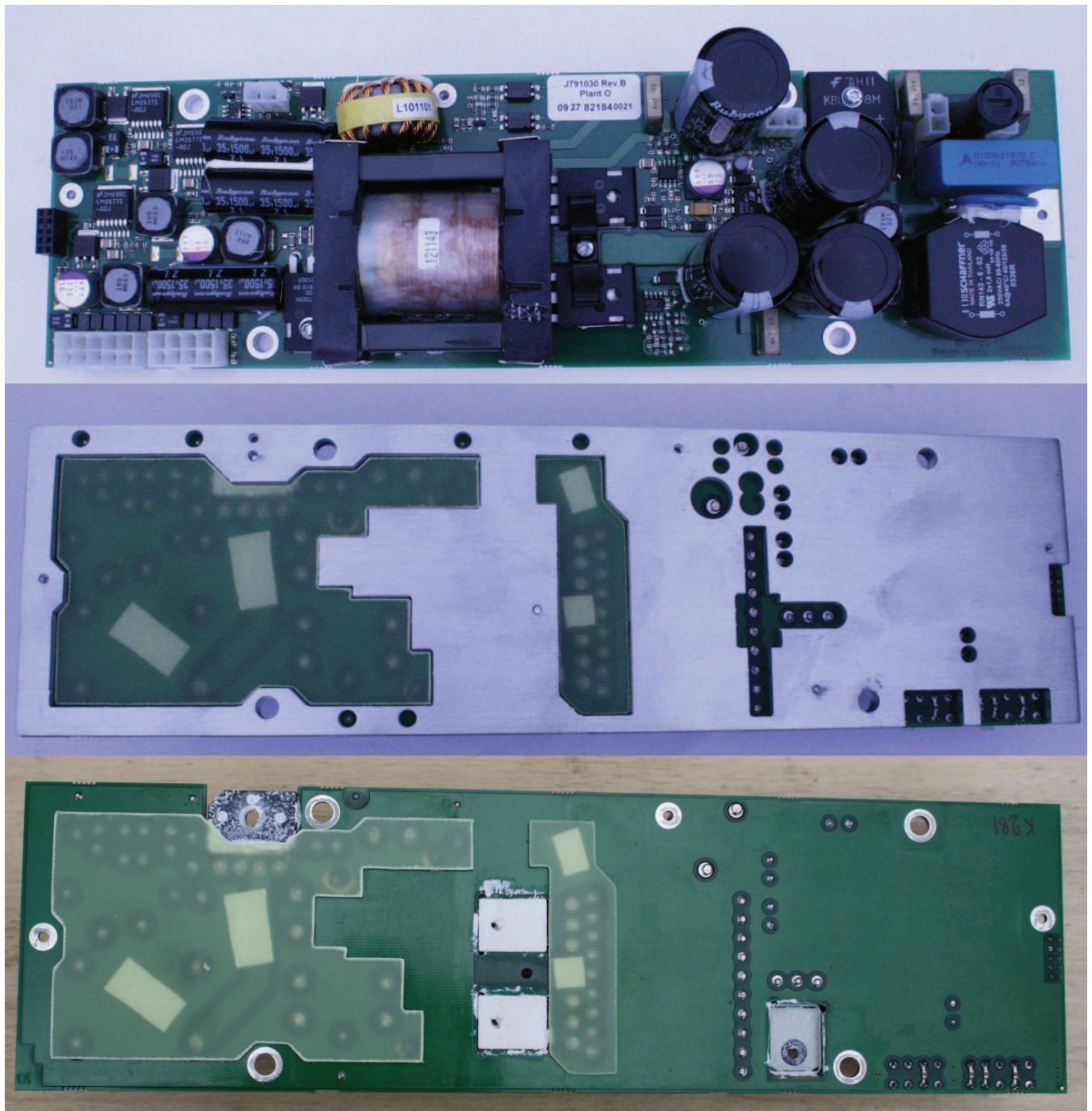
J791001 PSU
