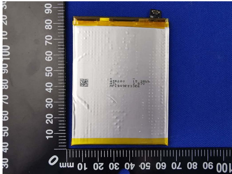
Battery Photo (FRONT) (Manufacturer: Dongguan NVT Technology Co., Ltd.)
