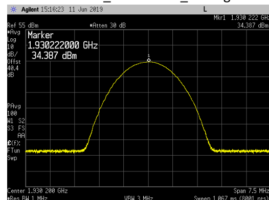
Bottom Channel_1930.2MHz_Average
