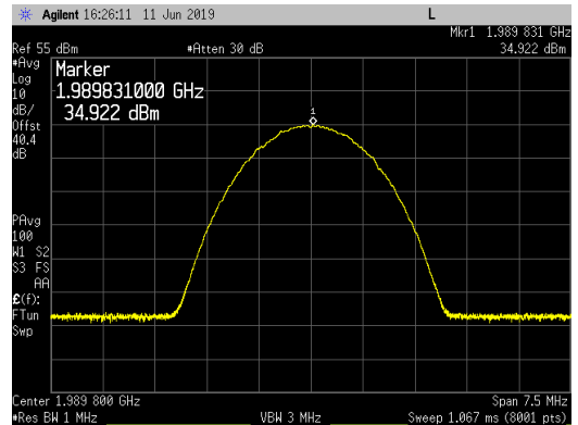
Top Channel_1989.8MHz_Average
