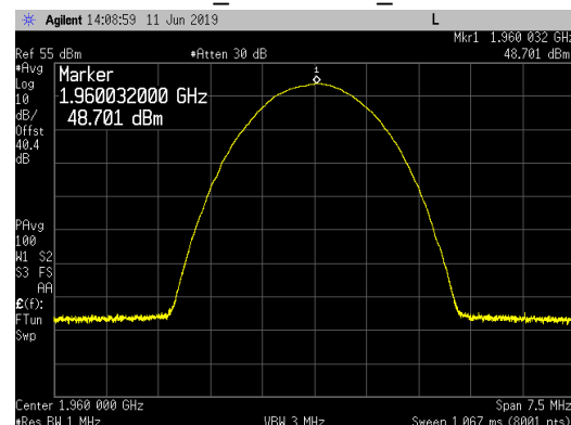
Middle Channel_1960.0MHz_Ave
