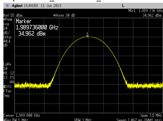
Top Channel_1989.8MHz_Peak
