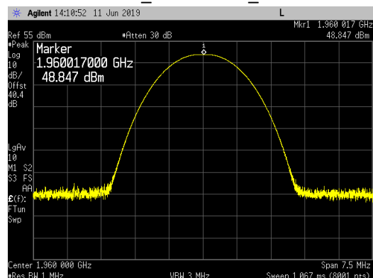
Middle Channel_1960.0MHz_Peak
