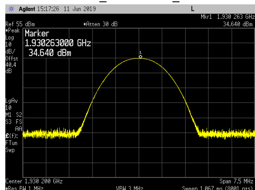
Bottom Channel_1930.2MHz_Peak
