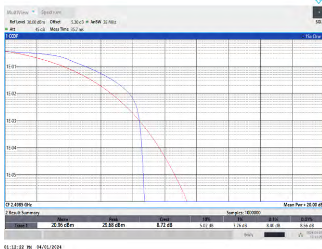
Band41-5MHz-QPSK-39675-25RB#0
