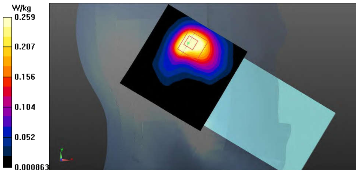
Fig.27 WLAN 2.4GHz Head
