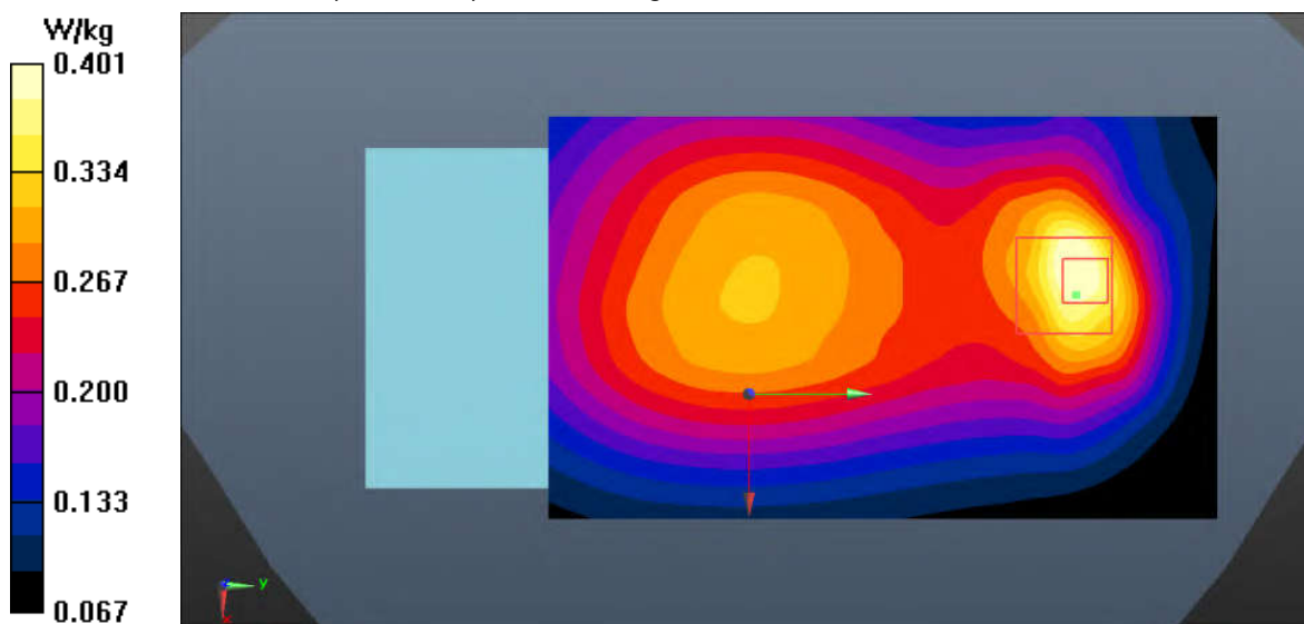
Fig.22 LTE Band 28 Body
