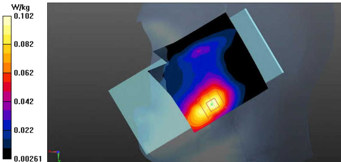
Fig.15 LTE Band 7 Head
