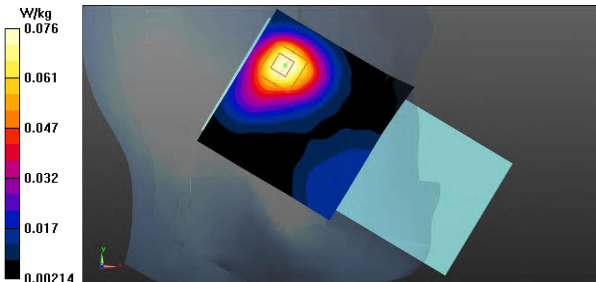
Fig.3 PCS1900 Head
