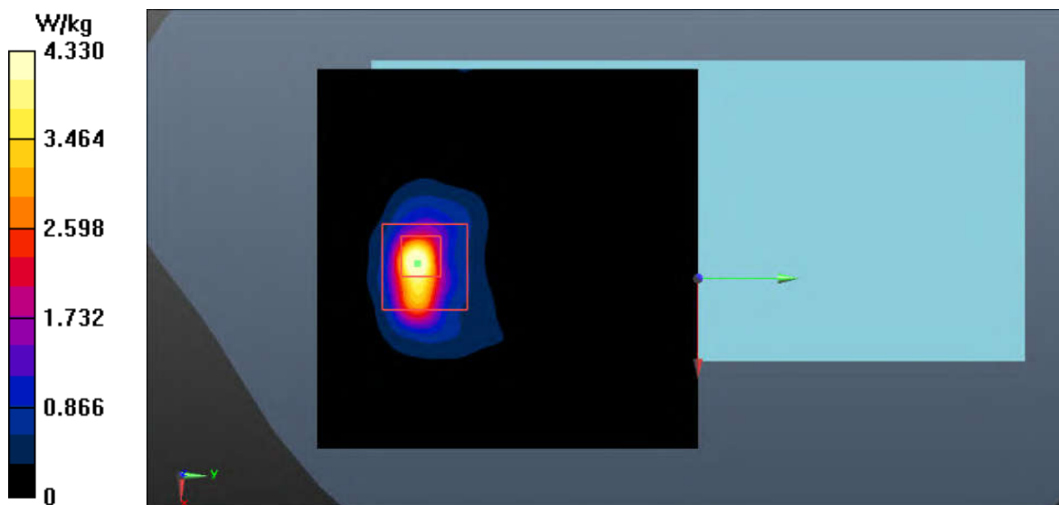
Fig.31 WLAN 5GHz Extremity
