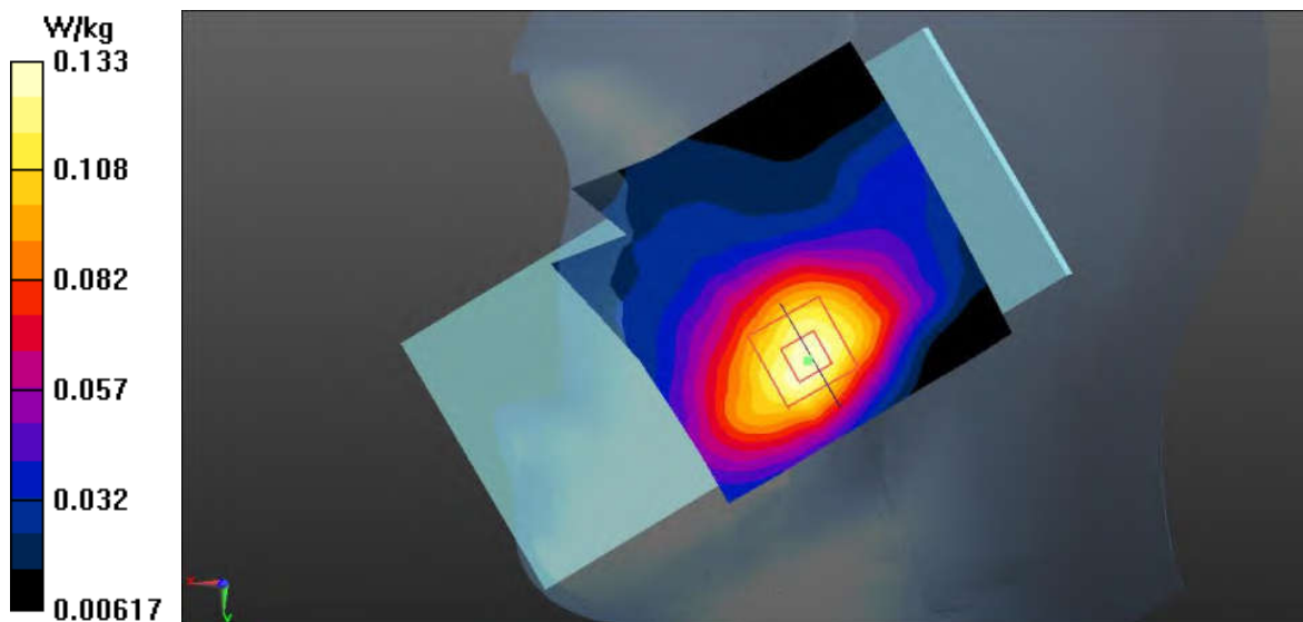
Fig.23 LTE Band 66 Head
