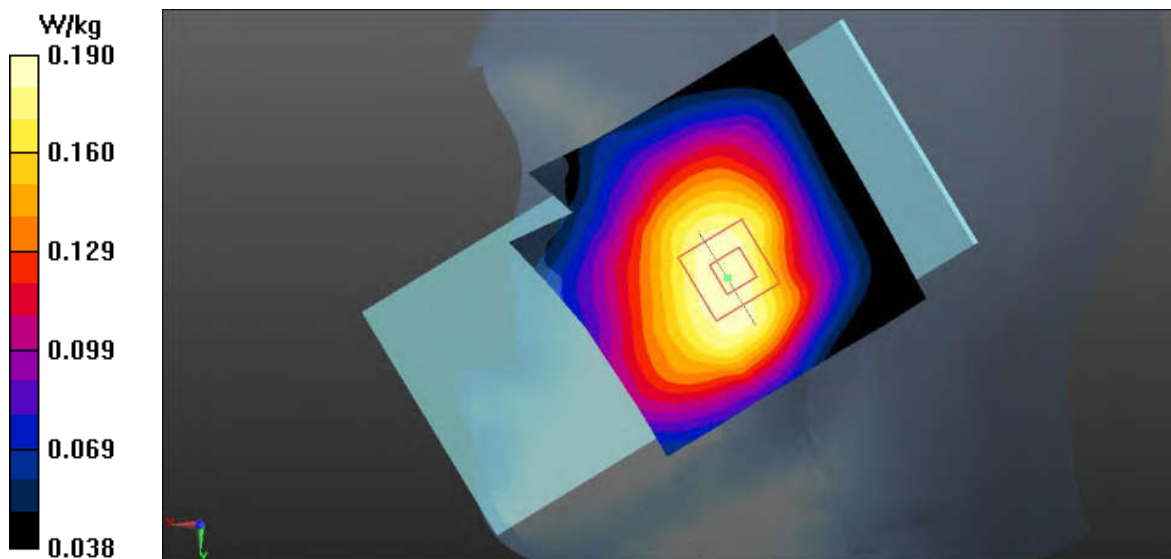
Fig.17 LTE Band 12 Head
