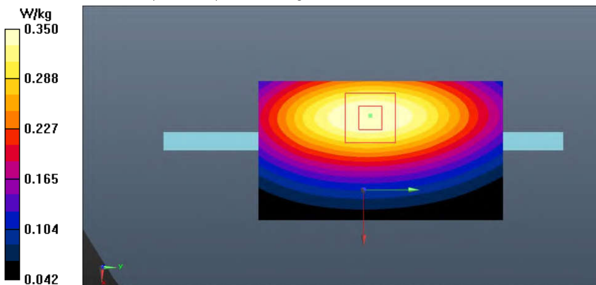
Fig.18 LTE Band 12 Body
