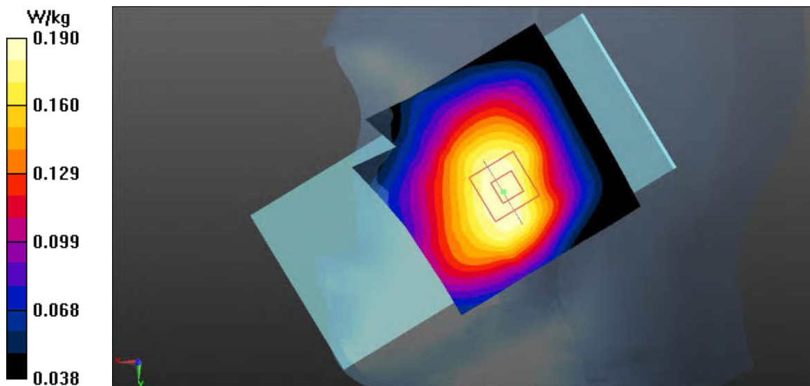
Fig.21 LTE Band 28 Head
