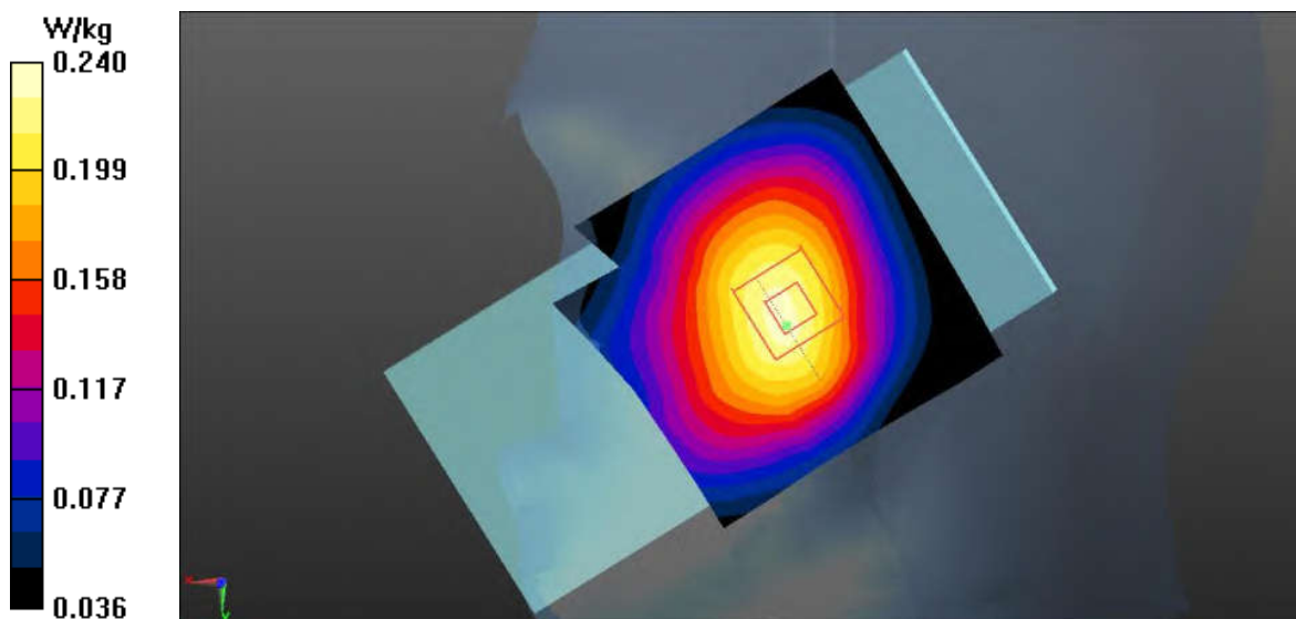
Fig.1 GSM850 Head
