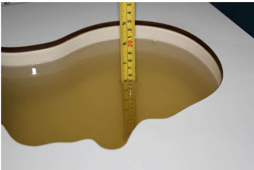
Picture 7-6: Liquid depth in the Head Phantom(2550MHz)
