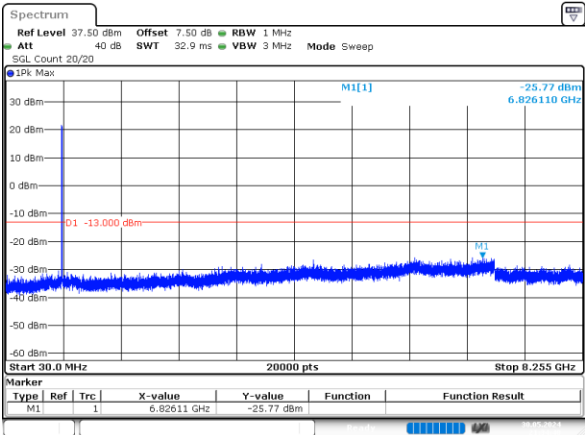
3MHz_Low_QPSK_15@0 -25.77dBm
