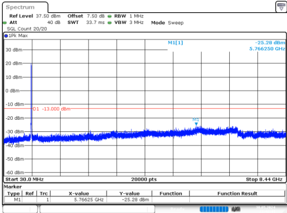
10MHz_High_QPSK_50@0 -25.28dBm
