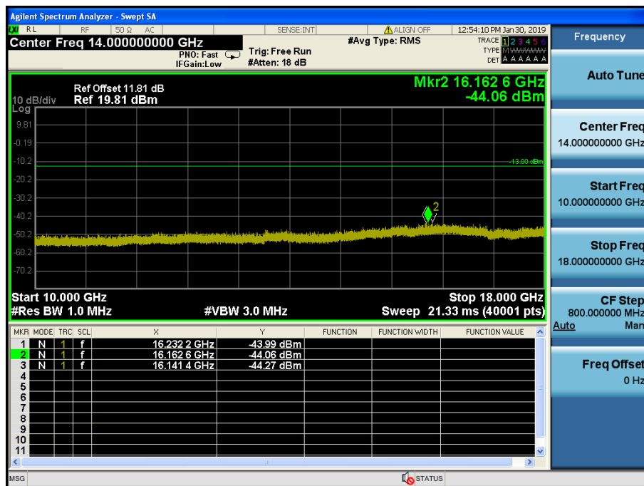
LTE Band 66 / 20MHz / 16QAM - RB Size/Offset (50/0) –Mid Channel
