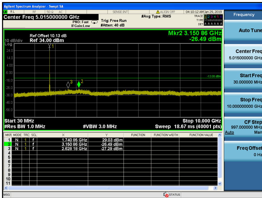
LTE Band 66 / 10MHz / QPSK - RB Size/Offset (1/0) – Mid Channel
