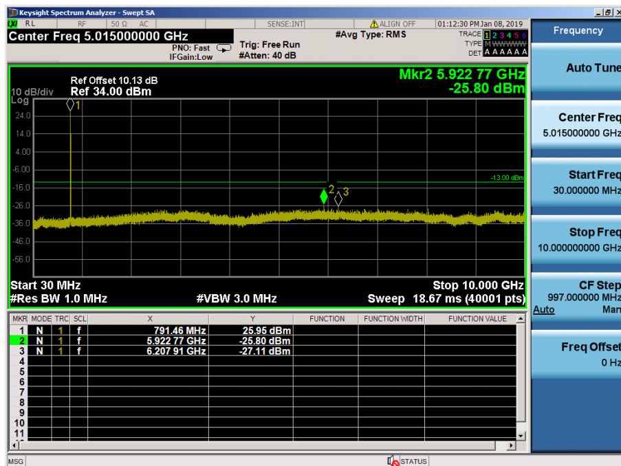
LTE Band 14 / 5MHz / QPSK - RB Size/Offset (12/13) – Low Channel
