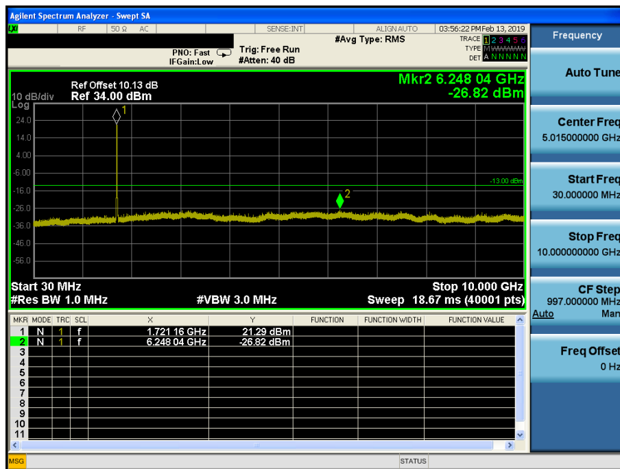
LTE Band 66 / 20MHz / 16QAM - RB Size/Offset (50/25) –Low Channel
