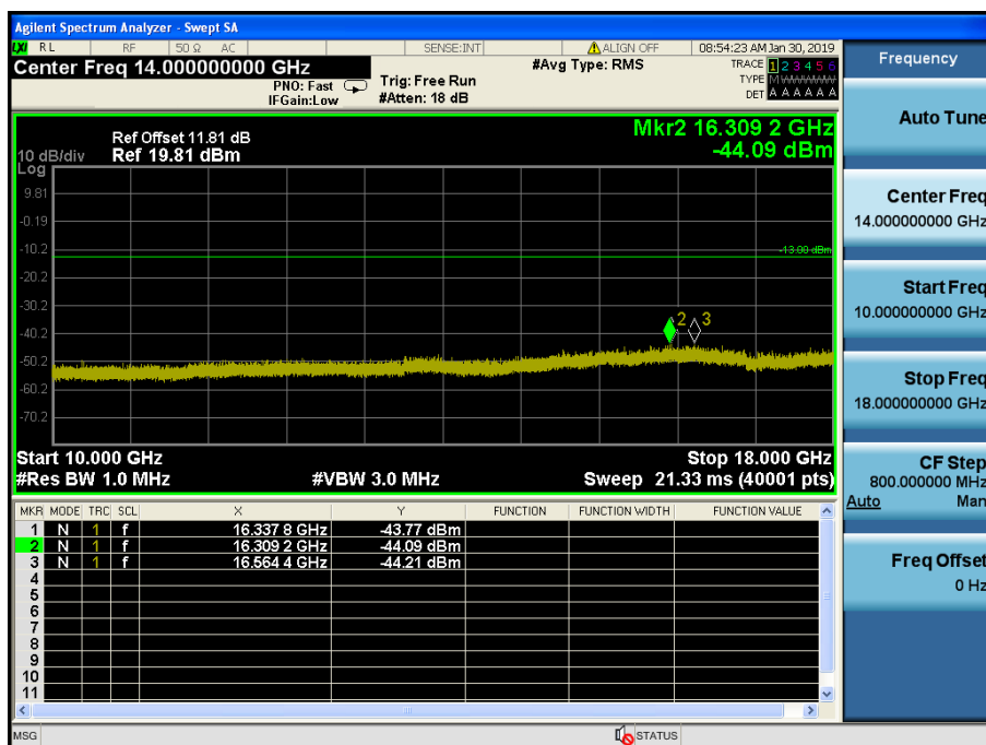
LTE Band 66 / 15MHz / 16QAM- RB Size/Offset (1/74) – Mid Channel
