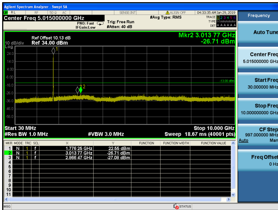
LTE Band 66 / 10MHz / QPSK - RB Size/Offset (50/0) – High Channel
