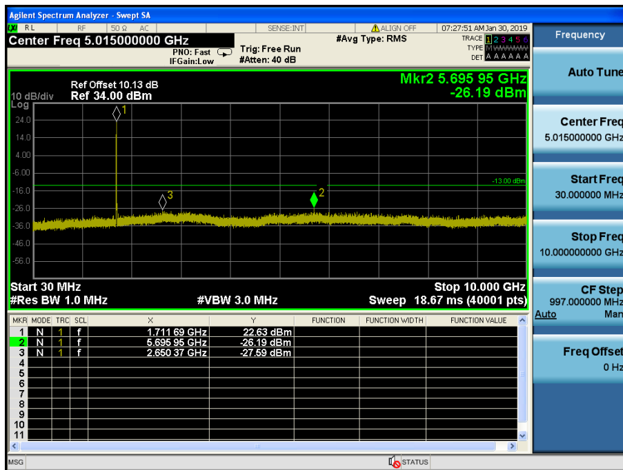
LTE Band 66 / 5MHz / 16QAM - RB Size/Offset (25/0) – Low Channel
