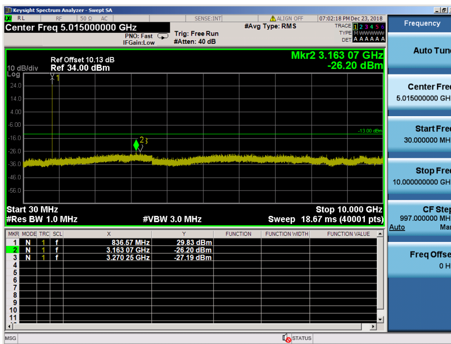
LTE Band 5 / 1.4MHz / QPSK - RB Size/Offset (3/0) – Mid Channel
