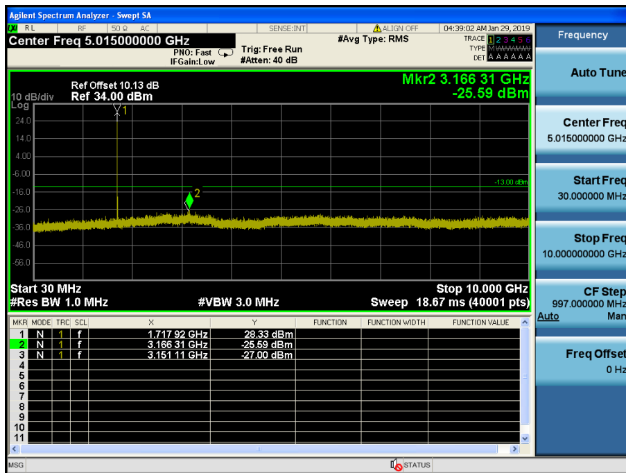
LTE Band 66 / 15MHz / QPSK - RB Size/Offset (1/36)–Low Channel
