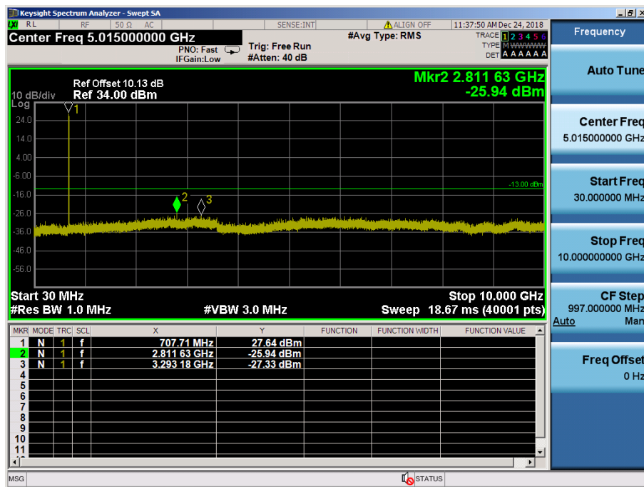
LTE Band 12 / 1.4MHz / QPSK - RB Size/Offset (6/0) – Mid Channel
