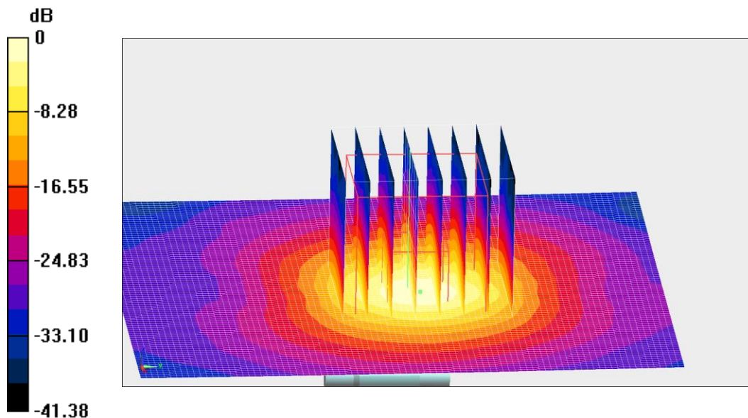
Fig.B.4 validation 5800 MHz 250mW
