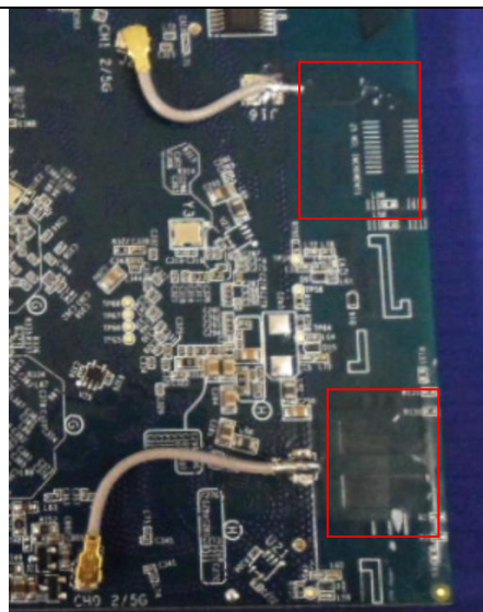
Antenna Location
