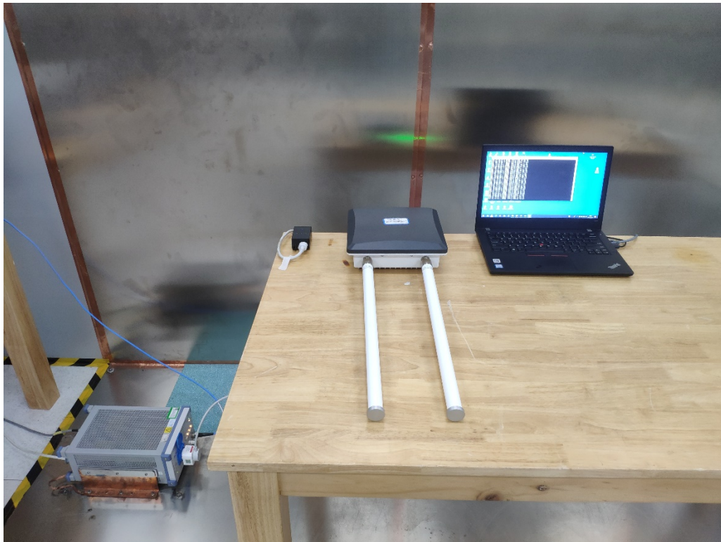
Photograph 2: Set-up for Co-Located Radiated Spurious Emissions, below 1GHz
