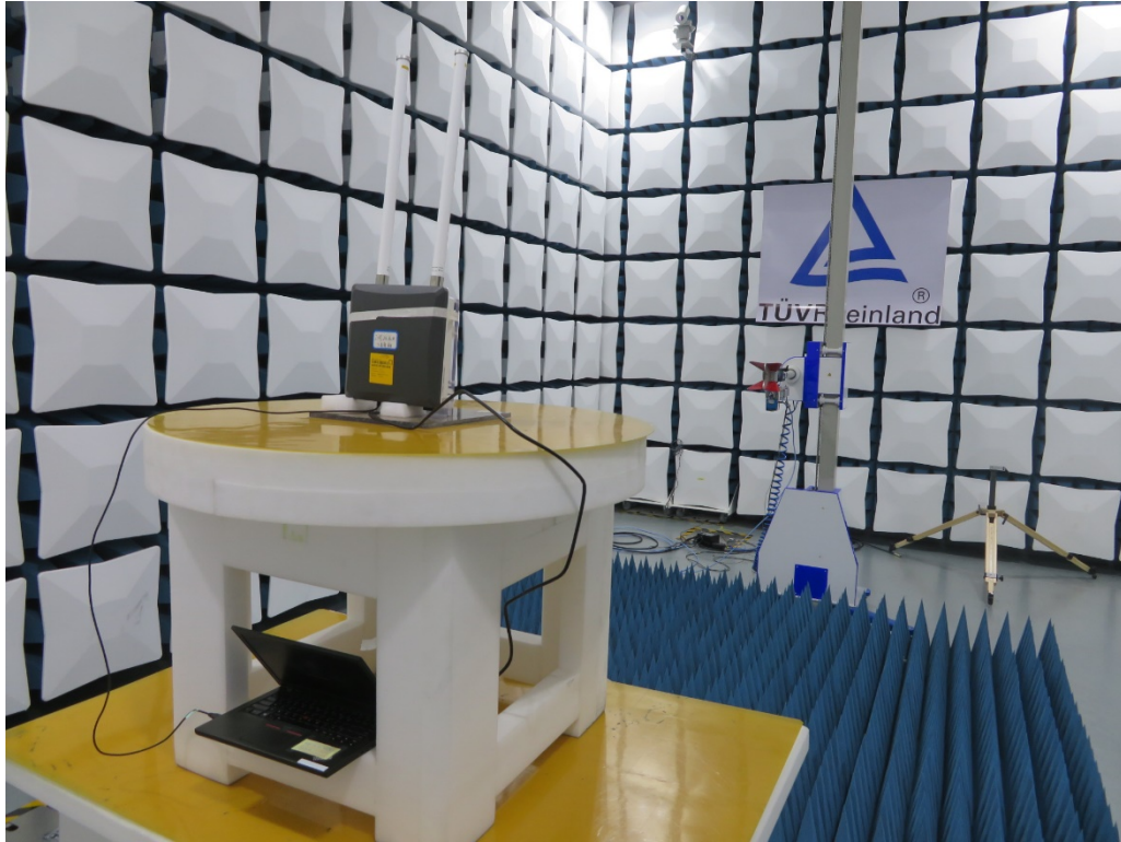
Photograph 3: Set-up for Co-Located Radiated Spurious Emissions, above 1GHz
