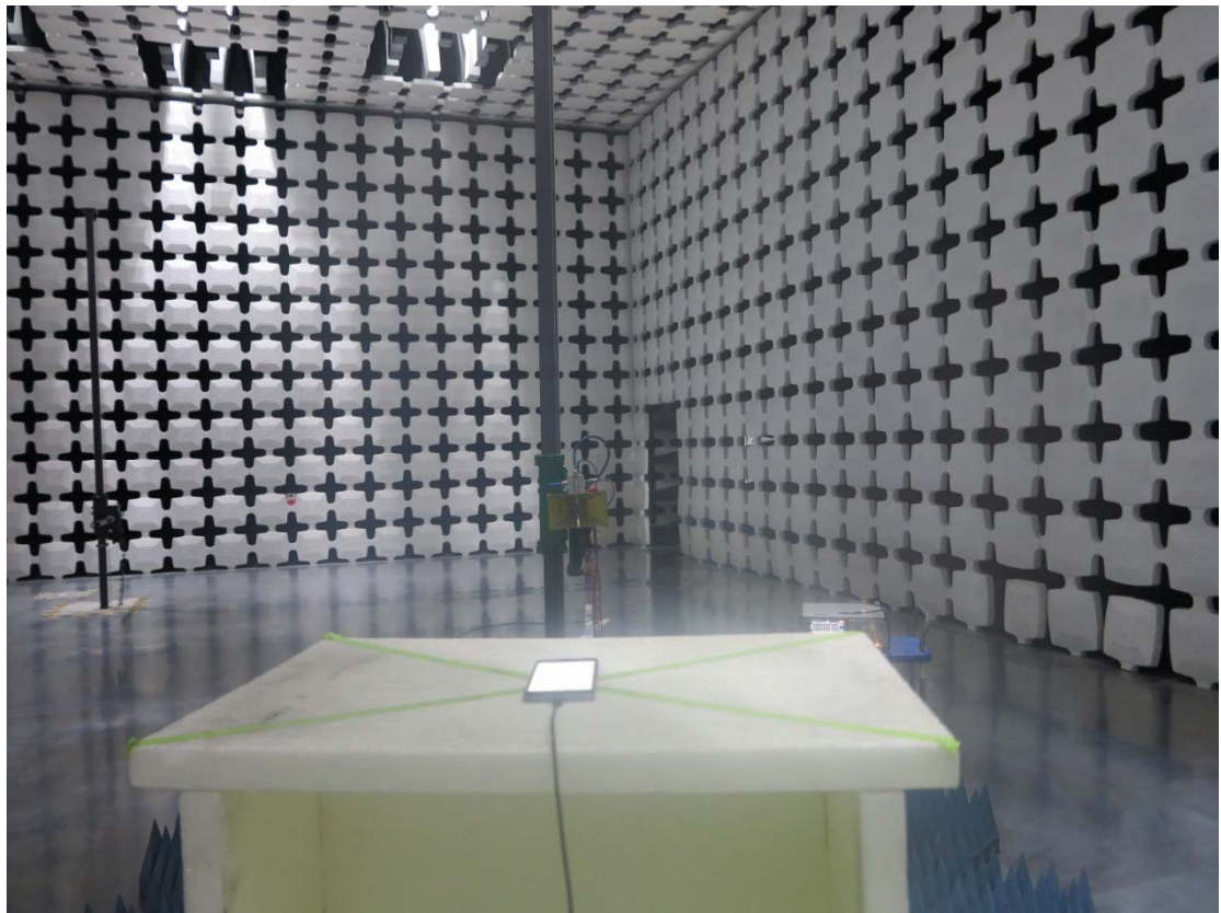
Spurious Emission
