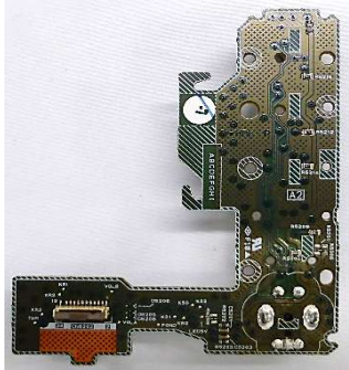
[TFT PCB / Solder Side] (Including BT)
