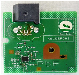
[KEY PCB / Solder Side]
