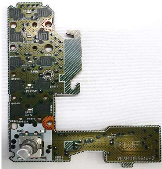
[TFT PCB / Surface Side] (Including BT)
