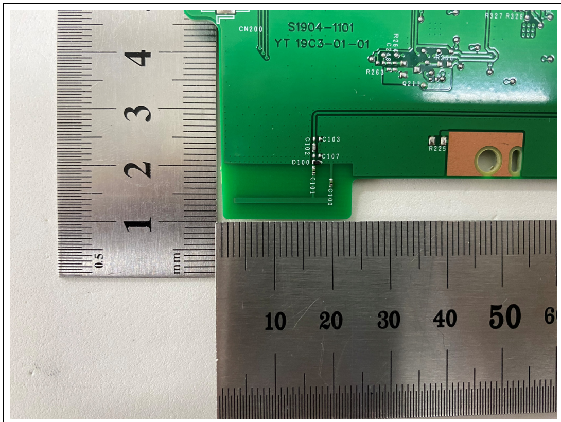
<BT Antenna>
