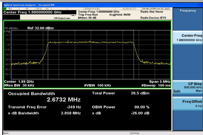
Band2-3MHz-16QAM-18900-15RB#0-2.6732
