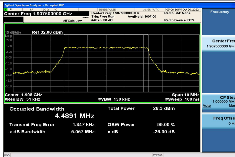
Band2-5MHz-QPSK-19175-25RB#0-4.4891
