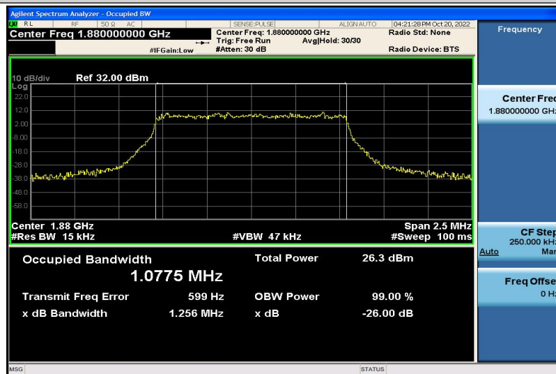
Band2-1.4MHz-16QAM-18900-6RB#0-1.0775
