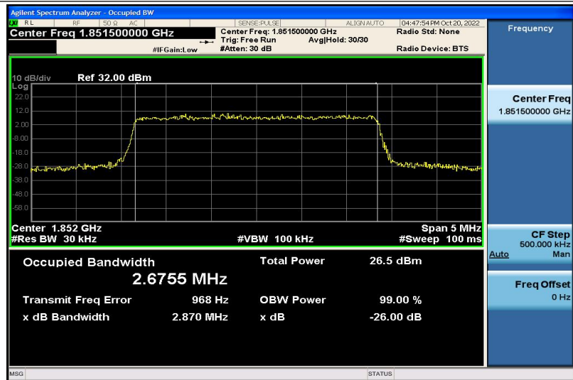
Band2-3MHz-16QAM-18615-15RB#0-2.6755
