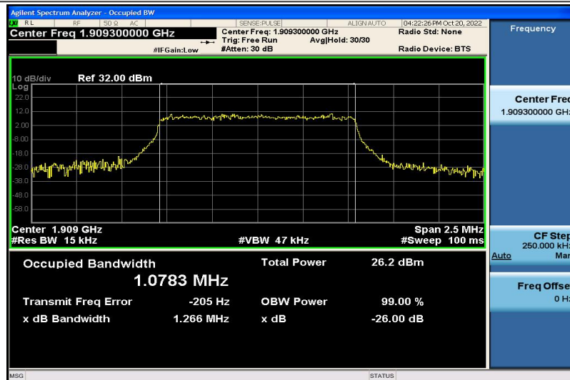
Band2-1.4MHz-16QAM-19193-6RB#0-1.0783
