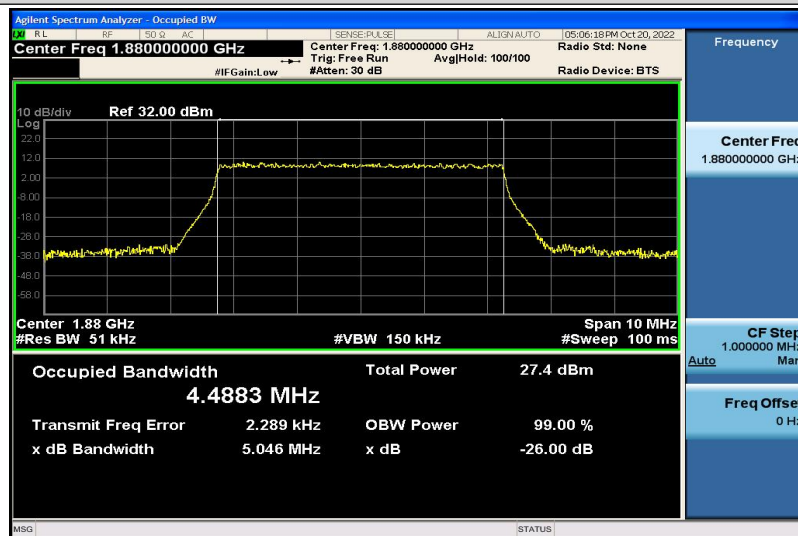
Band2-5MHz-16QAM-18900-25RB#0-4.4883
