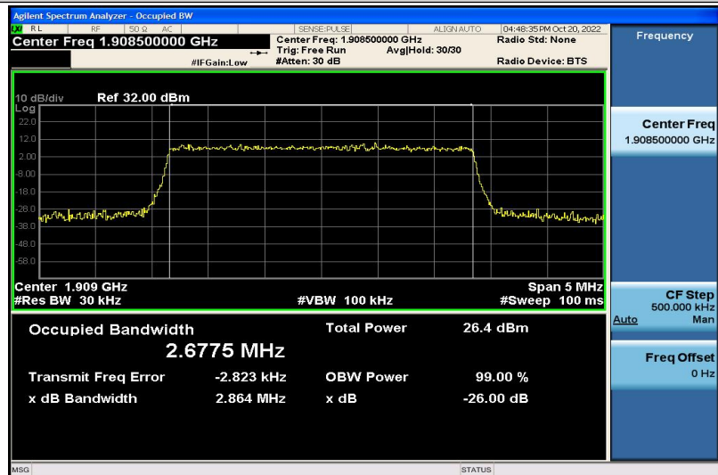
Band2-3MHz-16QAM-19185-15RB#0-2.6775
