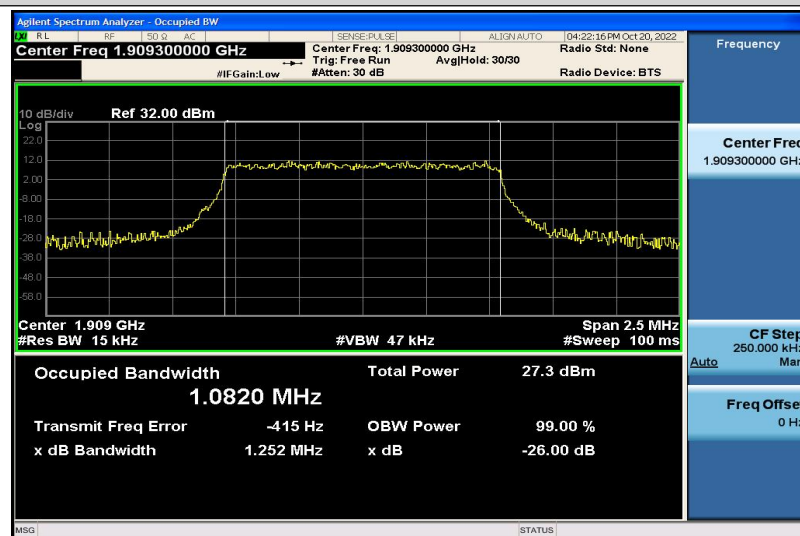
Band2-1.4MHz-QPSK-19193-6RB#0-1.0820
