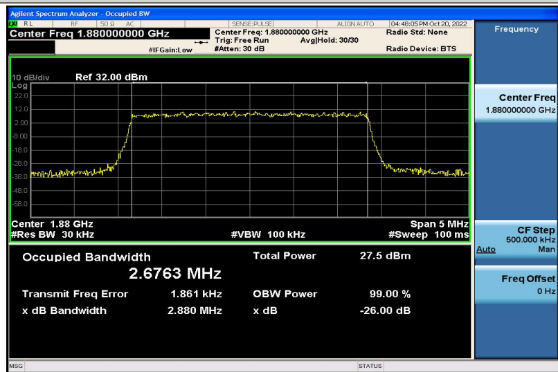
Band2-3MHz-QPSK-18900-15RB#0-2.6763
