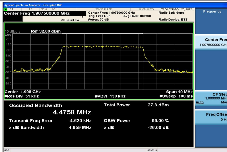
Band2-5MHz-16QAM-19175-25RB#0-4.4758
