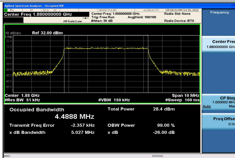
Band2-5MHz-QPSK-18900-25RB#0-4.4888
