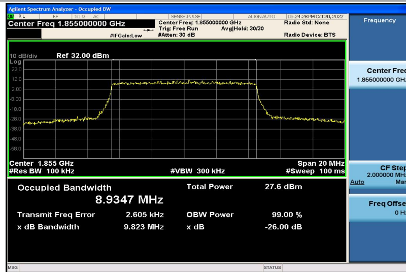
Band2-10MHz-QPSK-18650-50RB#0-8.9347
