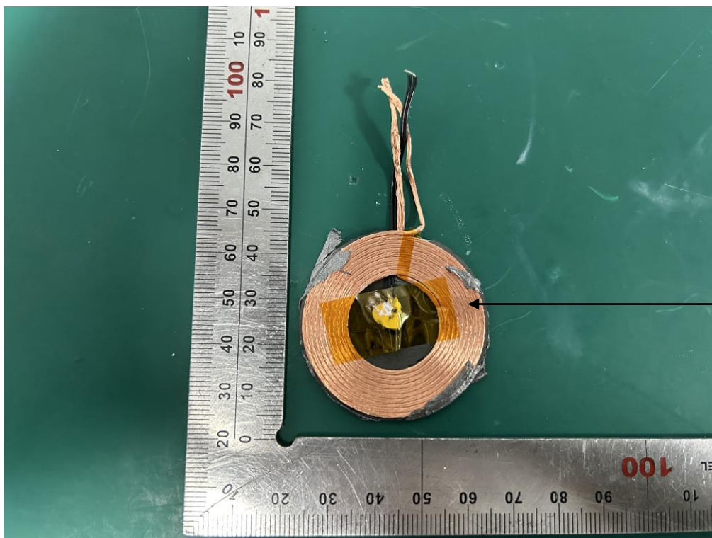
Coil Antenna
