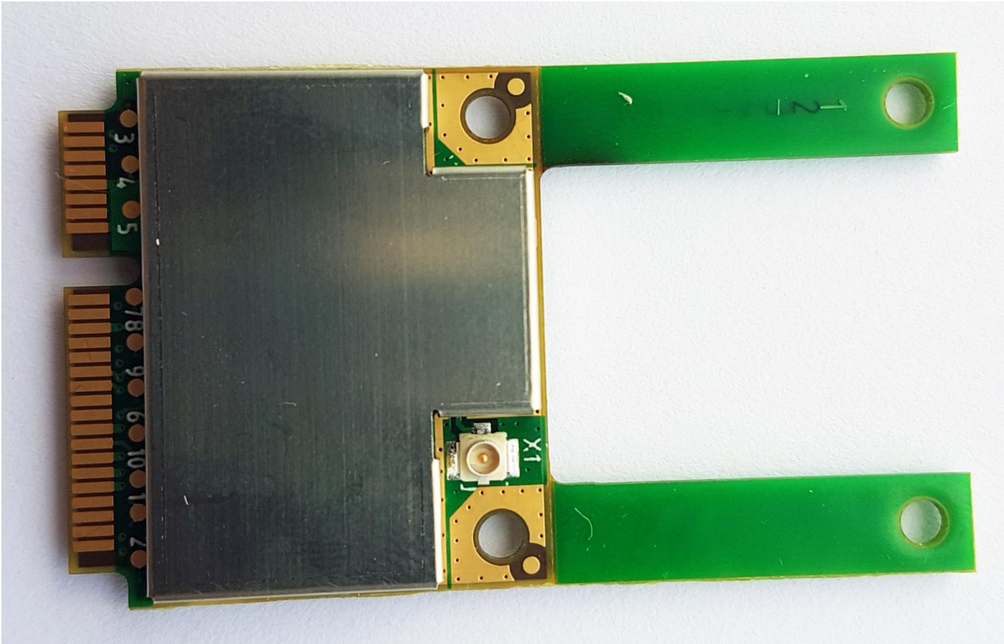
EUT top view
