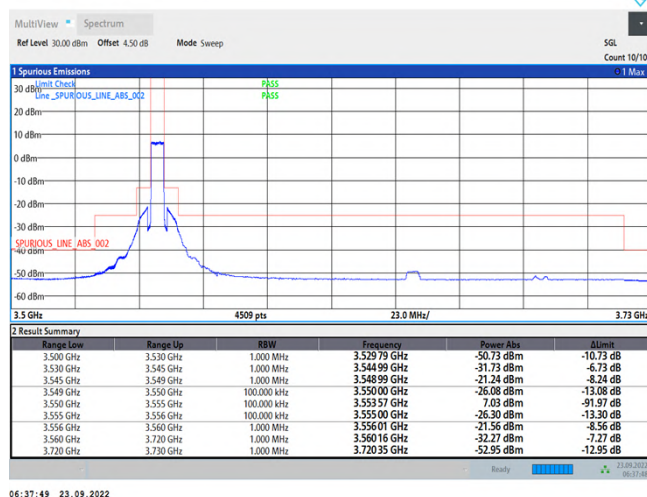
Band48-5MHz-QPSK-55265-25RB#0
