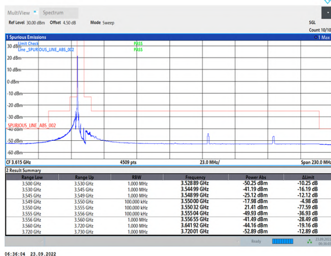
Band48-5MHz-QPSK-55265-25RB#0
