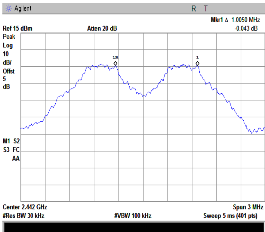
1M-Channel Separation-2441
