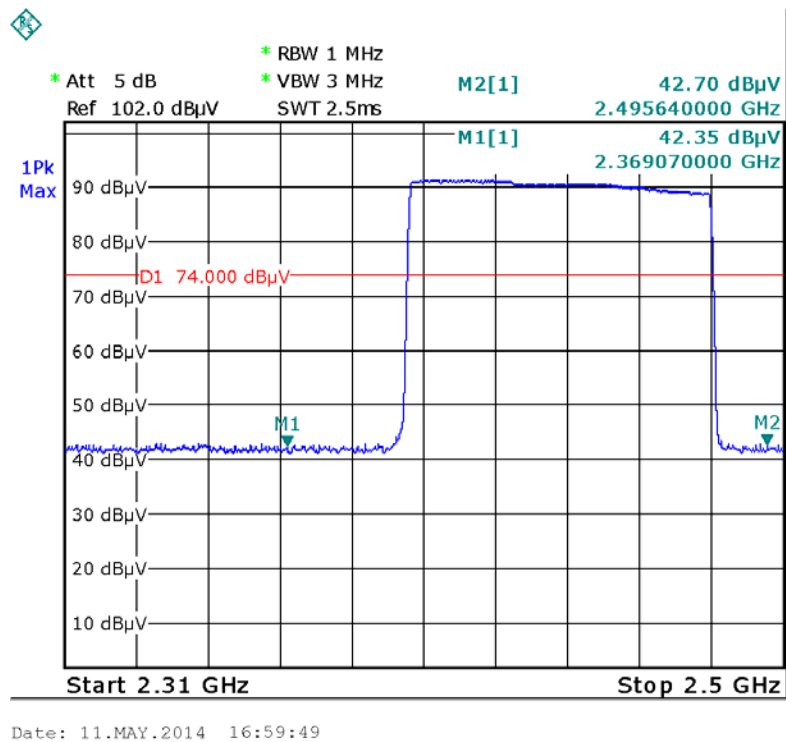
1M-HOPPING-PK
