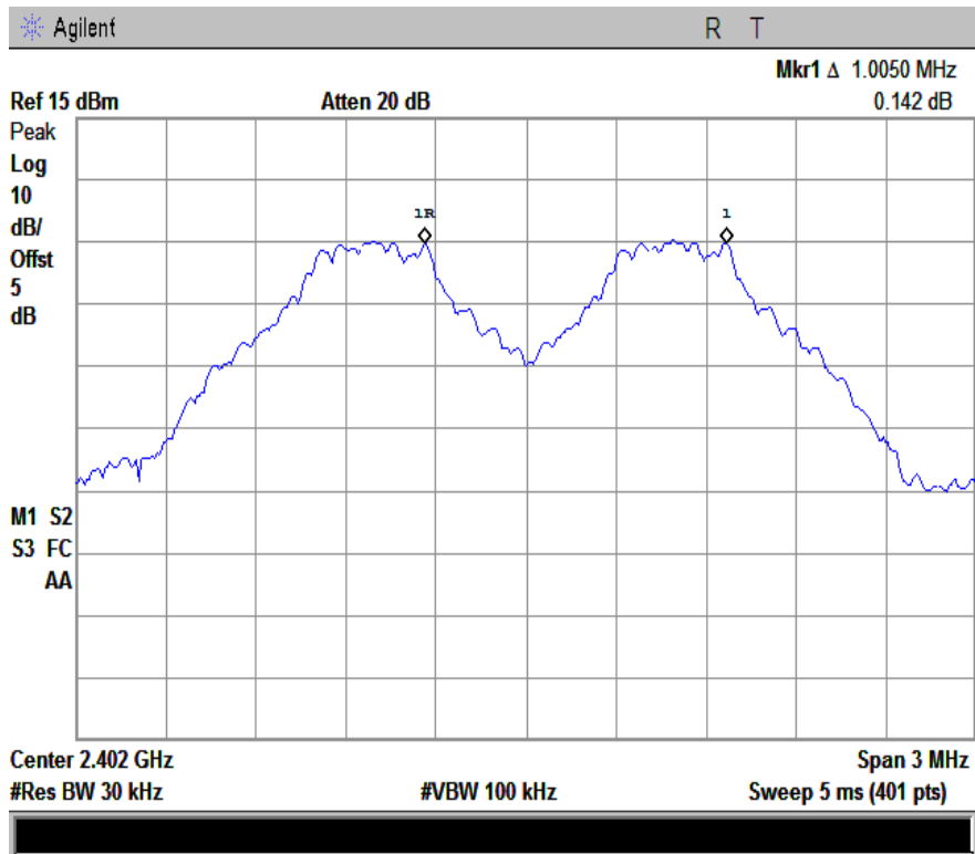
1M-Channel Separation-2402
