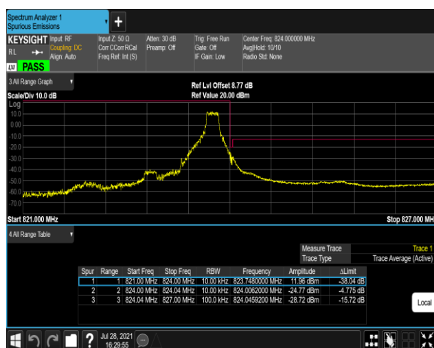
Band26-1.4MHz-QPSK-26783-1RB#5
