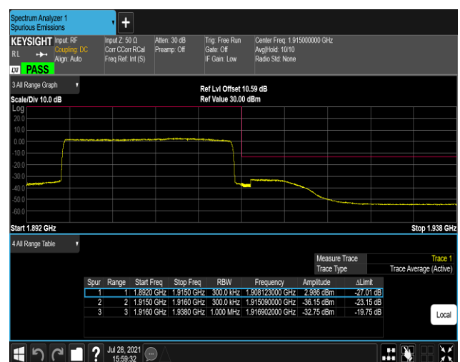
Band25-20MHz-16QAM-26590-100RB#0
