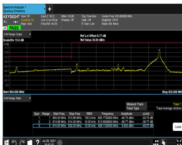
Band26-15MHz-16QAM-26765-1RB#74
