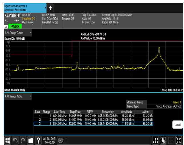
Band26-15MHz-QPSK-26865-1RB#0
