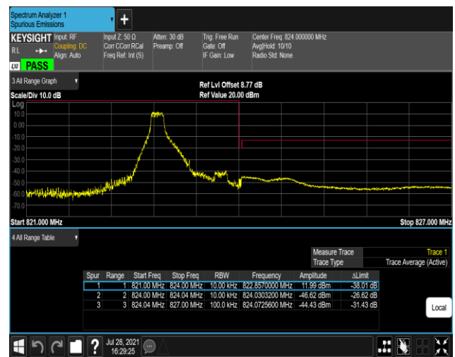
Band26-1.4MHz-QPSK-26783-6RB#0
