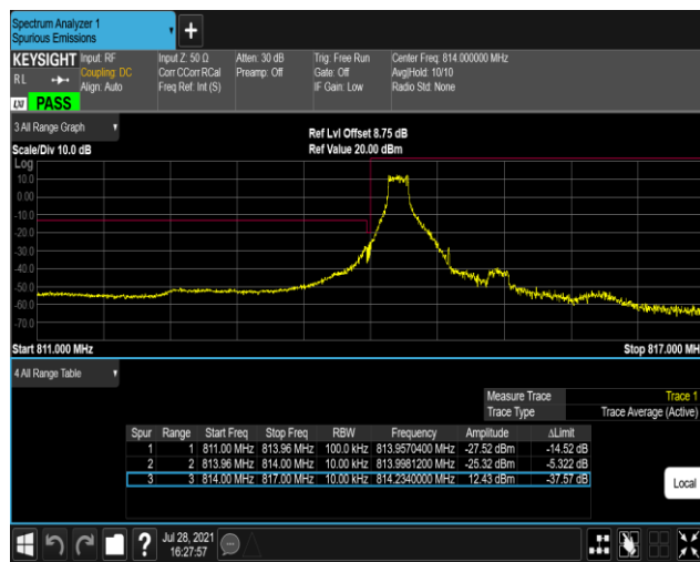
Band26-1.4MHz-QPSK-26697-6RB#0
