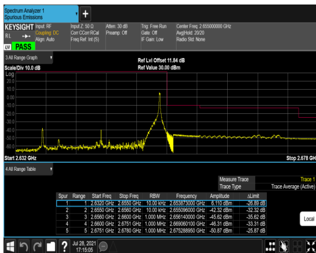
Band41-20MHz-16QAM-41140-1RB#99
