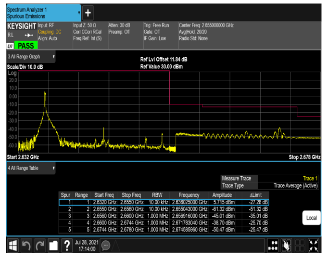
Band41-20MHz-QPSK-41140-100RB#0
