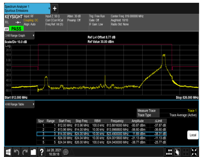
Band26-10MHz-16QAM-26740-1RB#0
