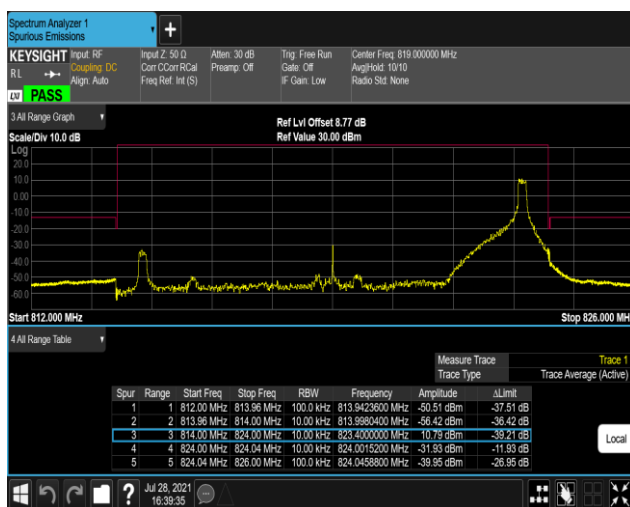
Band26-10MHz-16QAM-26740-1RB#49
