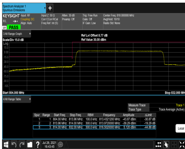
Band26-15MHz-QPSK-26865-1RB#74
