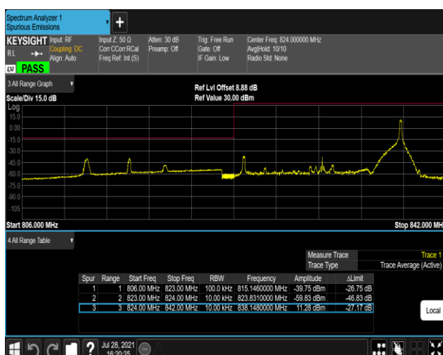
Band26-15MHz-QPSK-26865-1RB#74
