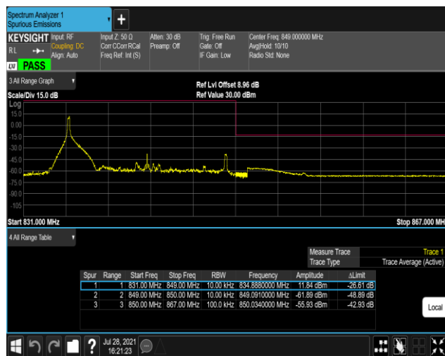
Band26-15MHz-QPSK-26965-75RB#0
