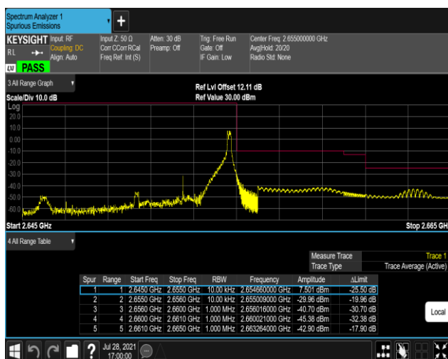
Band41-5MHz-QPSK-41215-1RB#24
