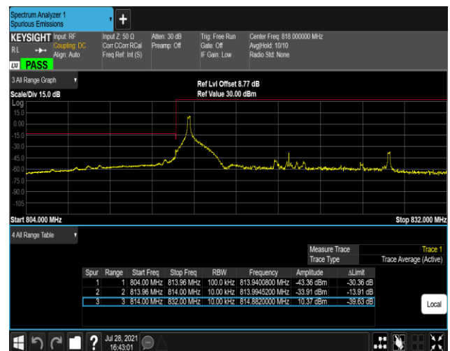
Band26-15MHz-16QAM-26765-75RB#0
