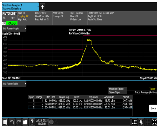
Band26-1.4MHz-QPSK-26797-6RB#0
