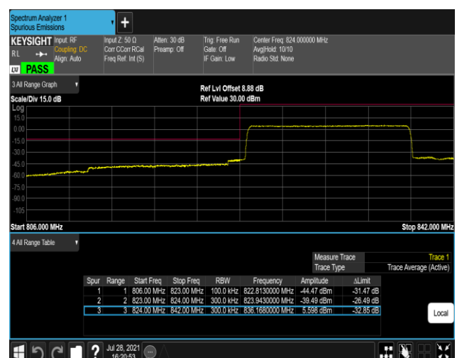
Band26-15MHz-QPSK-26865-75RB#0
