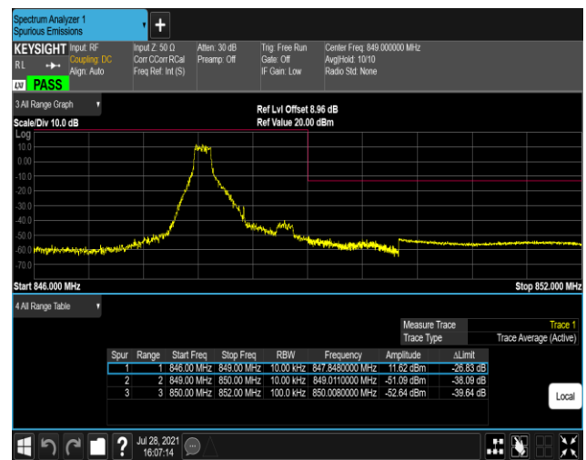
Band26-1.4MHz-16QAM-27033-6RB#0
