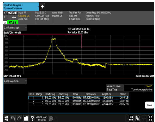
Band26-1.4MHz-QPSK-27033-6RB#0
