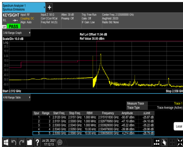
Band41-20MHz-16QAM-40140-100RB#0
