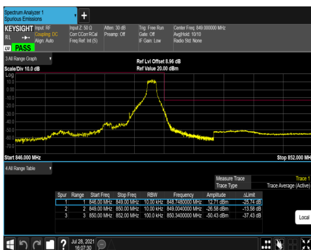
Band26-1.4MHz-QPSK-27033-1RB#5
