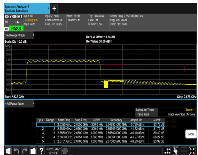
Band41-20MHz-16QAM-41140-100RB#0
