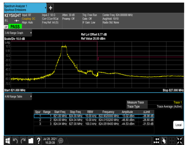
Band26-1.4MHz-16QAM-26783-6RB#0
