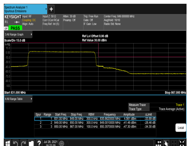
Band26-15MHz-16QAM-26965-75RB#0
