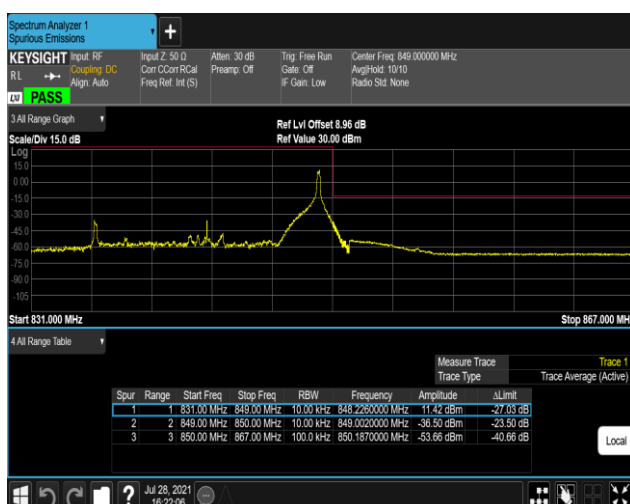
Band26-15MHz-16QAM-26965-1RB#74
