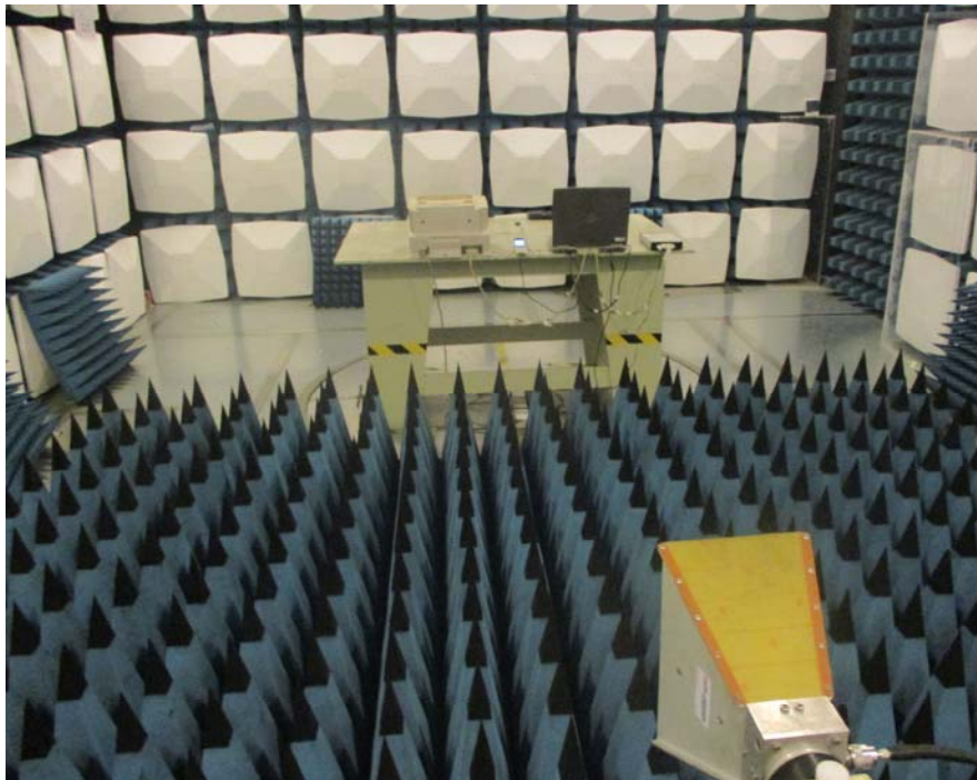
Radiated Emission Rear View (Above 1GHz)
