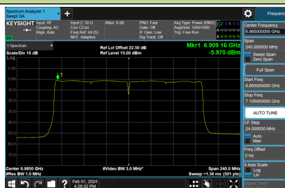
Channel 207 (6985MHz)
