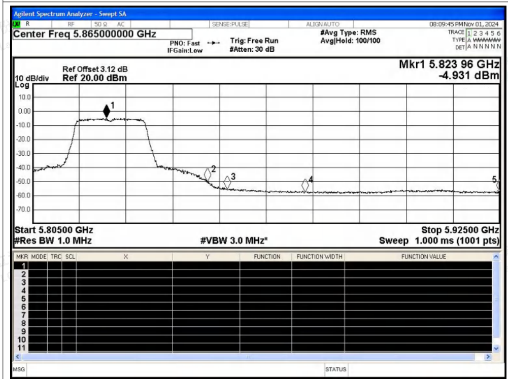
Restrict Band NVNT ac20 5825MHz Ant0 Average
