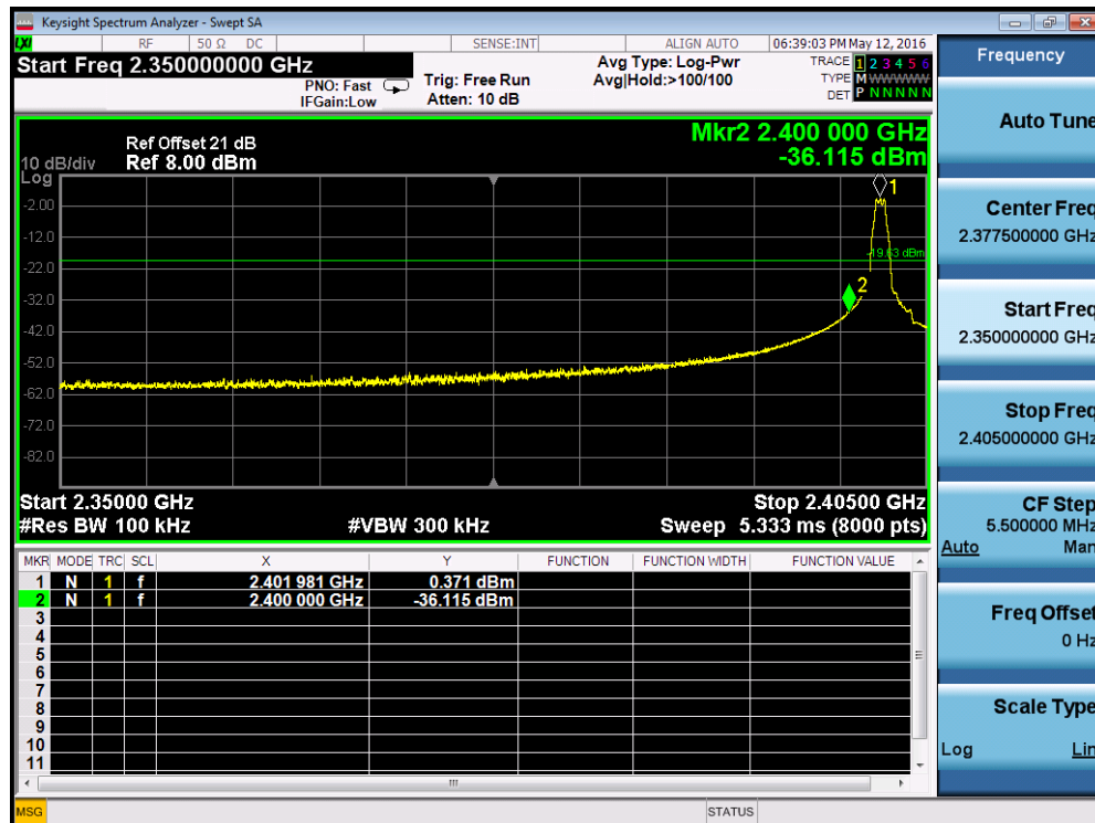
Mode 1 CH00(2402MHz)
