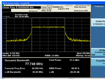
CH151 26 dB Bandwidth
