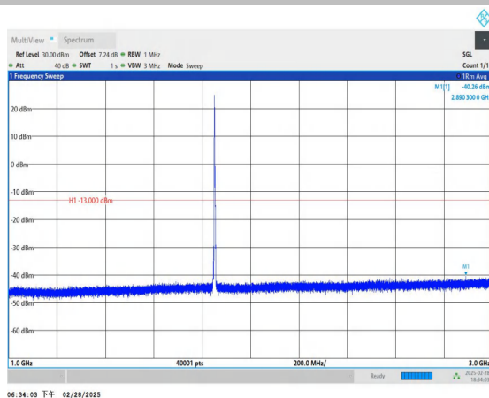
Band2_3MHz_QPSK_18615_1RB#0_1000~3000_1000~3000
