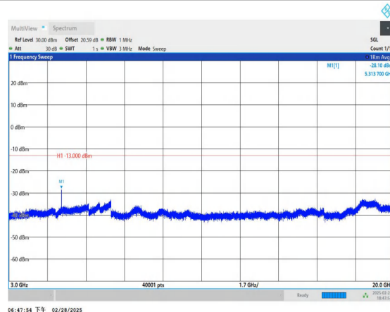
Band2_5MHz_QPSK_18900_1RB#0_3000~20000_3000~20000
