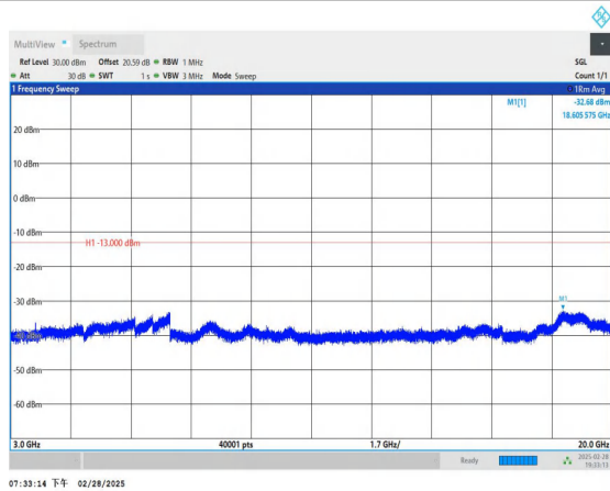
Band2_15MHz_QPSK_18675_1RB#0_3000~20000_3000~2000
