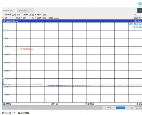
Band2_15MHz_QPSK_18675_1RB#0_30~1000_30~1000
