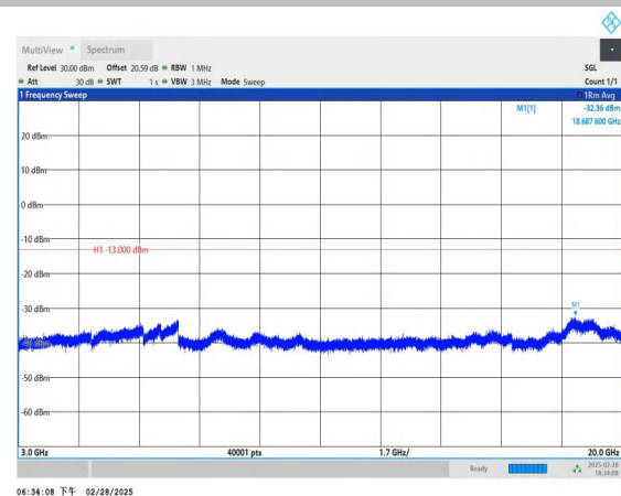
Band2_3MHz_QPSK_18615_1RB#0_3000~20000_3000~20000
