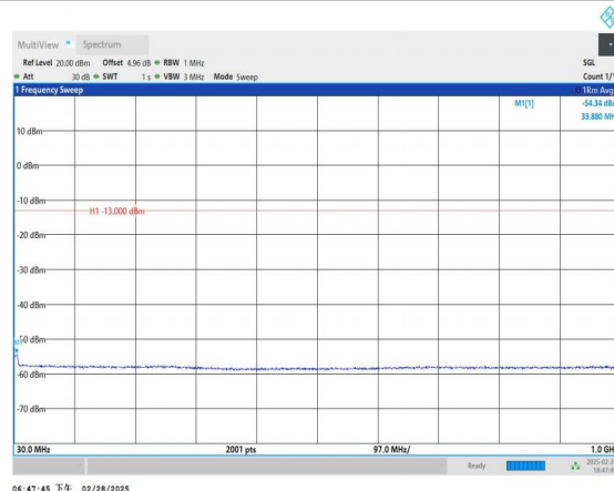
Band2_5MHz_QPSK_18900_1RB#0_30~1000_30~1000
