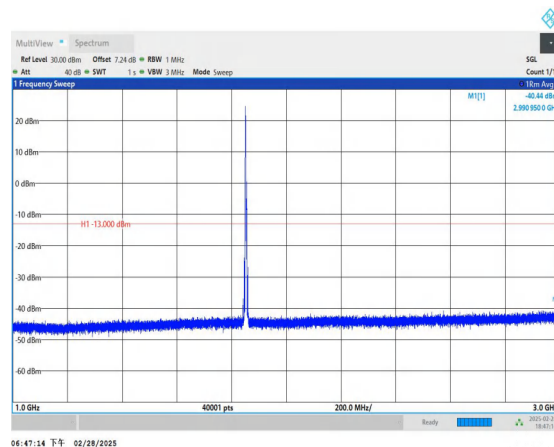
Band2_5MHz_QPSK_18625_1RB#0_1000~3000_1000~3000
