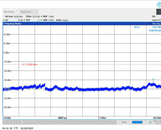
Band2_1.4MHz_QPSK_19193_1RB#0_3000~20000_3000~2000
