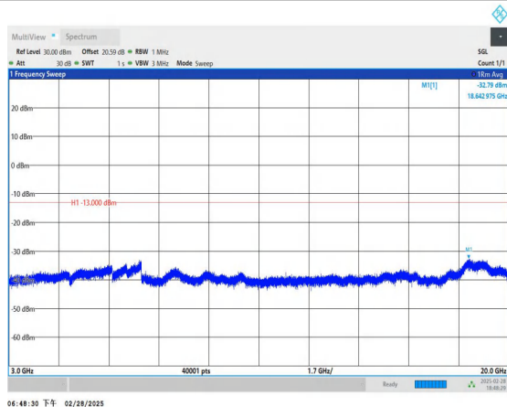
Band2_5MHz_QPSK_19175_1RB#0_3000~20000_3000~20000
