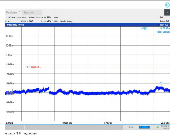
Band2_1.4MHz_QPSK_18900_1RB#0_3000~20000_3000~2000
