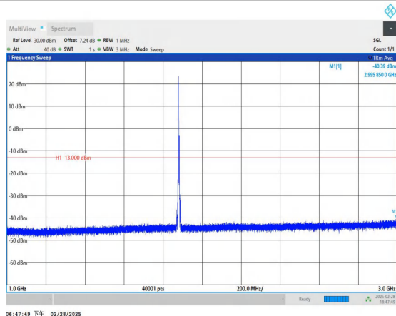
Band2_5MHz_QPSK_18900_1RB#0_1000~3000_1000~3000
