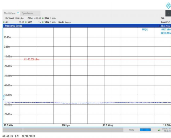
Band2_5MHz_QPSK_19175_1RB#0_30~1000_30~1000
