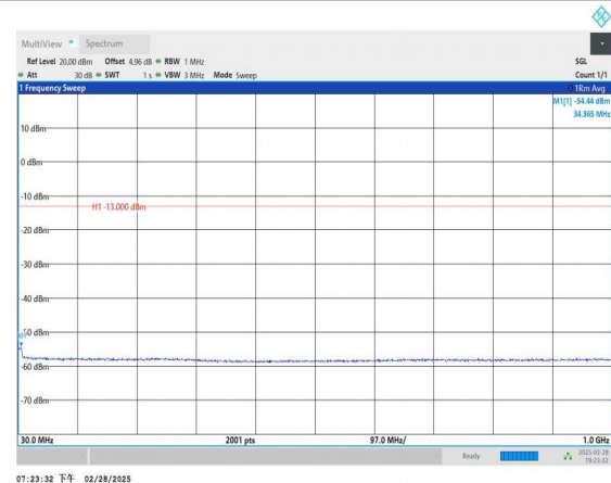
Band2_10MHz_QPSK_18650_1RB#0_30~1000_30~1000
