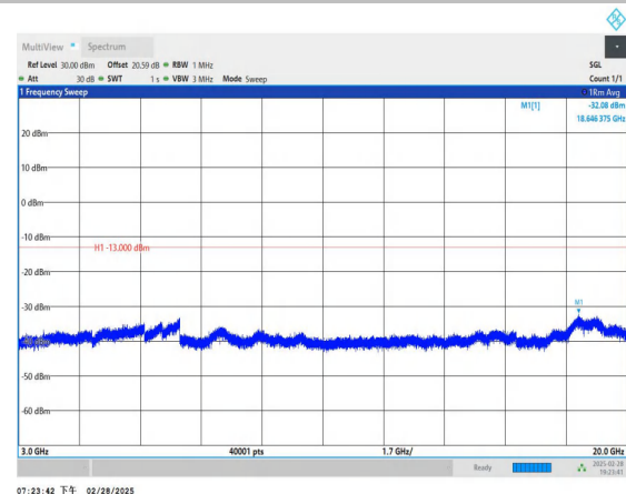
Band2_10MHz_QPSK_18650_1RB#0_3000~20000_3000~20000
