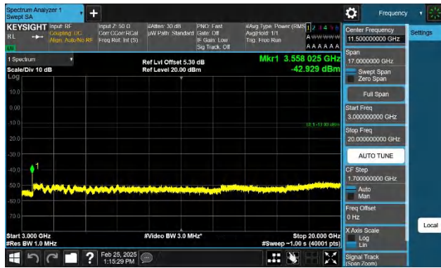
Band66-1.4MHz-QPSK-132665-1RB#0-3000~20000-PASS
