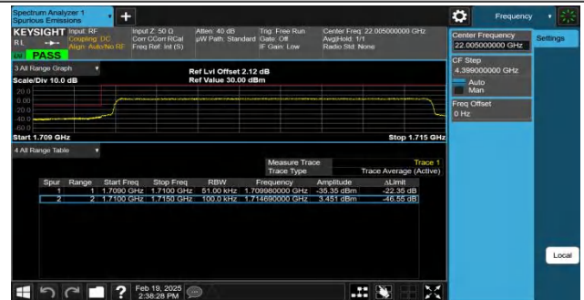
Band66-5MHz-QPSK-131997-25RB#0-PASS
