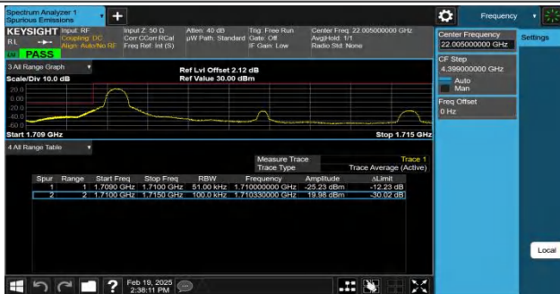
Band66-5MHz-QPSK-131997-1RB#0-PASS
