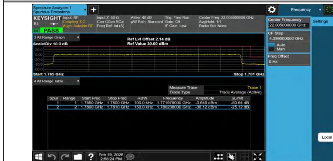
Band66-15MHz-QPSK-132597-75RB#0-PASS
