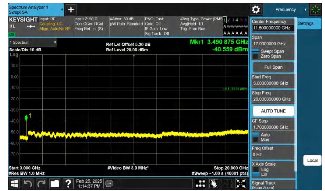
Band66-1.4MHz-QPSK-132322-1RB#5-3000~20000-PASS
