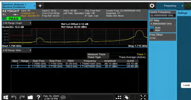
Band66-5MHz-QPSK-131997-1RB#24-PASS
