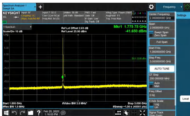
Band66-1.4MHz-QPSK-132665-1RB#5-1000~3000-PASS
