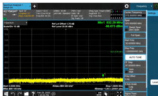
Band66-3MHz-QPSK-132657-1RB#14-30~1000-PASS
