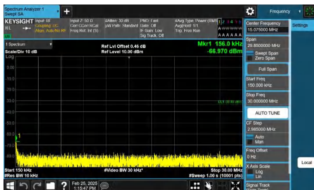
Band66-1.4MHz-QPSK-132665-1RB#5-0.15~30-PASS
