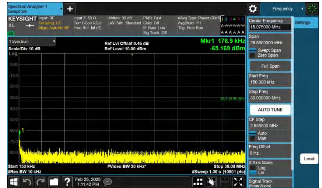
Band66-1.4MHz-QPSK-131979-1RB#0-0.15~30-PASS
