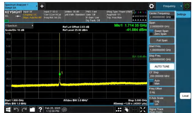
Band66-1.4MHz-QPSK-131979-1RB#0-1000~3000-PASS
