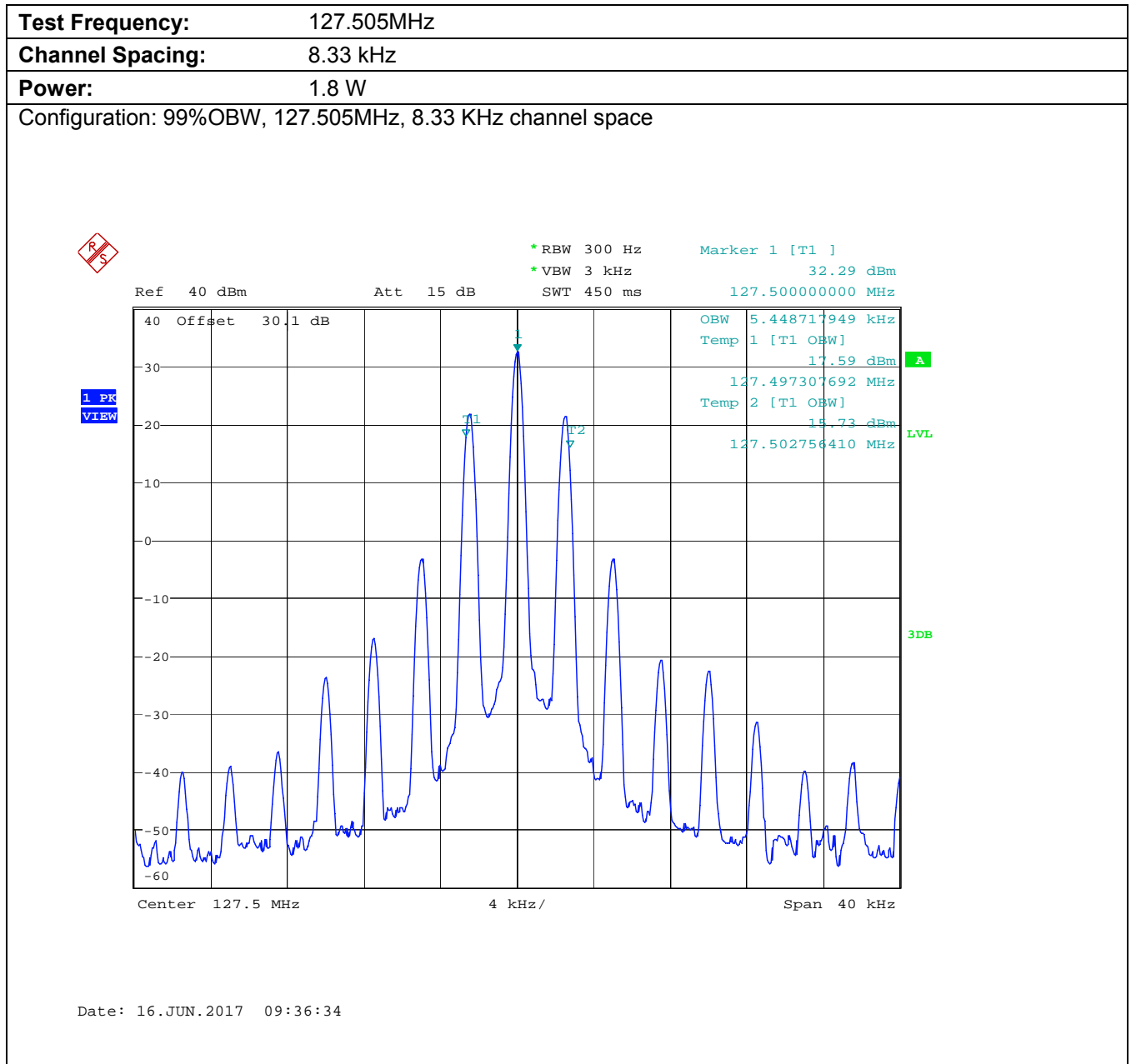
Plot 5.6.4.1.2. 99% Occupied Bandwidth
