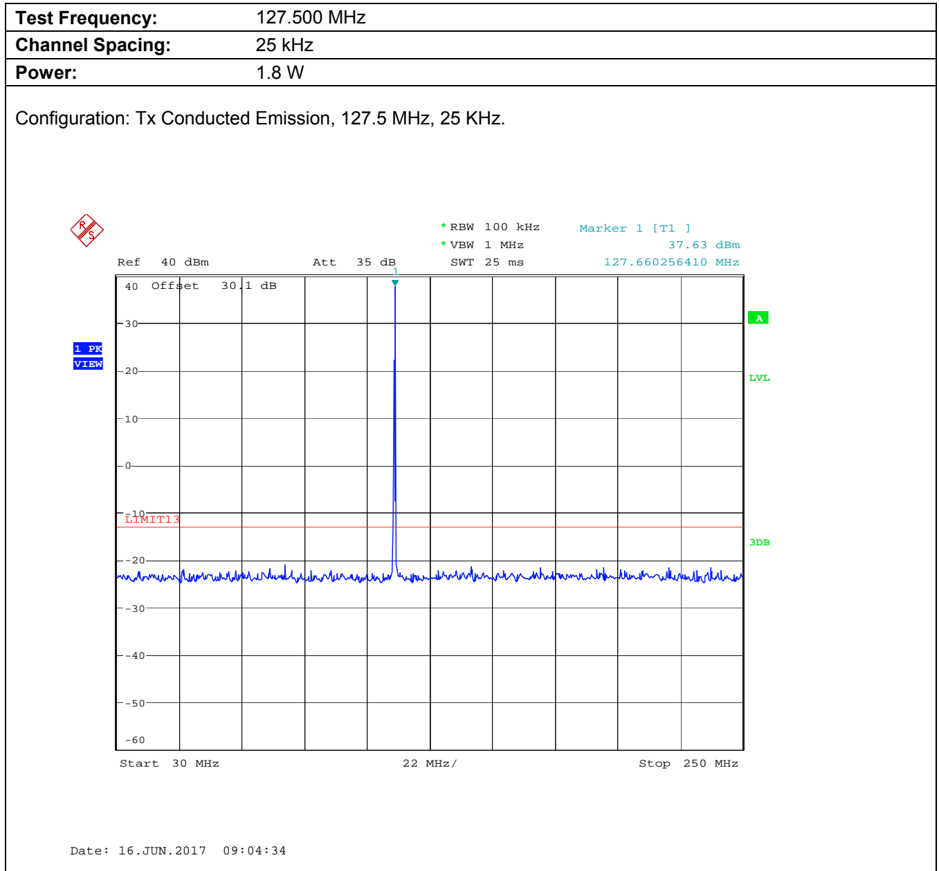
Plot 5.10.4.2. Conducted Transmitter Spurious Emissions
