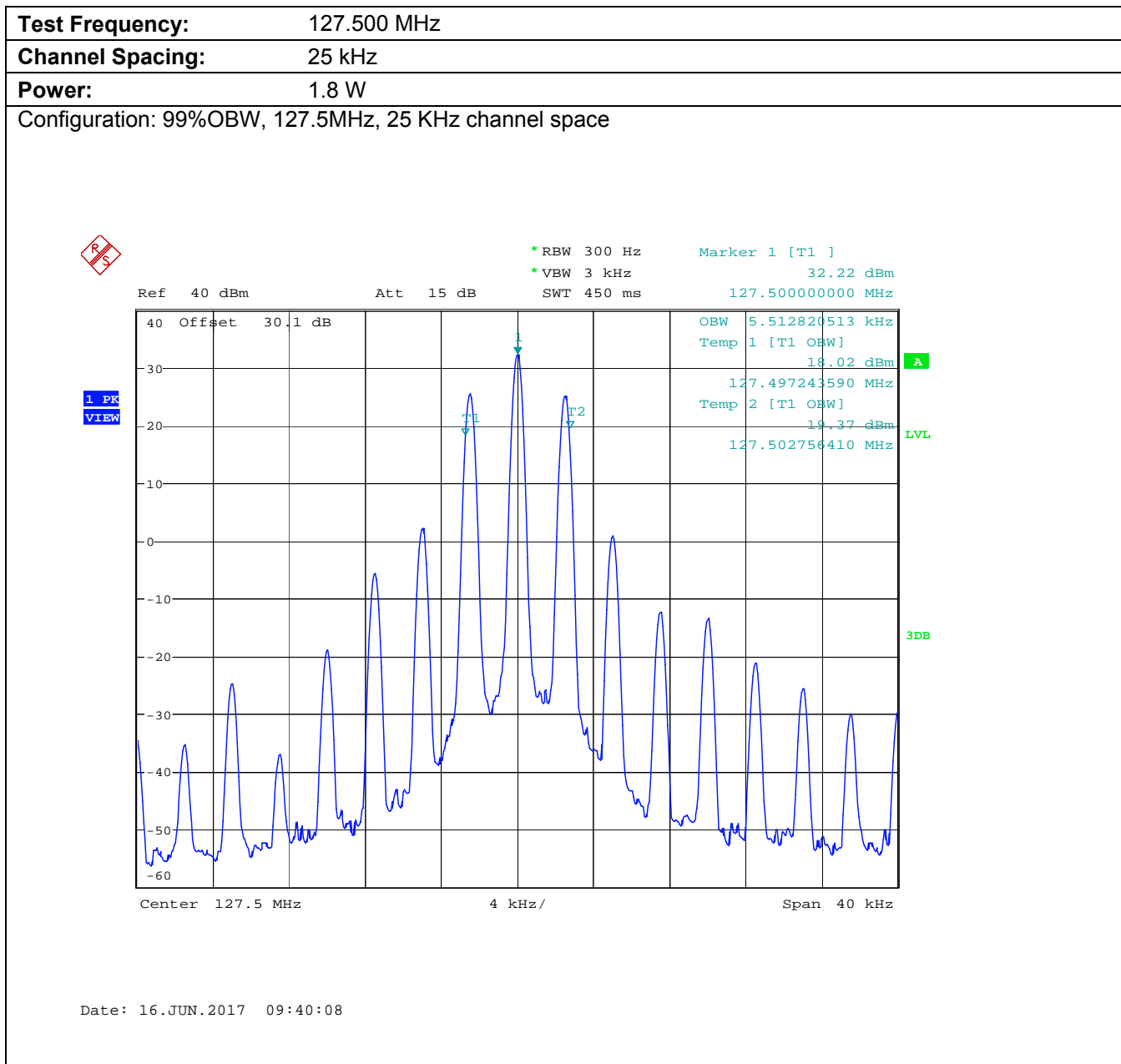
Plot 5.6.4.1.5. 99% Occupied Bandwidth
