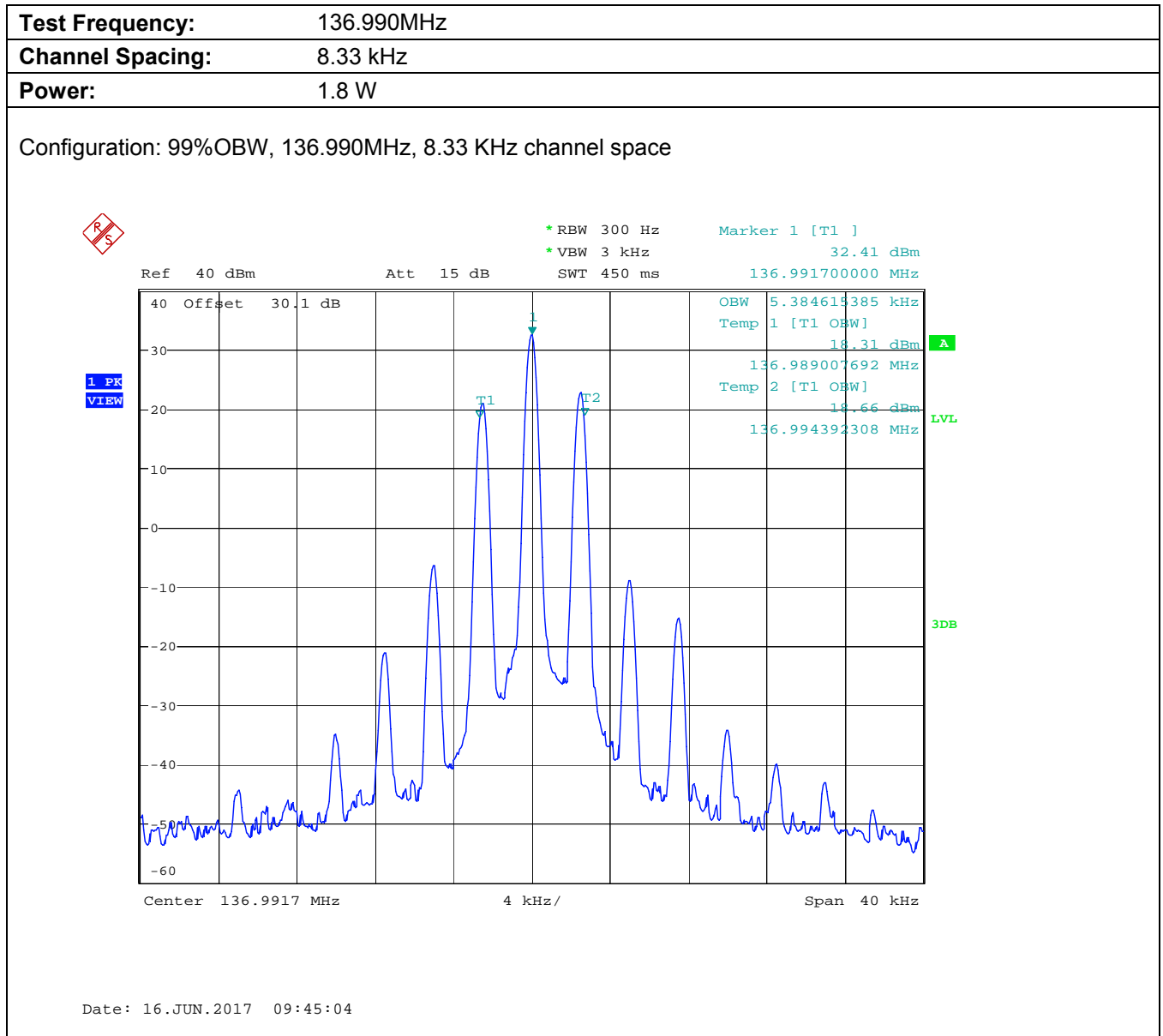
Plot 5.6.4.1.3. 99% Occupied Bandwidth
