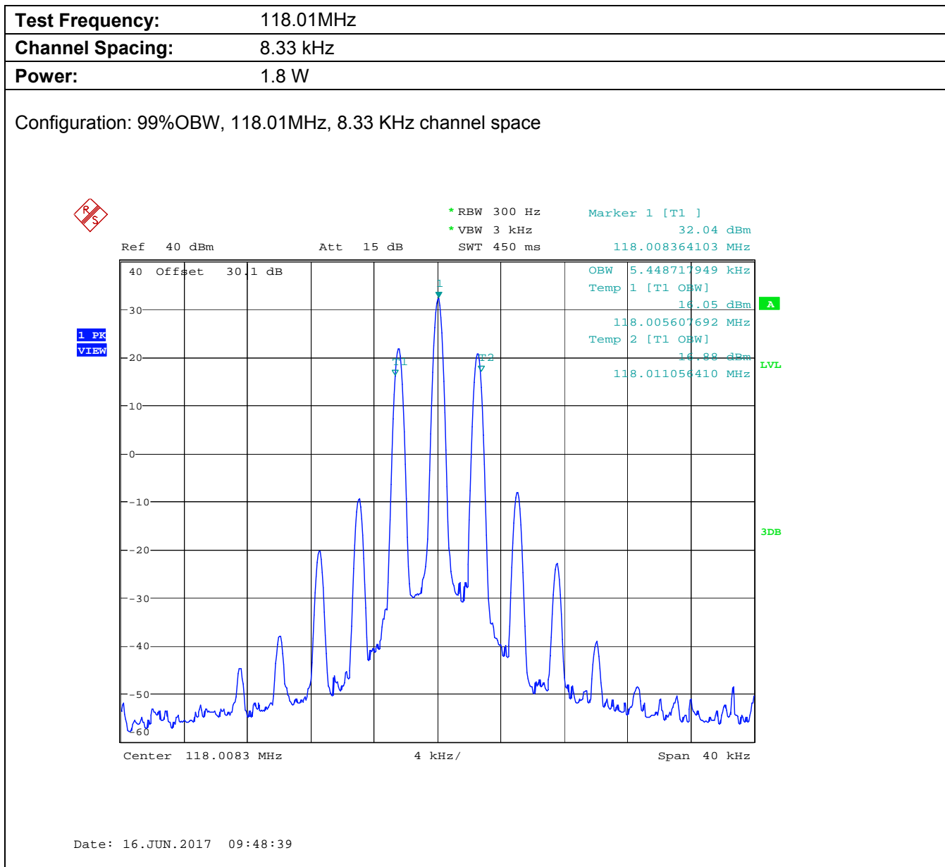
Plot 5.6.4.1.1. 99% Occupied Bandwidth
