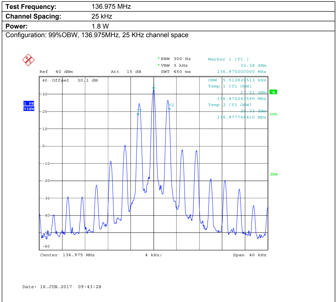
Plot 5.6.4.1.6. 99% Occupied Bandwidth
