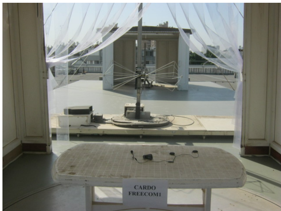
Note – Preliminary radiated emission testing set-up. All emissions were at least 20dB below the limit
